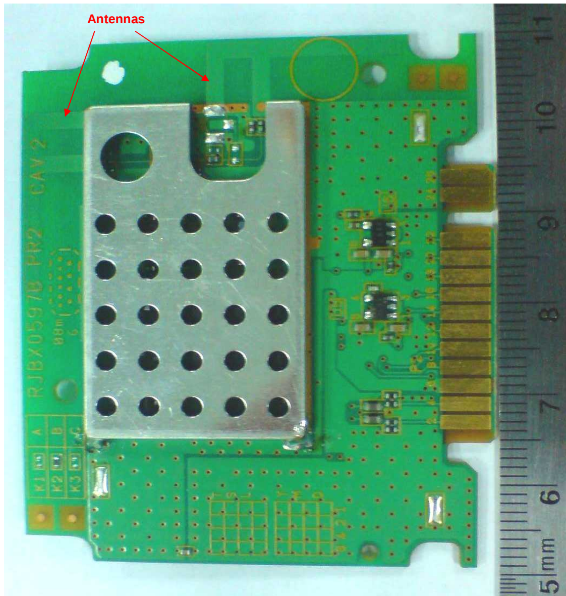
Front View
