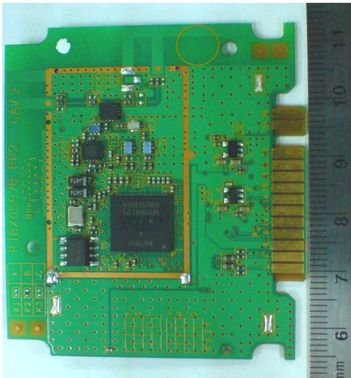
Shield Removed View
