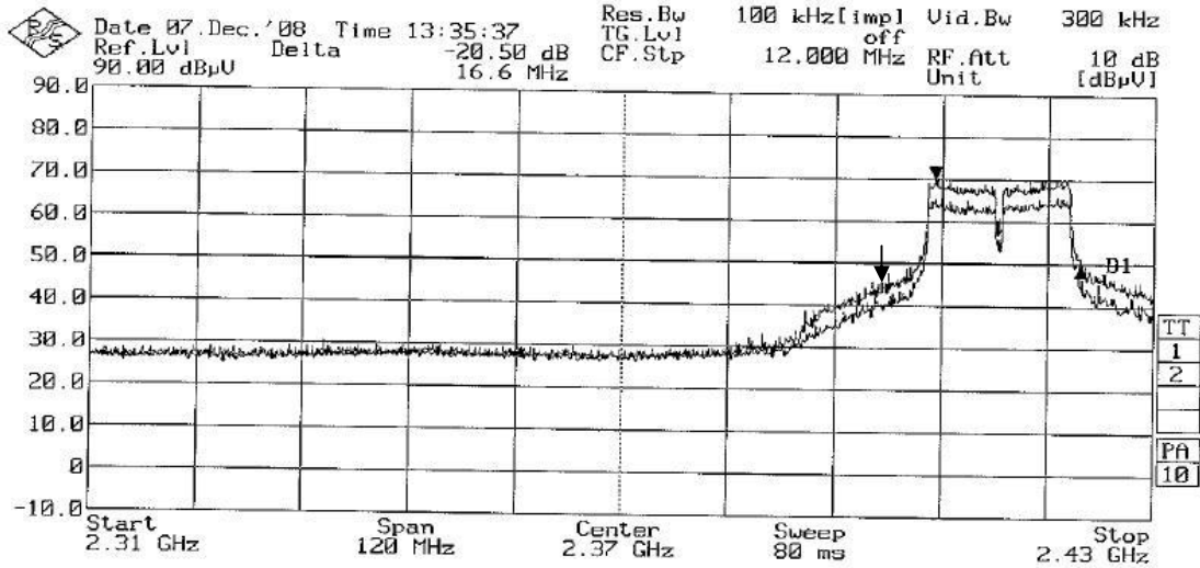
Plot 12 – Lower Band Edge at 2.400GHz
