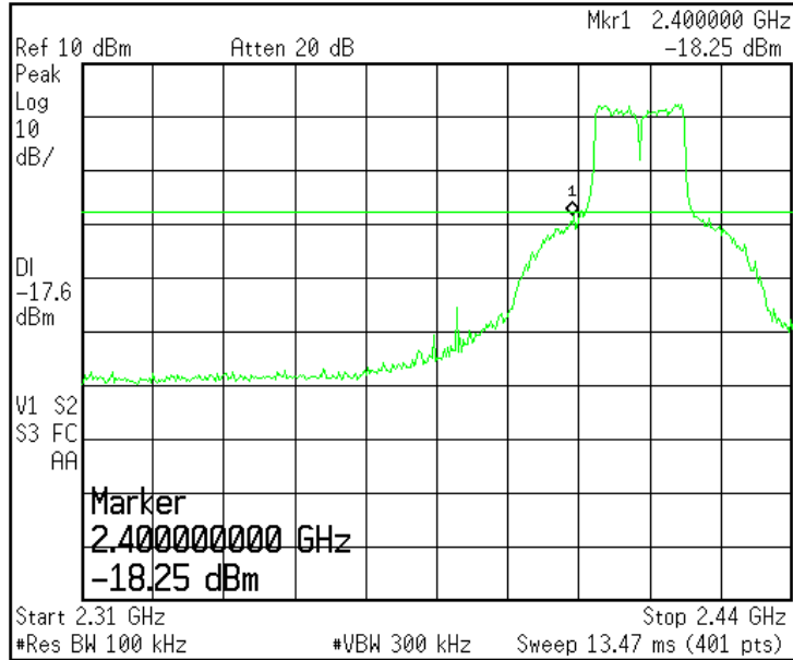
Plot 10 – Lower Band Edge at 2.4000GHz
