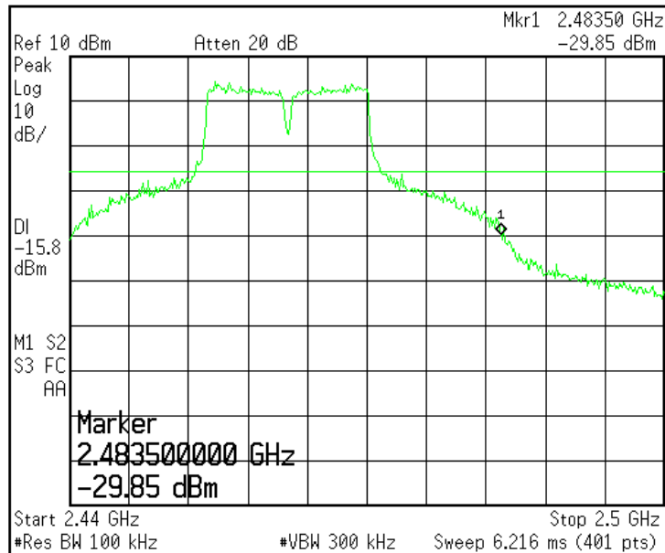
Plot 11 – Upper Band Edge at 2.4620GHz
