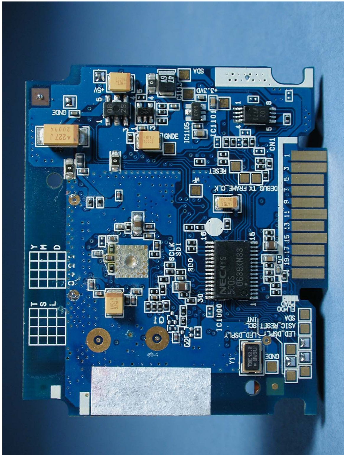
Photograph 2: Rear view SH-FX65-1
