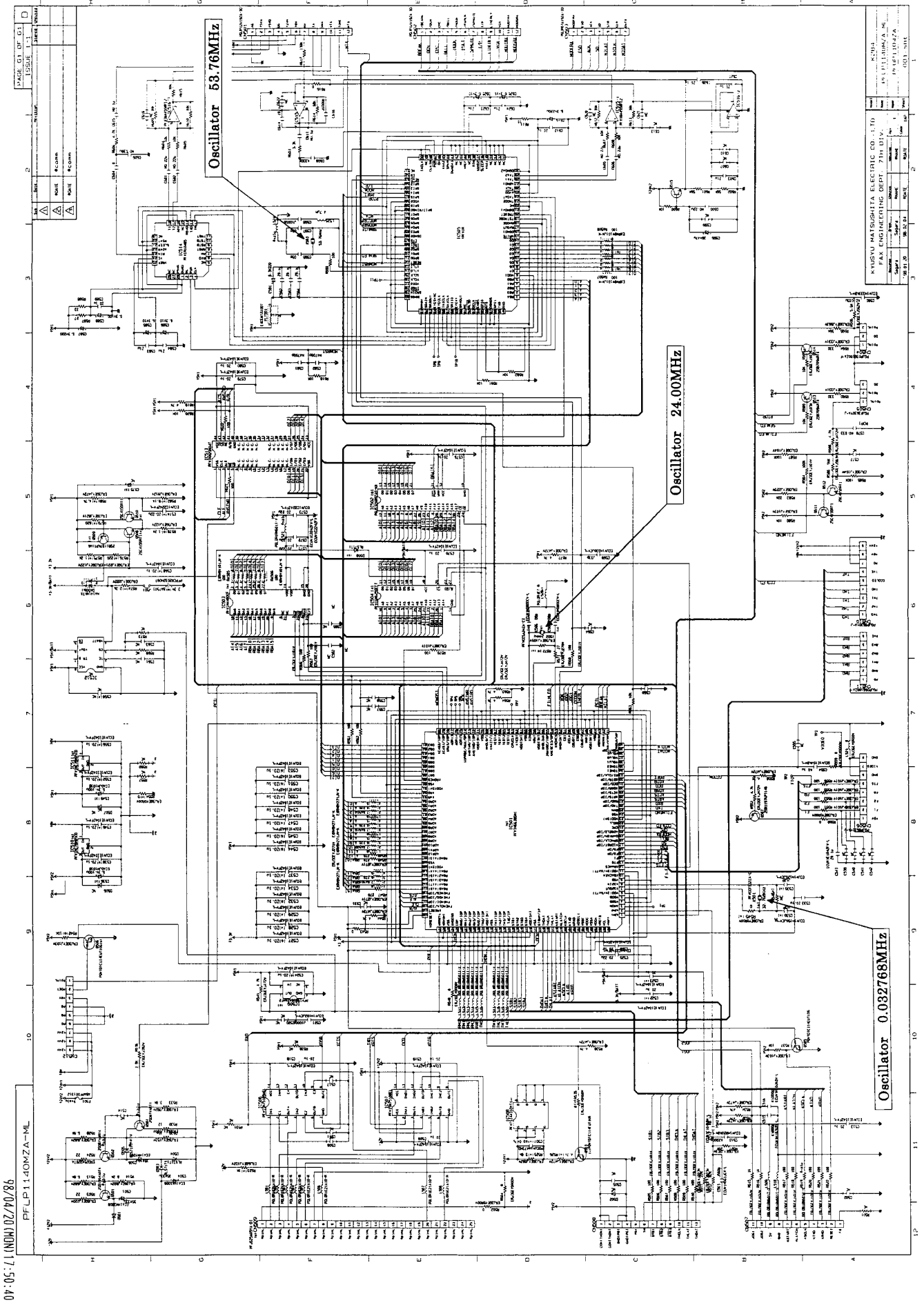
FIG. 3 DIGITAL BOARD
