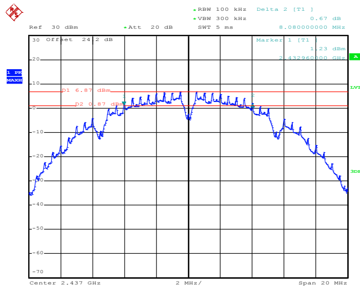
6 dB Bandwidth Plot on Channel 06
