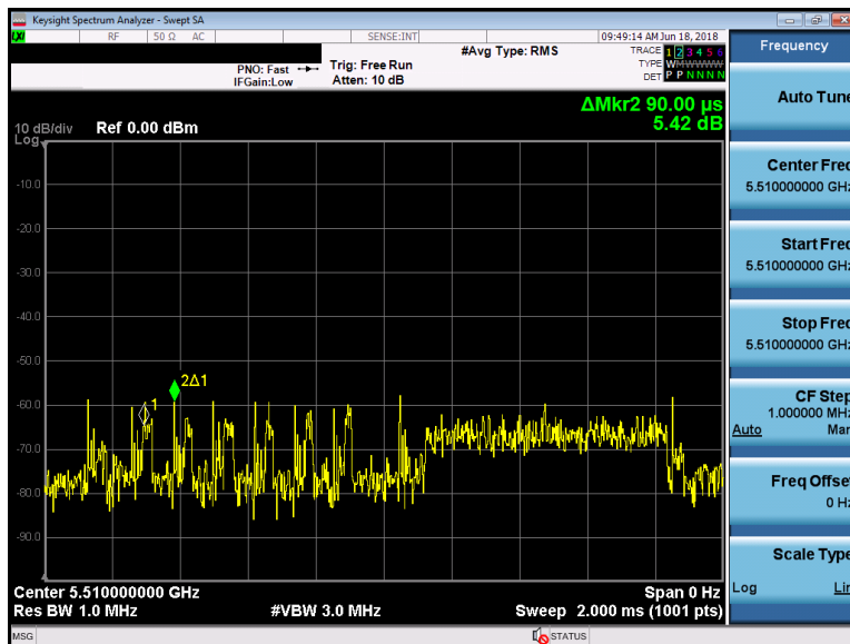
Figure 5-4. Band 2C Period
