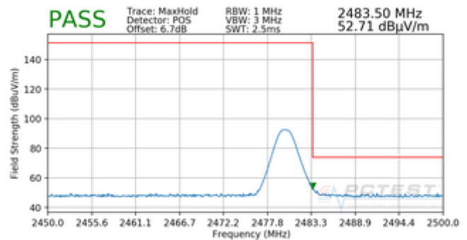
Plot 7-48. Radiated Restricted Upper Band Edge Measurement (Peak - L-Battery)
