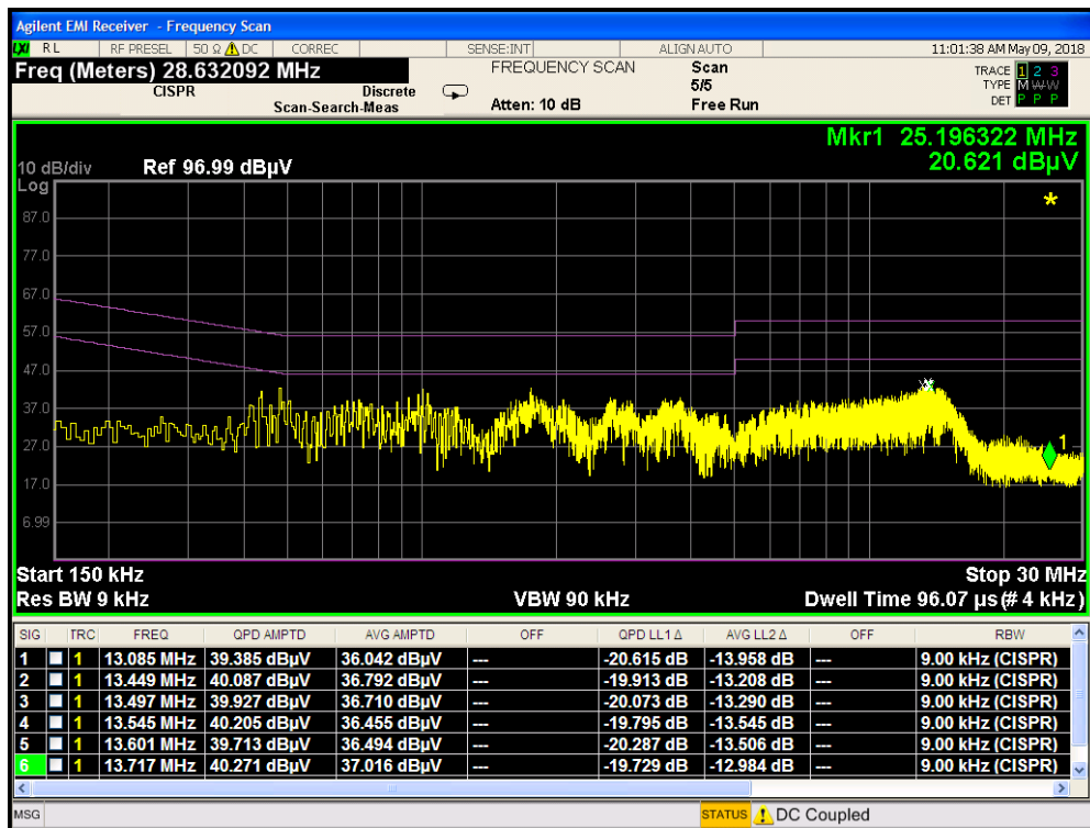
Plot 7-122. Line Conducted Plot with 802.11a UNII Band 3 (L1)
