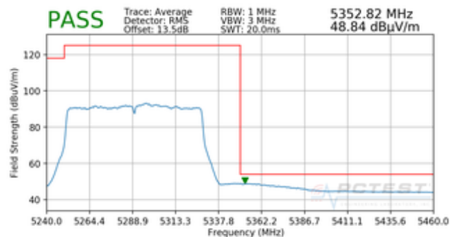
Plot 7-113. Radiated Band Edge Plot (Average – L-Battery)
