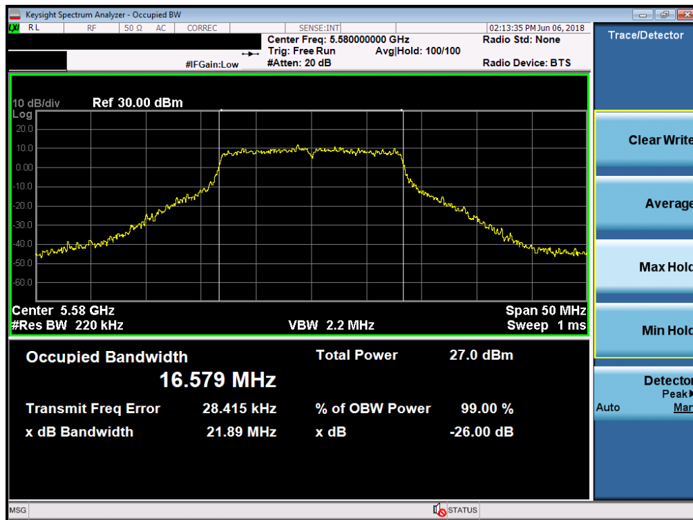
Plot 7-20. 26dB Bandwidth Plot (802.11a (UNII Band 2C) – Ch. 116120)
