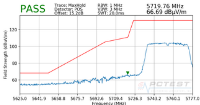
Plot 7-101. Radiated Lower Band Edge Plot (Peak – UNII Band 3)
