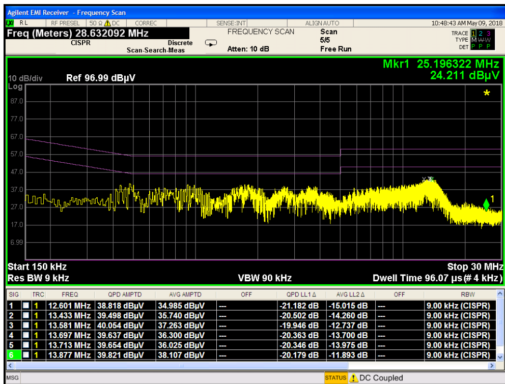
Plot 7-120. Line Conducted Plot with 802.11a UNII Band 2C (L1)
