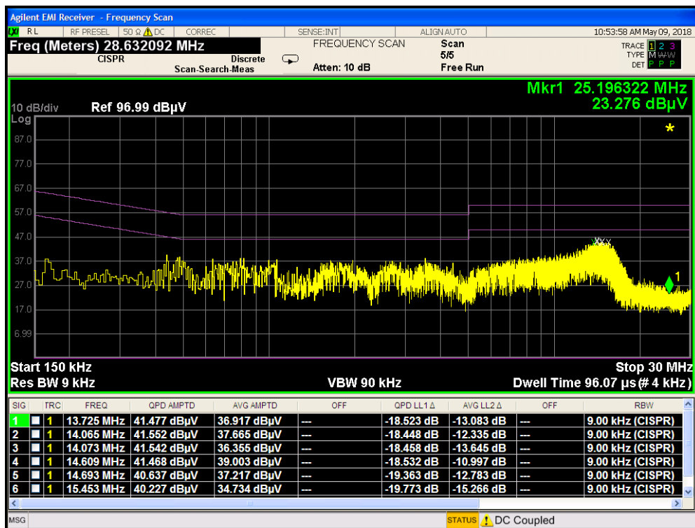
Plot 7-121. Line Conducted Plot with 802.11a UNII Band 2C (N)
