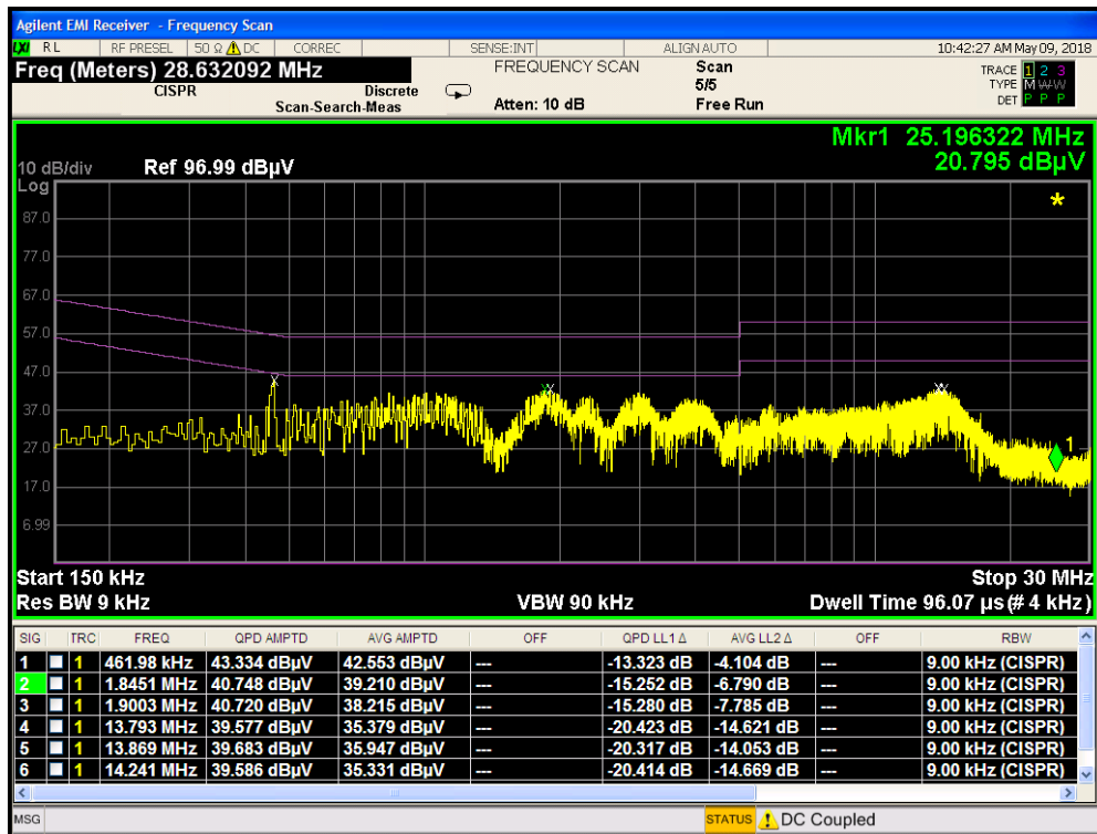
Plot 7-118. Line Conducted Plot with 802.11a UNII Band 2A (L1)
