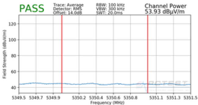
Plot 7-96. Radiated Upper Band Edge Plot (Average – UNII Band 2A)
