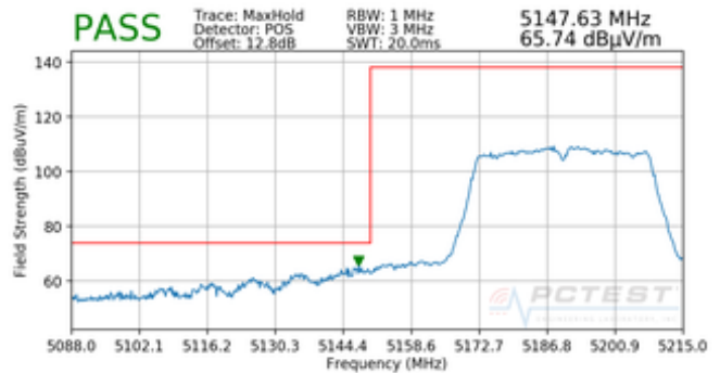
Plot 7-95. Radiated Lower Band Edge Plot (Peak – UNII Band 1)
