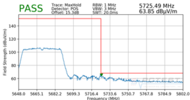
Plot 7-100. Radiated Upper Band Edge Plot (Peak – UNII Band 2C)
