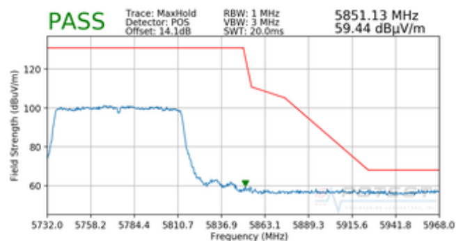
Plot 7-112. Radiated Upper Band Edge Plot (Peak – UNII Band 3)
