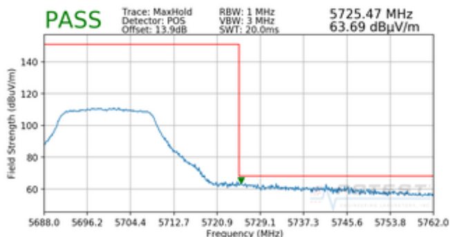
Plot 7-89. Radiated Upper Band Edge Plot (Peak – UNII Band 2C)
