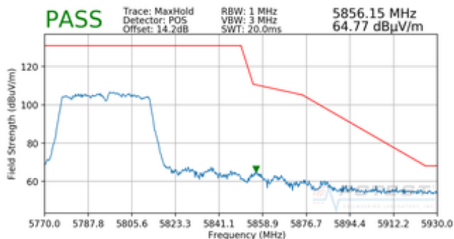
Plot 7-102. Radiated Upper Band Edge Plot (Peak – UNII Band 3)
