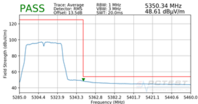
Plot 7-103. Radiated Band Edge Plot (Average – L-Battery)
