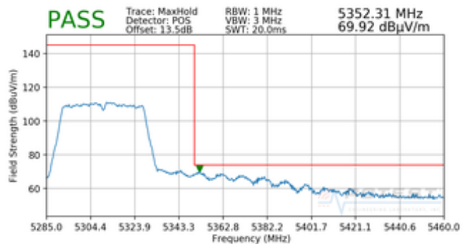
Plot 7-97. Radiated Upper Band Edge Plot (Peak – UNII Band 2A)
