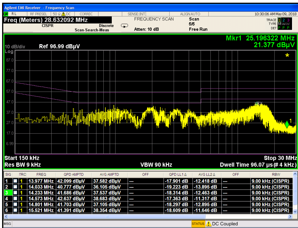
Plot 7-119. Line Conducted Plot with 802.11a UNII Band 2A (N)
