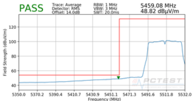
Plot 7-98. Radiated Lower Band Edge Plot (Average – UNII Band 2C)
