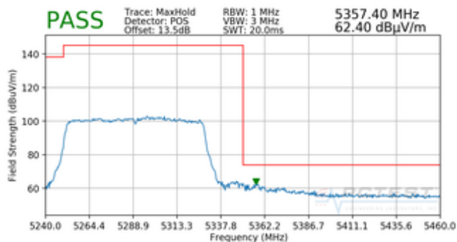
Plot 7-114. Radiated Band Edge Plot (Peak – L-Battery)
