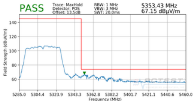
Plot 7-104. Radiated Band Edge Plot (Peak – L-Battery)
