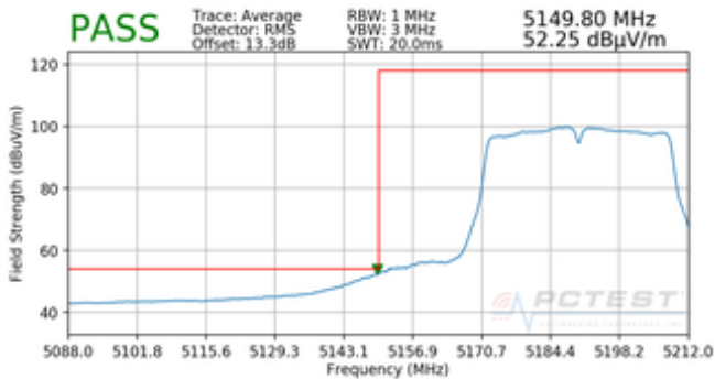
Plot 7-94. Radiated Lower Band Edge Plot (Average – UNII Band 1)
