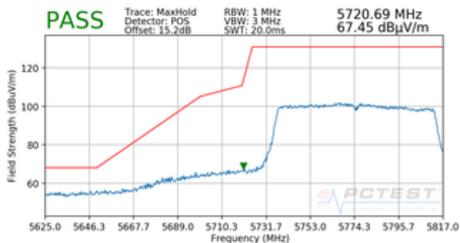
Plot 7-111. Radiated Lower Band Edge Plot (Peak – UNII Band 3)
