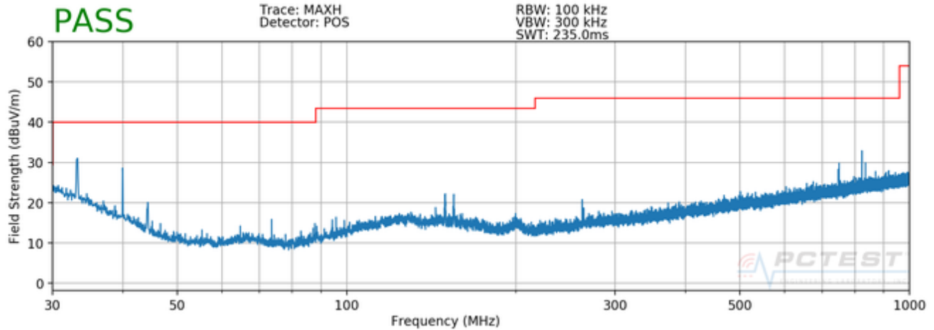
Plot 7-115. Radiated Spurious Plot below 1GHz (802.11a – U3 Ch. 157)
