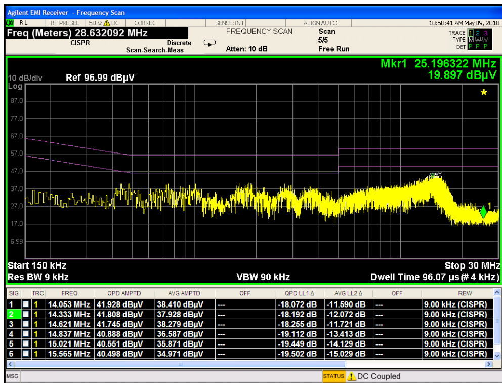
Plot 7-123. Line Conducted Plot with 802.11a UNII Band 3 (N)
