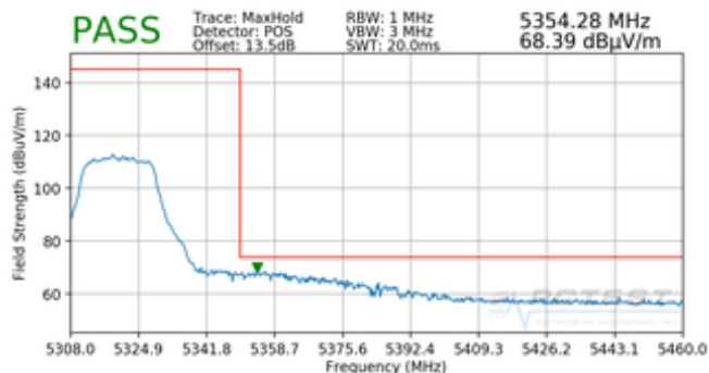
Plot 7-93. Radiated Band Edge Plot (Peak – L-Battery)
