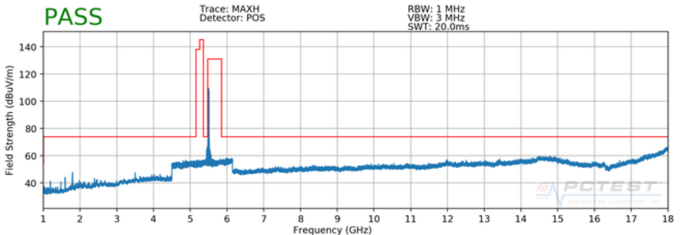
Plot 7-79. Radiated Spurious Plot above 1GHz (802.11a – U2C Ch. 116120)
