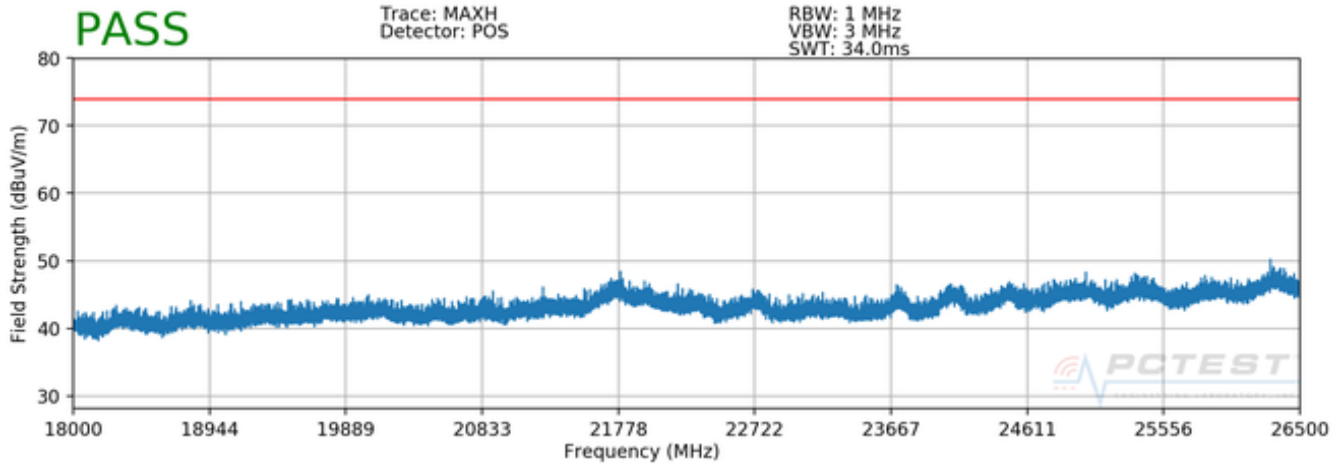
Plot 7-81. Radiated Spurious Plot 18GHz - 26.5GHz (802.11a)
