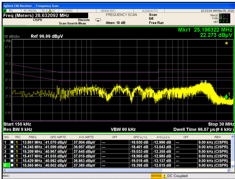
Plot 7-117. Line Conducted Plot with 802.11a UNII Band 1 (N)
