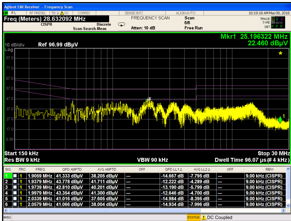
Plot 7-116. Line Conducted Plot with 802.11a UNII Band 1 (L1)
