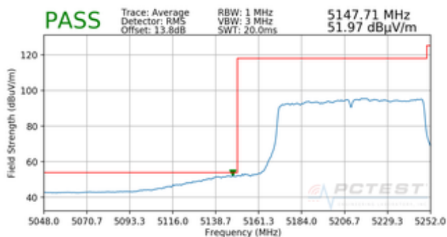
Plot 7-105. Radiated Lower Band Edge Plot (Average – UNII Band 1)
