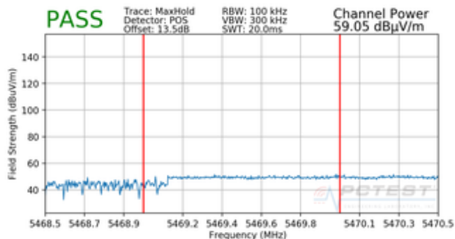
Plot 7-99. Radiated Lower Band Edge Plot (Peak – UNII Band 2C)
