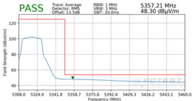
Plot 7-92. Radiated Band Edge Plot (Average – L-Battery)
