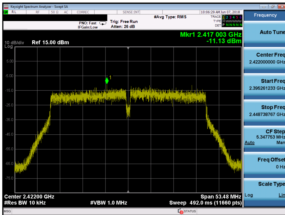
Plot 7-22. Power Spectral Density Plot (40MHz 802.11n (2.4GHz) – Ch. 3)
