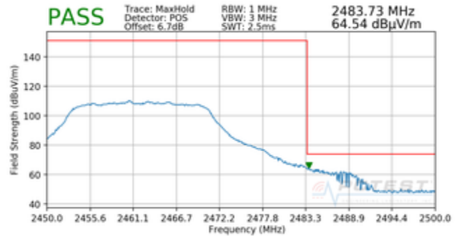
Plot 7-56. Radiated Restricted Upper Band Edge Measurement (Peak – L-Battery)
