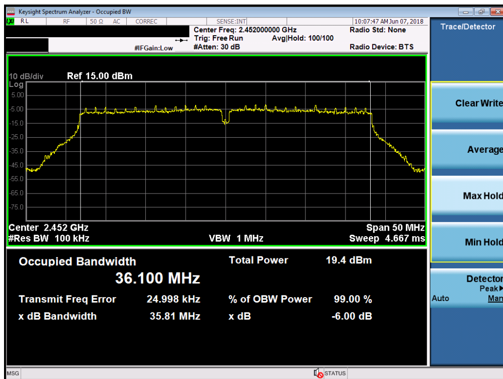
Plot 7-12. 6dB Bandwidth Plot (40MHz 802.11n (2.4GHz) – Ch. 9)
