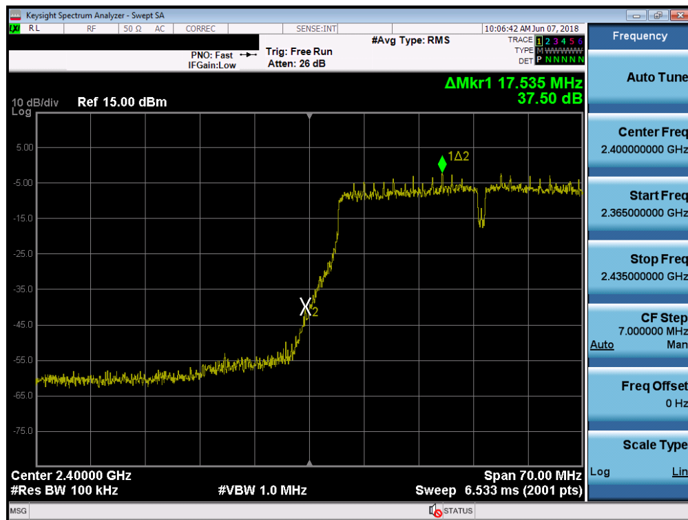
Plot 7-31. Band Edge Plot (40MHz 802.11n (2.4GHz) – Ch. 3)
