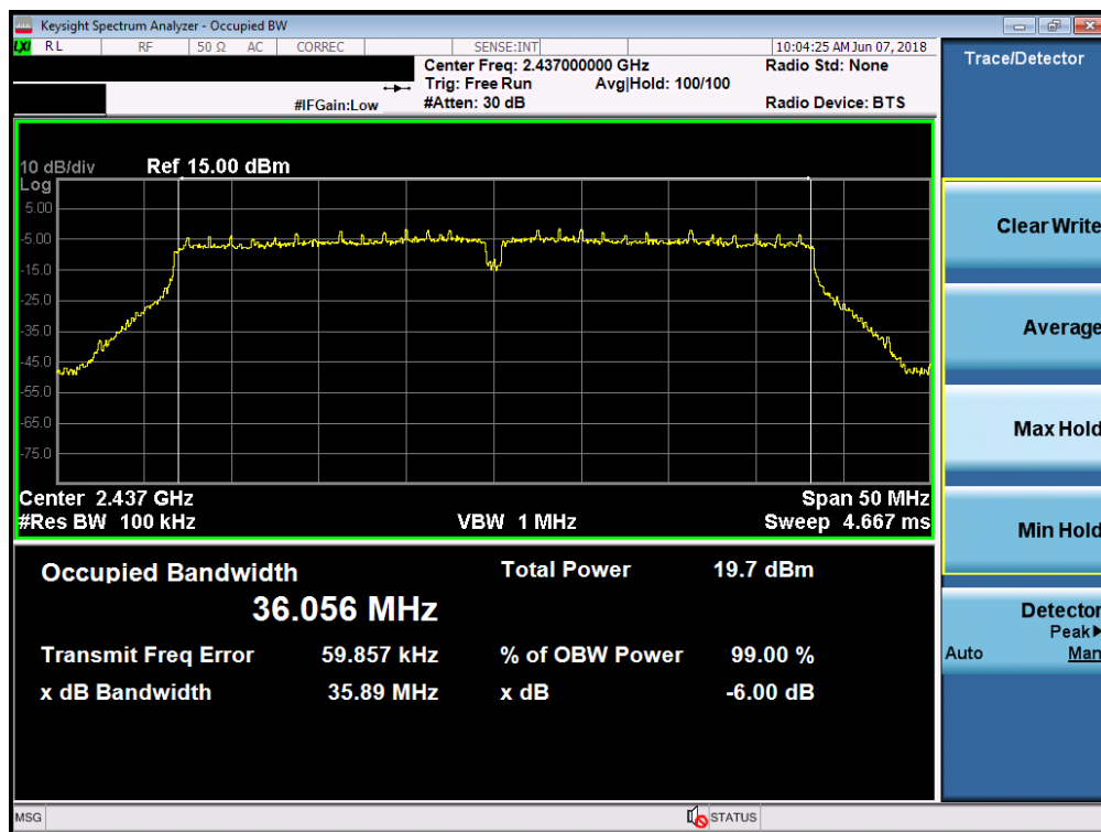
Plot 7-11. 6dB Bandwidth Plot (40MHz 802.11n (2.4GHz) – Ch. 6)
