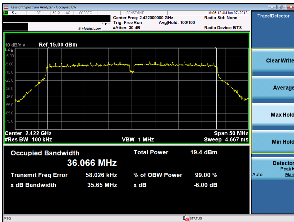
Plot 7-10. 6dB Bandwidth Plot (40MHz 802.11n (2.4GHz) – Ch. 3)
