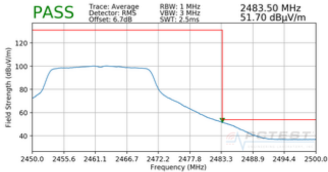
Plot 7-55. Radiated Restricted Upper Band Edge Measurement (Average – L-Battery)
