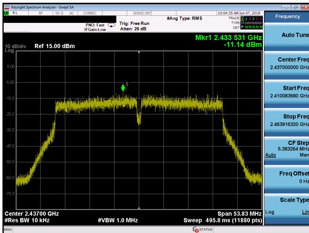
Plot 7-23. Power Spectral Density Plot (40MHz 802.11n (2.4GHz) – Ch. 6)
