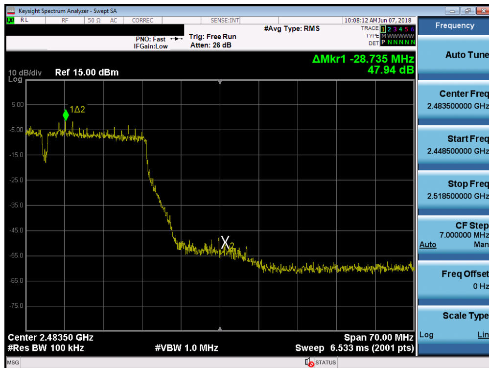
Plot 7-32. Band Edge Plot (40MHz 802.11n (2.4GHz) – Ch. 9)
