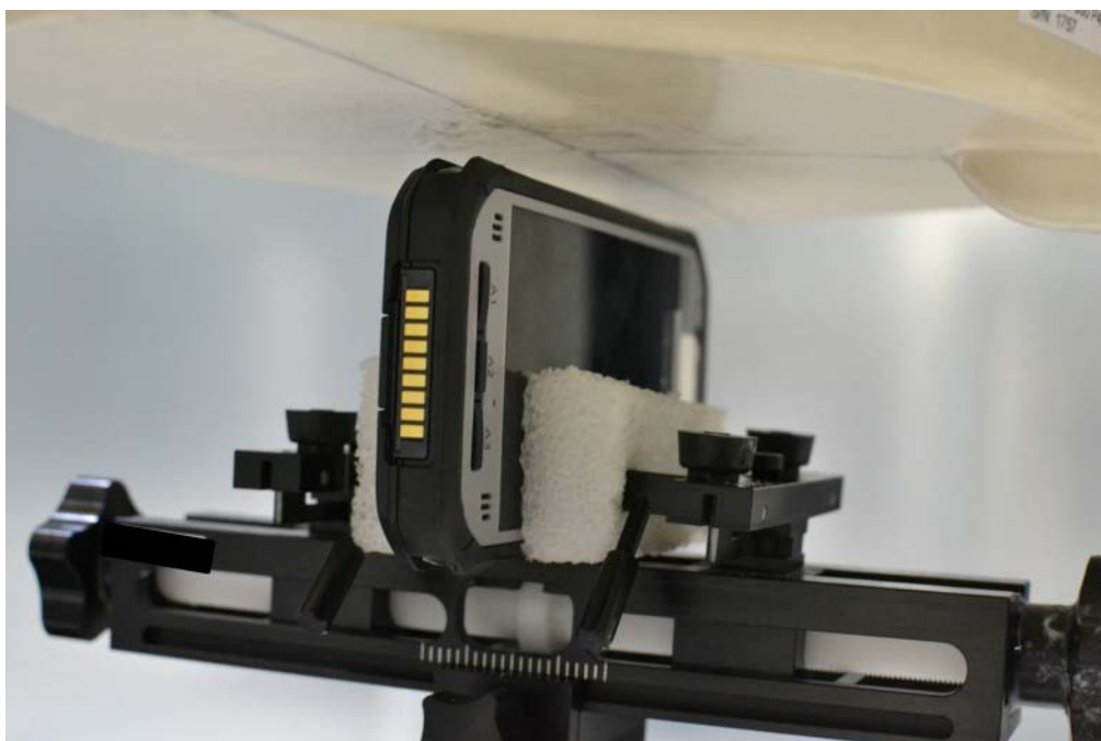
SAR Test Setup Photo 27 – Left Edge at 1.0 cm with Standard Battery
