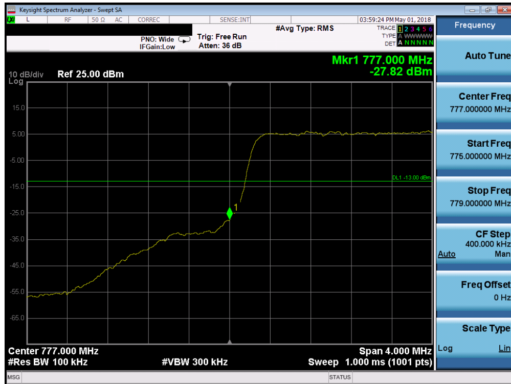
Plot 7-98. Lower Band Edge Plot (Band 13 - 5.0MHz QPSK - Full RB Configuration)
