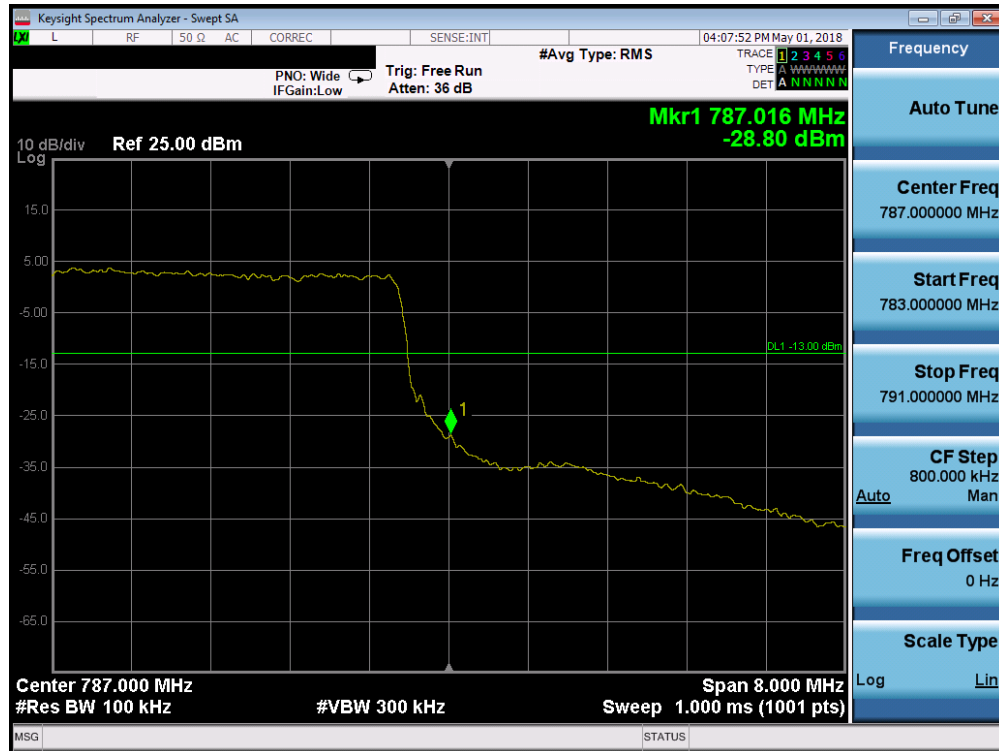
Plot 7-104. Upper Band Edge Plot (Band 13 - 10.0MHz QPSK - Full RB Configuration)
