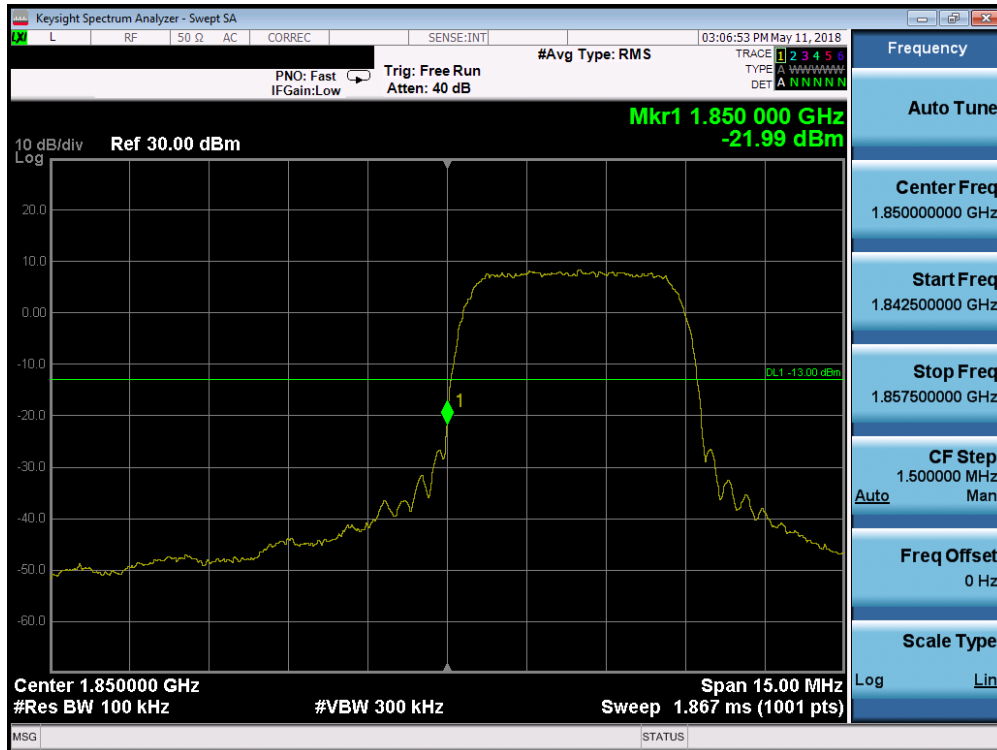
Plot 7-23. Band Edge Plot (PCS WCDMA Mode - Low Channel)
