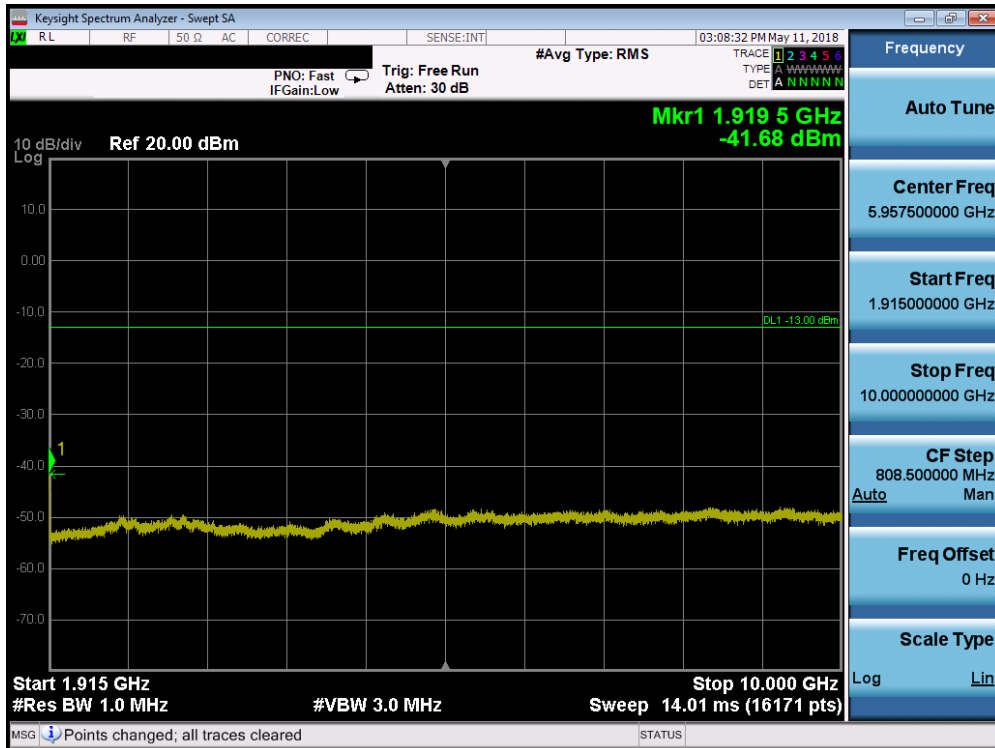
Plot 7-19. Conducted Spurious Plot (PCS WCDMA Mode - High Channel)
