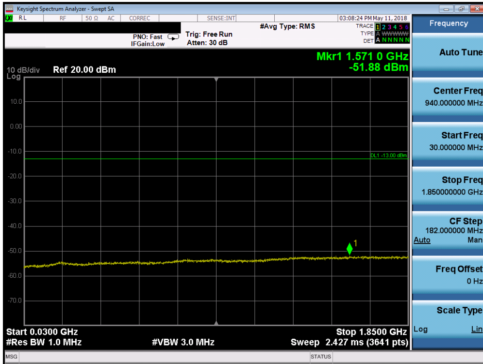
Plot 7-18. Conducted Spurious Plot (PCS WCDMA Mode - High Channel)
