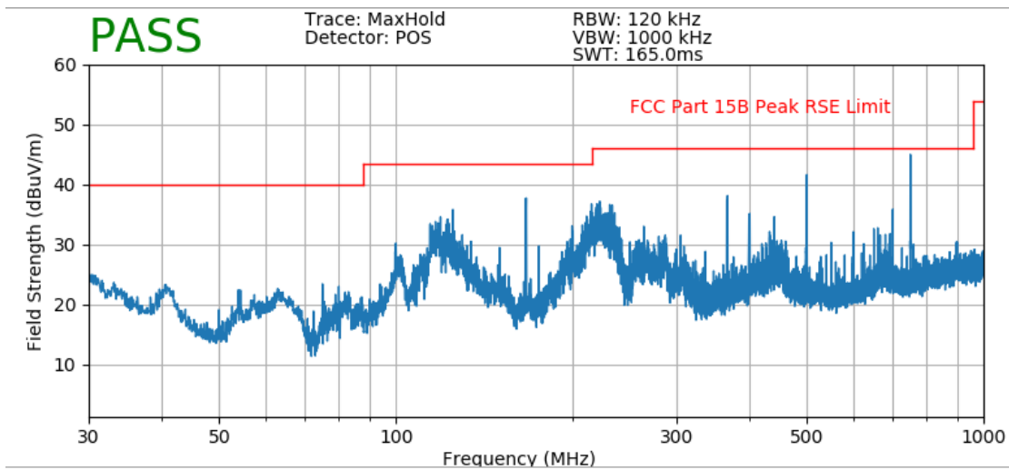
Plot 7-1. Radiated Prescan Plot (H)
