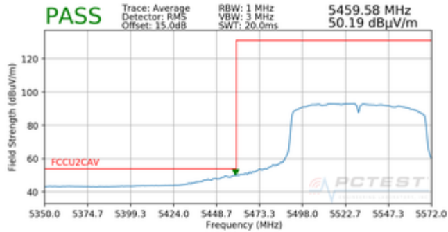
Plot 7-112. Radiated Band Edge Plot (Average – Rugged USB Dock)
