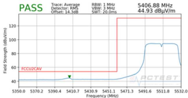
Plot 7-102. Radiated Band Edge Plot (Average – Rugged USB Dock)
