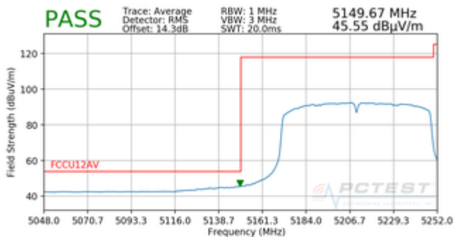
Plot 7-104. Radiated Lower Band Edge Plot (Average – UNII Band 1)
