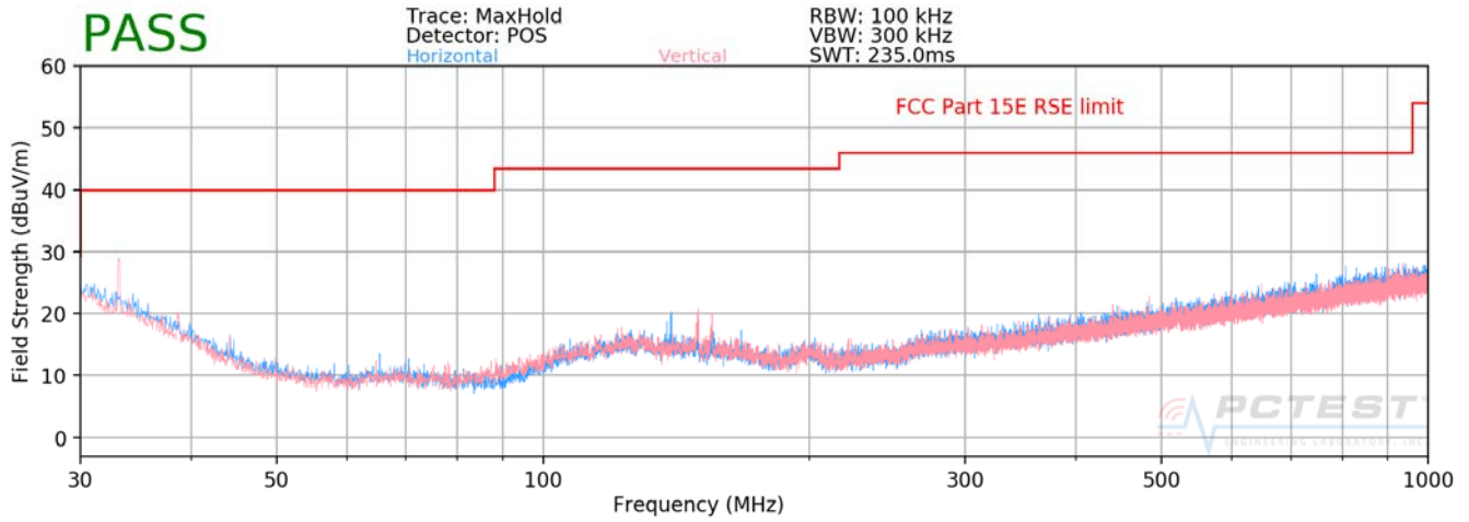
Plot 7-114. Radiated Spurious Plot below 1GHz (802.11a – U3 Ch. 157)
