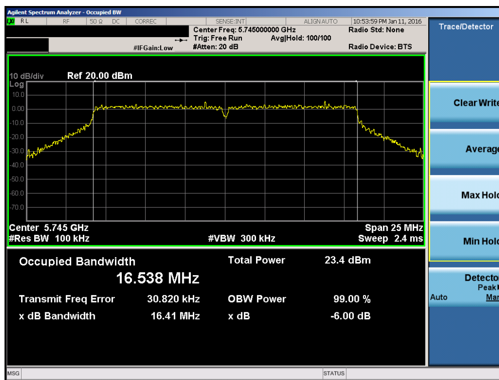
Plot 7-29. 6dB Bandwidth Plot (802.11a (UNII Band 3) – Ch. 149)
