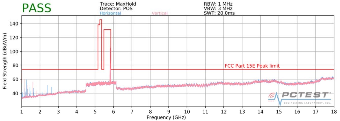
Plot 7-78. Radiated Spurious Plot above 1GHz (802.11a – U3 Ch. 165)
