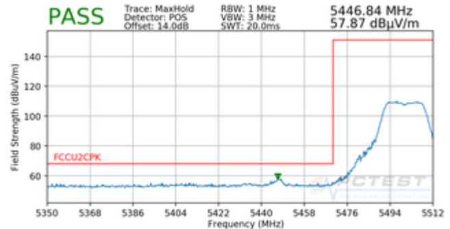
Plot 7-87. Radiated Lower Band Edge Plot (Peak – UNII Band 2C)
