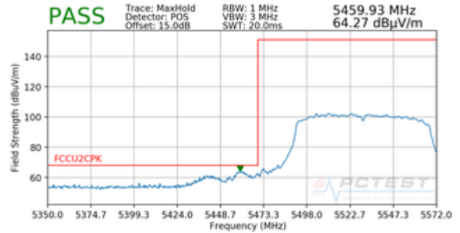
Plot 7-113. Radiated Band Edge Plot (Peak – Rugged USB Dock)
