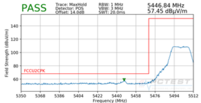
Plot 7-92. Radiated Band Edge Plot (Peak – Rugged USB Dock)
