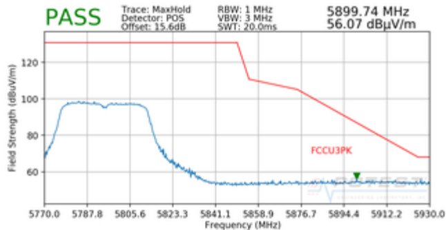
Plot 7-101. Radiated Upper Band Edge Plot (Peak – UNII Band 3)
