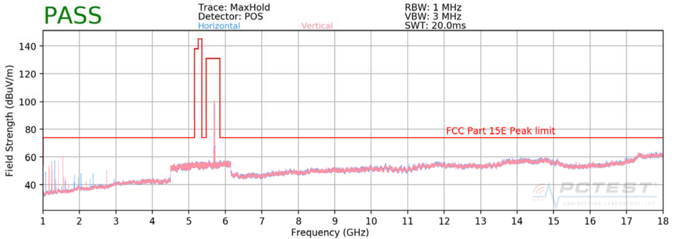
Plot 7-77. Radiated Spurious Plot above 1GHz (802.11a – U2C Ch. 140)
