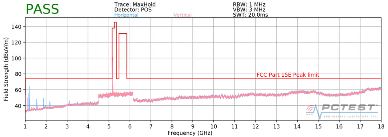
Plot 7-75. Radiated Spurious Plot above 1GHz (802.11a – U1 Ch. 40)
