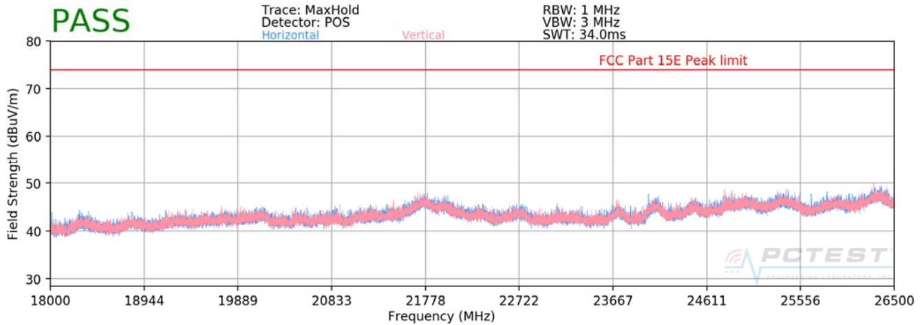
Plot 7-79. Radiated Spurious Plot 18GHz - 26.5GHz (802.11a)
