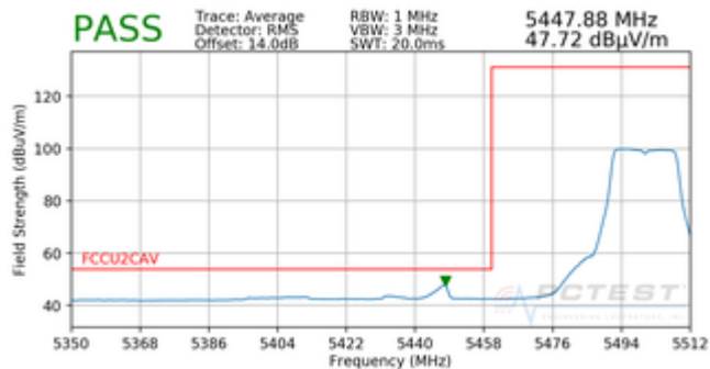
Plot 7-91. Radiated Band Edge Plot (Average – Rugged USB Dock)
