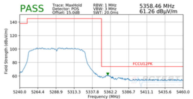
Plot 7-107. Radiated Upper Band Edge Plot (Peak – UNII Band 2A)
