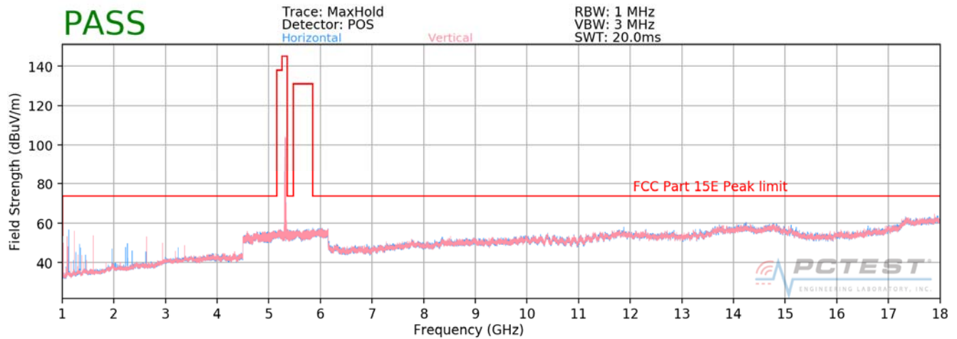
Plot 7-76. Radiated Spurious Plot above 1GHz (802.11a – U2A Ch. 64)
