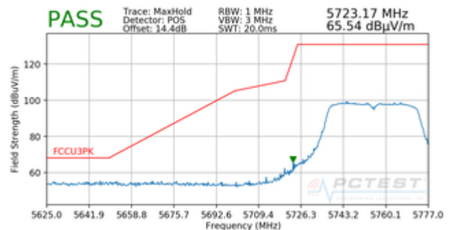
Plot 7-100. Radiated Lower Band Edge Plot (Peak – UNII Band 3)
