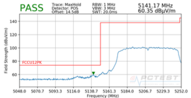
Plot 7-105. Radiated Lower Band Edge Plot (Peak – UNII Band 1)
