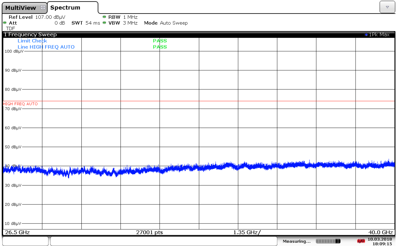
Plot 7-81. Radiated Spurious Plot 26.5GHz - 40GHz (802.11a) (V)
