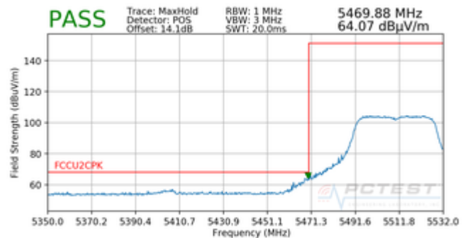
Plot 7-103. Radiated Band Edge Plot (Peak – Rugged USB Dock)
