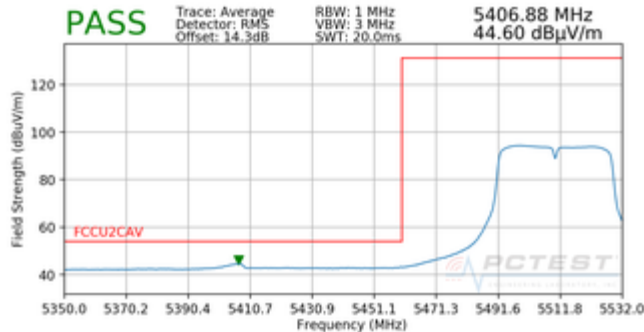
Plot 7-97. Radiated Lower Band Edge Plot (Average – UNII Band 2C)
