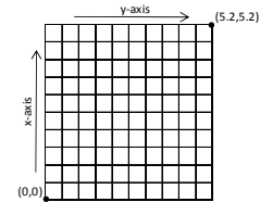
Figure 4-12 Measurement Grid
