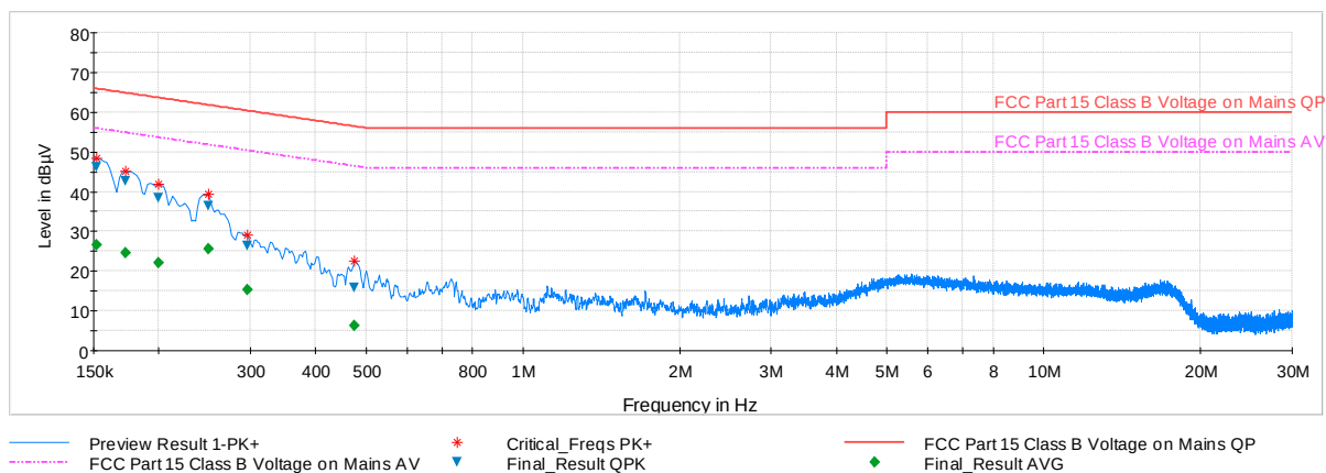
Plot 7-51. Line Conducted Plot with 802.11b (L1)
