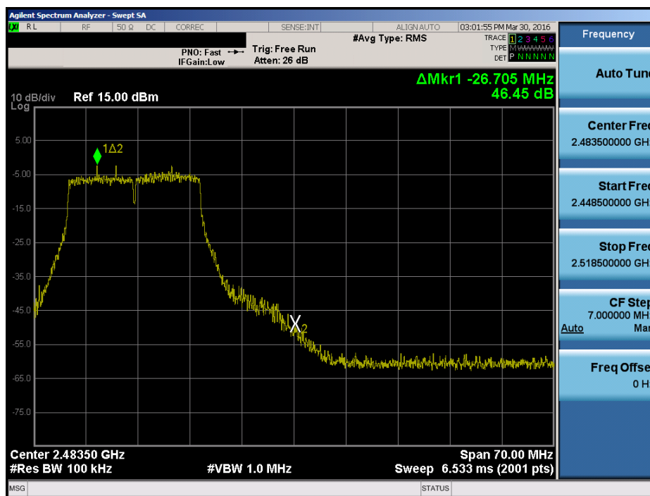
Plot 7-28. Band Edge Plot (802.11n (2.4GHz) – Ch. 11)
