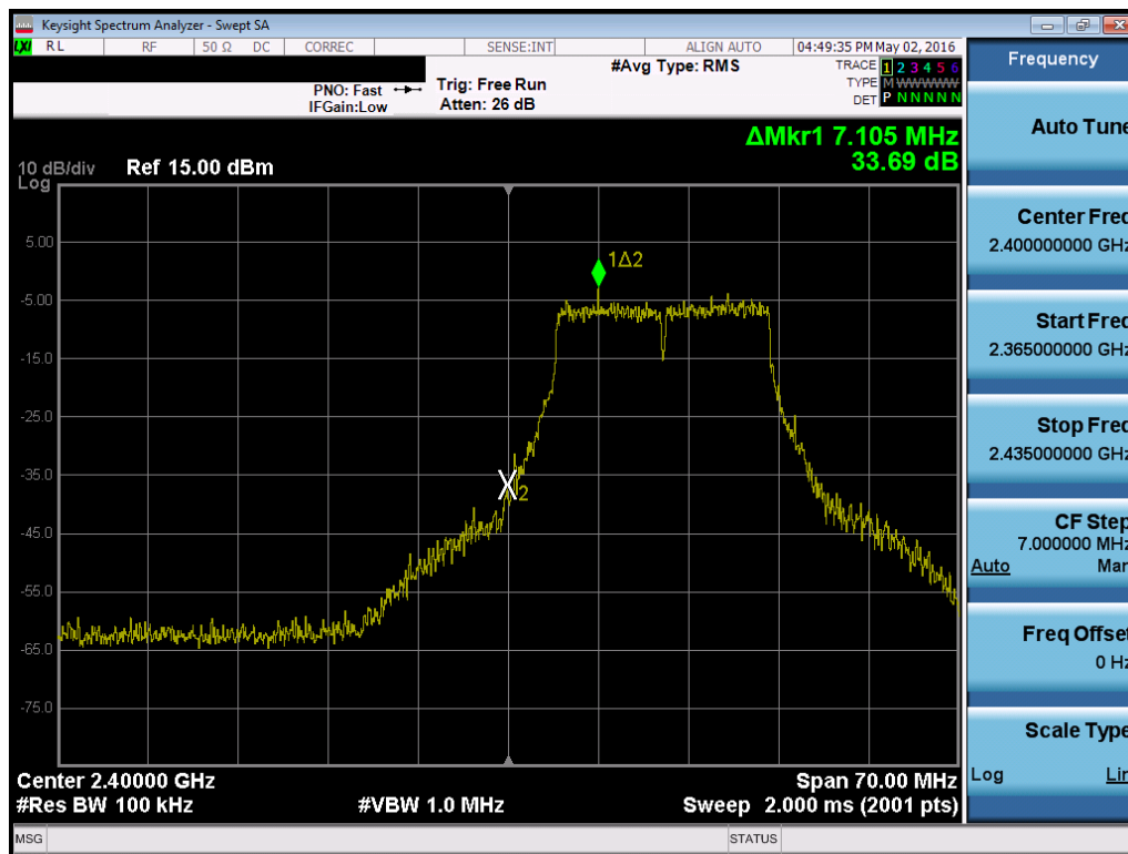
Plot 7-21. Band Edge Plot (802.11g– Ch. 1)
