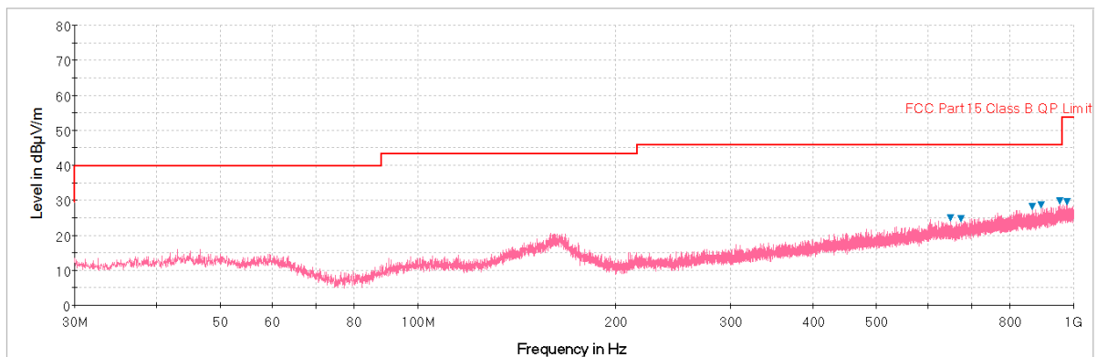
Plot 7-50. Radiated Spurious Plot below 1GHz (Pol. V)
