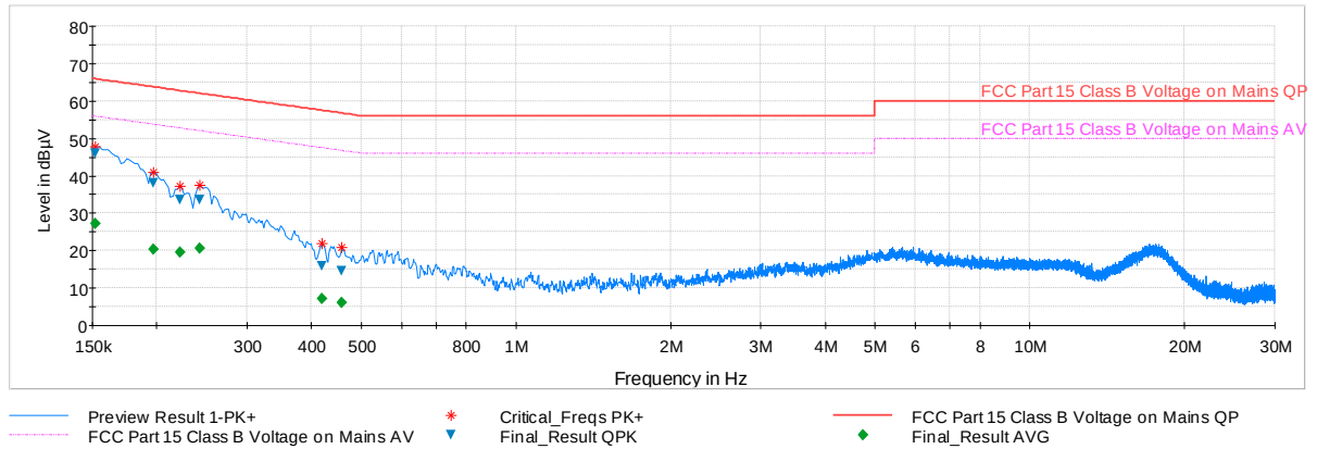
Plot 7-52. Line Conducted Plot with 802.11b (N)
