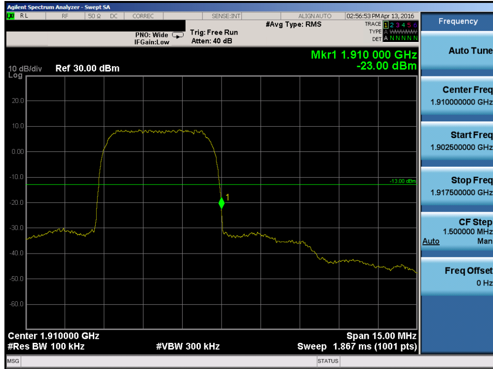
Plot 7-81. Band Edge Plot (PCS WCDMA Mode – Ch. 9538)
