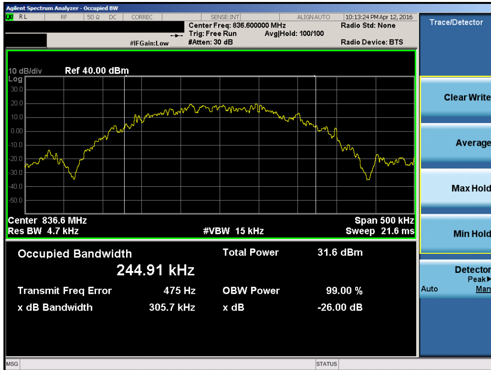
Plot 7-2. Occupied Bandwidth Plot (Cellular EDGE Mode – Ch. 190)
