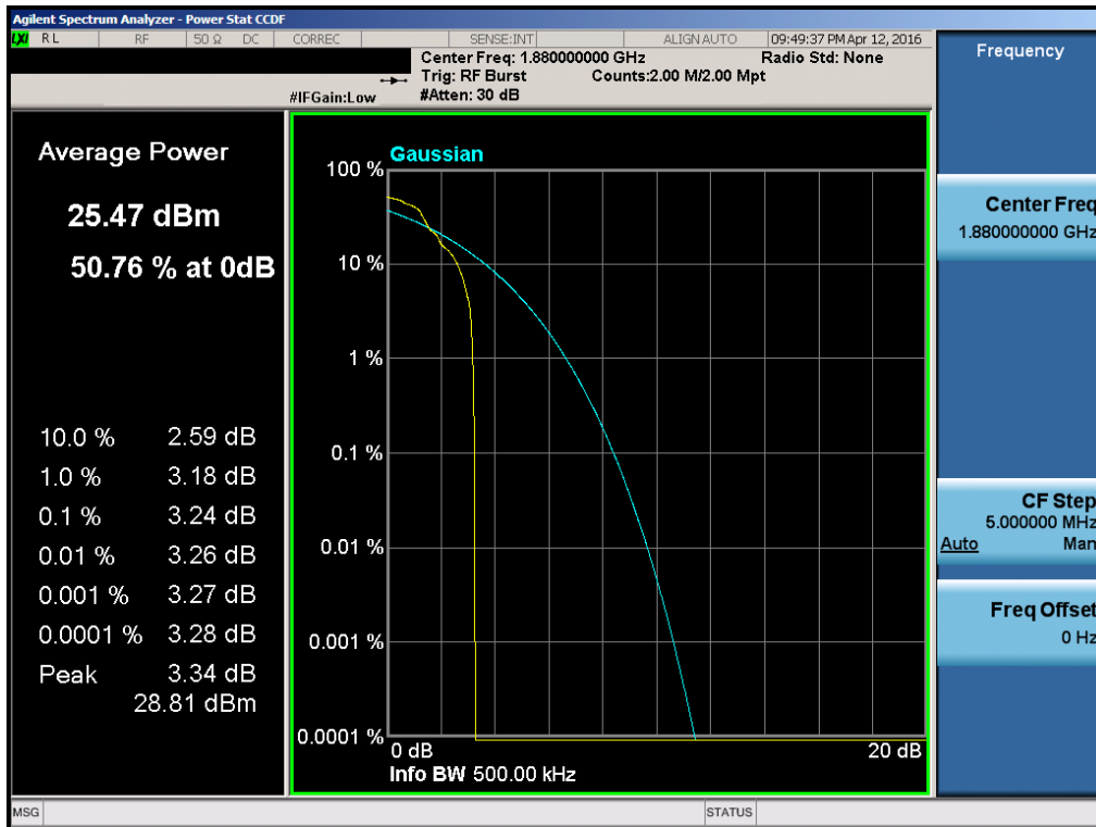
Plot 7-84. Peak-Average Ratio Plot (PCS EDGE Mode – Ch. 661)
