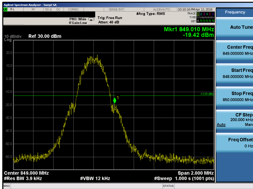
Plot 7-64. Band Edge Plot (Cellular GSM Mode – Ch. 251)
