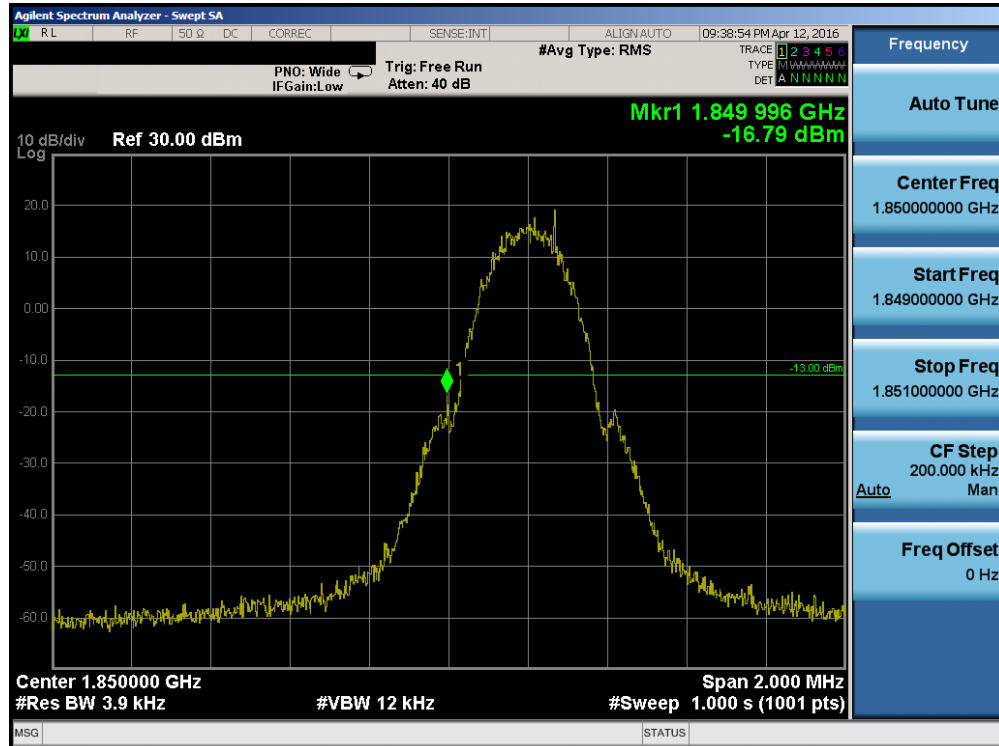
Plot 7-65. Band Edge Plot (PCS GSM Mode – Ch. 512)
