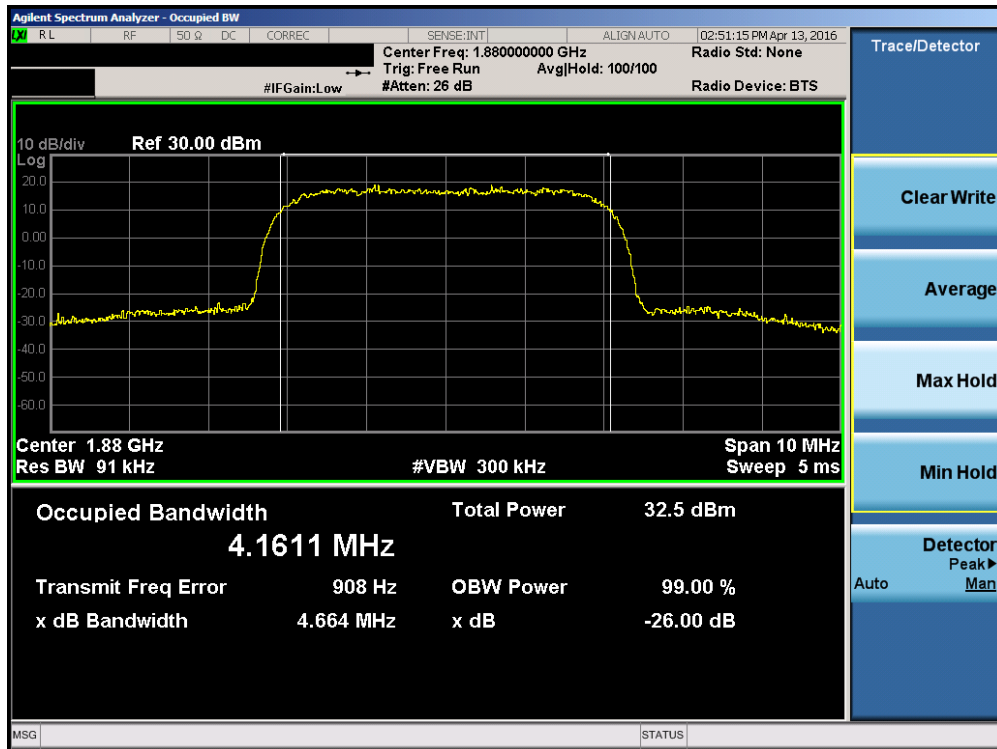
Plot 7-8. Occupied Bandwidth Plot (PCSWCDMA Mode – Ch. 9400)
