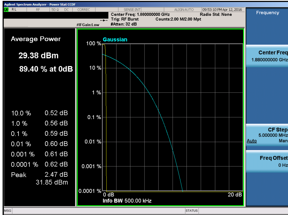
Plot 7-83. Peak-Average Ratio Plot (PCS GSM Mode – Ch. 661)
