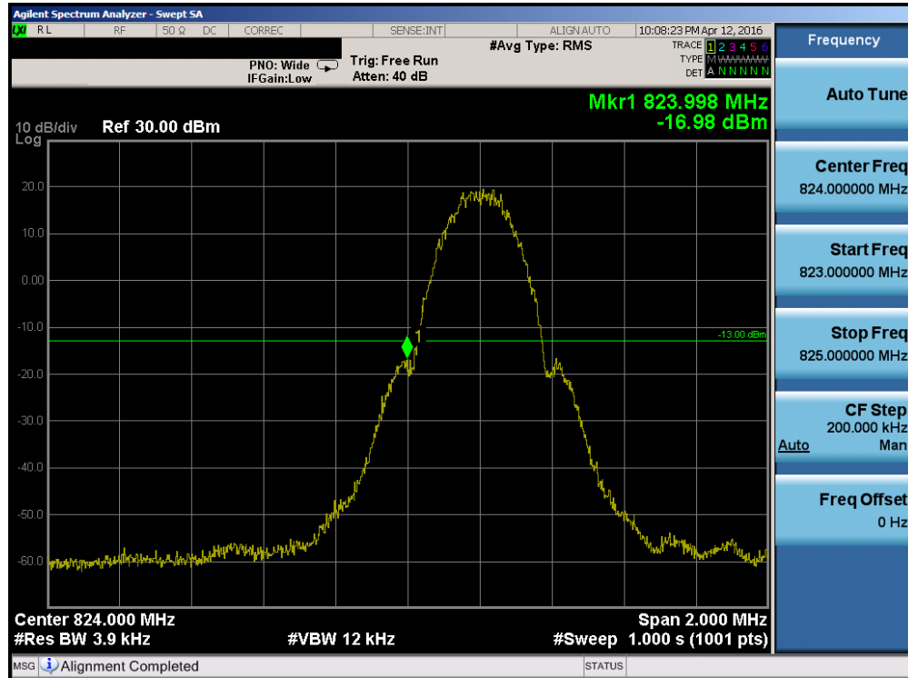
Plot 7-63. Band Edge Plot (Cellular GSM Mode – Ch. 128)
