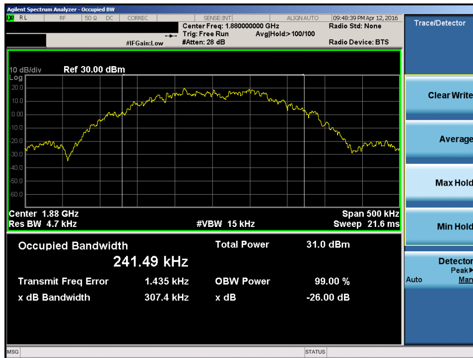
Plot 7-4. Occupied Bandwidth Plot (EDGE GSM Mode – Ch. 661)
