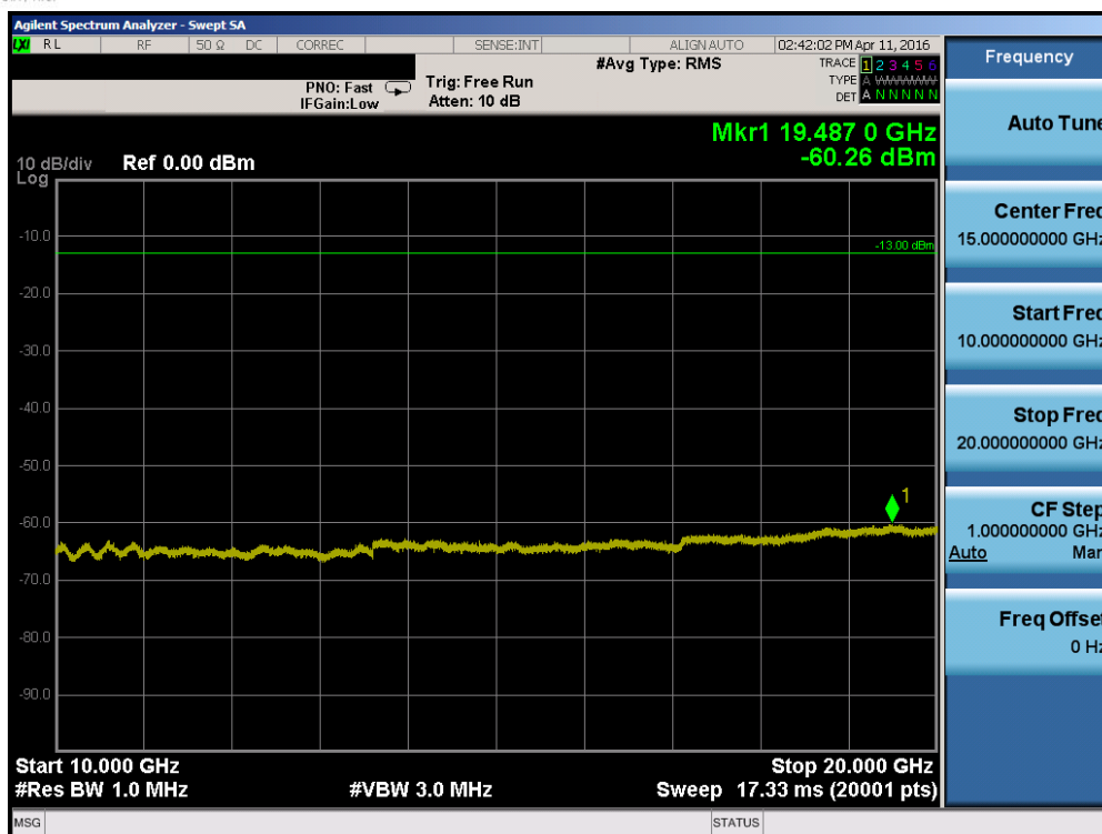
Plot 7-77. Conducted Spurious Plot (Band 2 – 10.0MHz QPSK – RB Size 1, RB Offset 0 – Low Channel)
