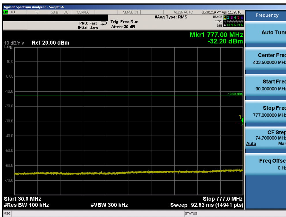
Plot 7-54. Conducted Spurious Plot (Band 13 – 10.0MHz QPSK – RB Size 1, RB Offset 0)
