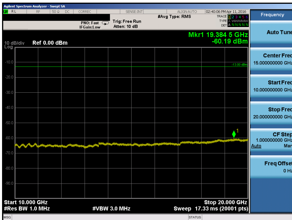
Plot 7-80. Conducted Spurious Plot (Band 2 – 10.0MHz QPSK – RB Size 1, RB Offset 0 – Mid Channel)
