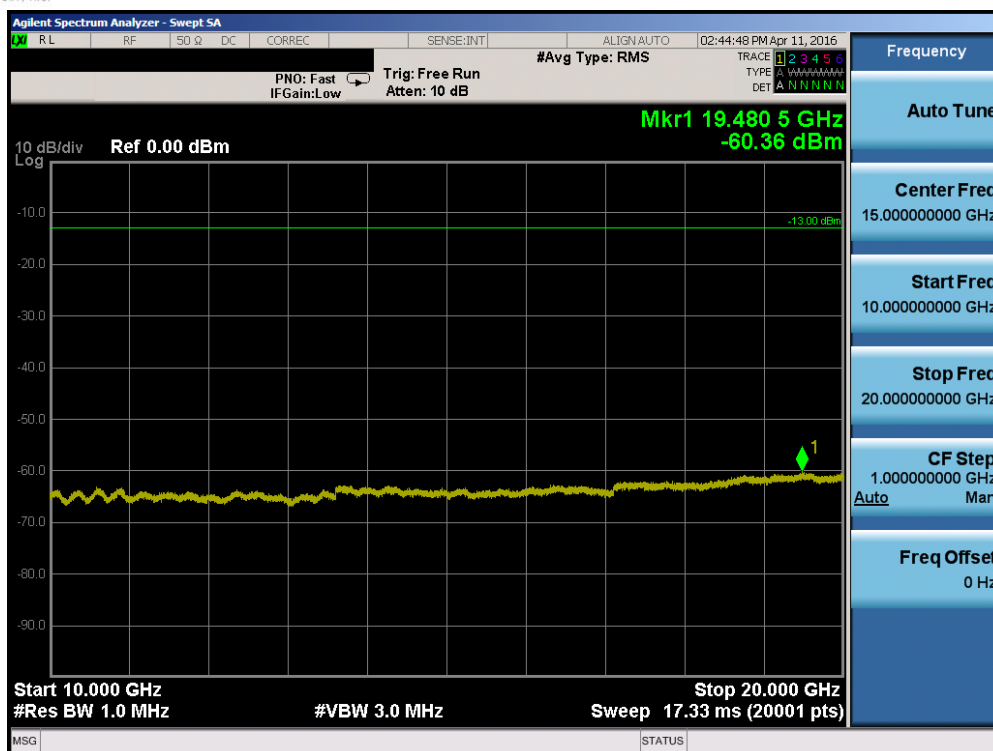
Plot 7-83. Conducted Spurious Plot (Band 2 – 10.0MHz QPSK – RB Size 1, RB Offset 0 – High Channel)
