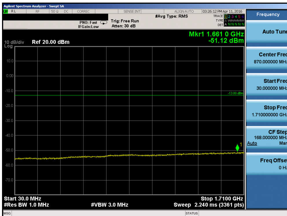
Plot 7-72. Conducted Spurious Plot (Band 4 – 10.0MHz QPSK – RB Size 1, RB Offset 0 – High Channel)
