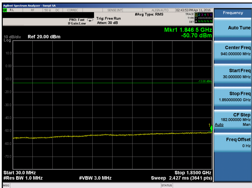
Plot 7-81. Conducted Spurious Plot (Band 2 – 10.0MHz QPSK – RB Size 1, RB Offset 0 – High Channel)
