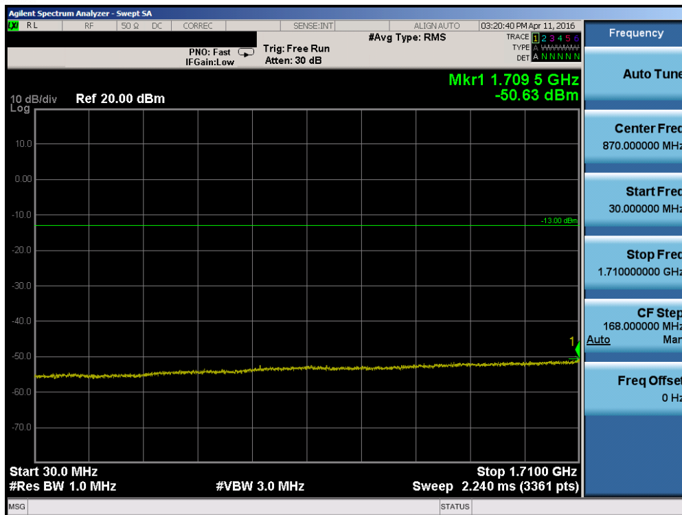
Plot 7-69. Conducted Spurious Plot (Band 4 – 10.0MHz QPSK – RB Size 1, RB Offset 0 – Mid Channel)
