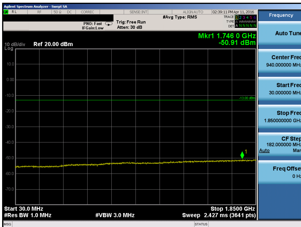
Plot 7-78. Conducted Spurious Plot (Band 2 – 10.0MHz QPSK – RB Size 1, RB Offset 0 – Mid Channel)
