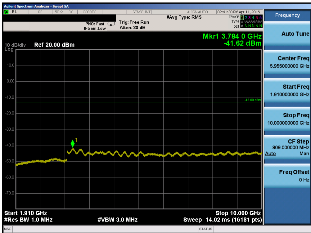
Plot 7-76. Conducted Spurious Plot (Band 2 – 10.0MHz QPSK – RB Size 1, RB Offset 0 – Low Channel)
