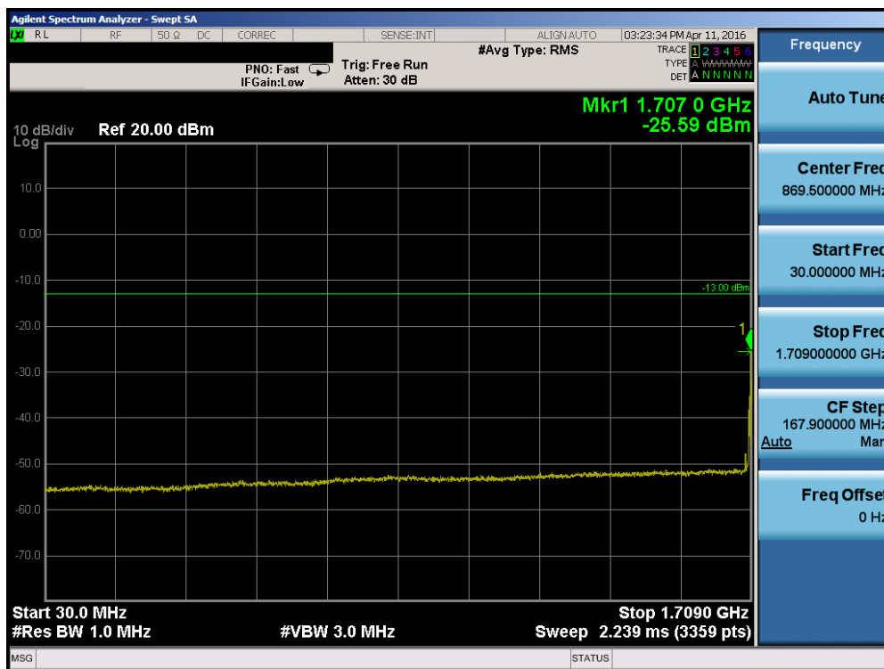
Plot 7-66. Conducted Spurious Plot (Band 4 – 10.0MHz QPSK – RB Size 1, RB Offset 0– Low Channel)
