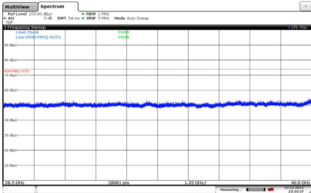
Plot 7-86. Radiated Spurious Plot above 18GHz (802.11a – Ant. Pol. H)
