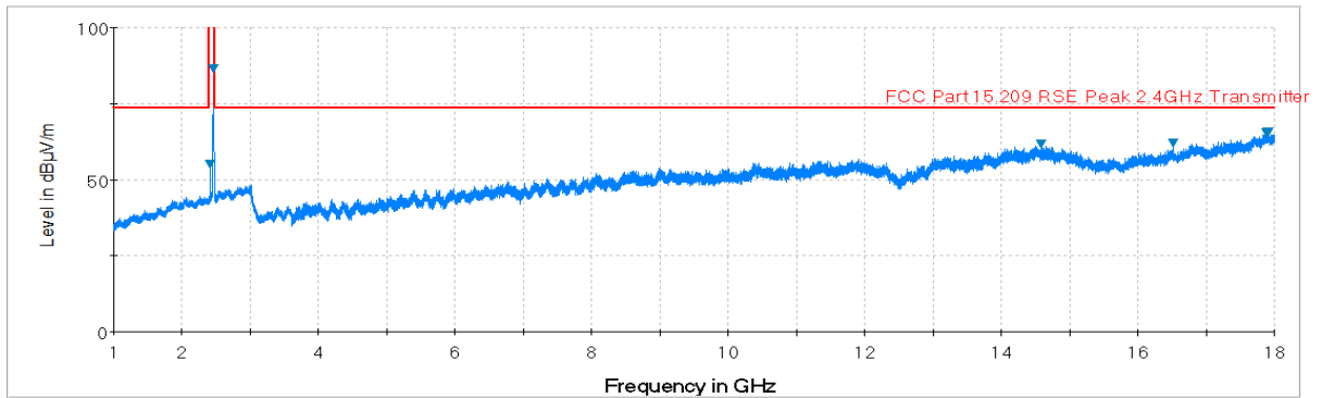
Plot 7-41. Radiated Spurious Plot above 1GHz (802.11b – Ch. 11, Ant. Pol. H)
