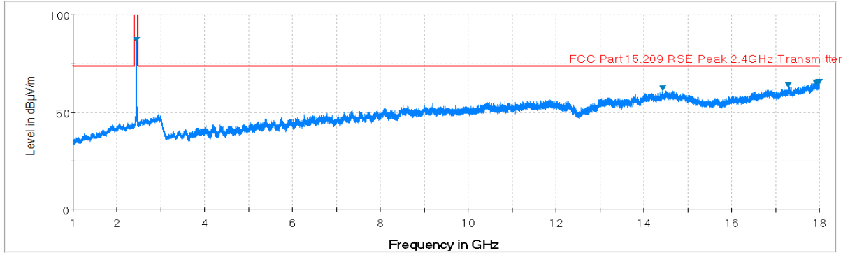
Plot 7-40. Radiated Spurious Plot above 1GHz (802.11b – Ch. 6, Ant. Pol. V)
