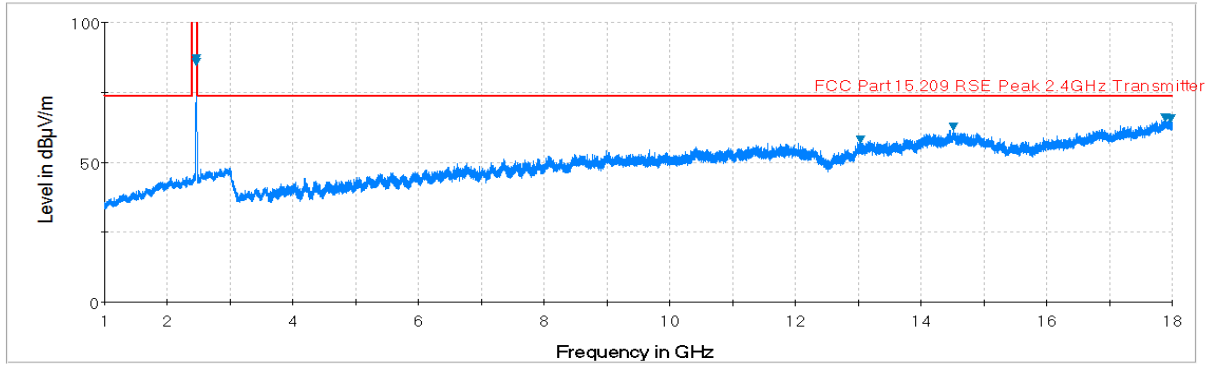
Plot 7-42. Radiated Spurious Plot above 1GHz (802.11b – Ch. 11, Ant. Pol. V)
