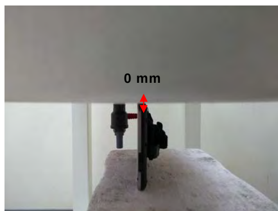
Fig.19 EUT Bottom side(Hand Strap 13U) to flat phantom
