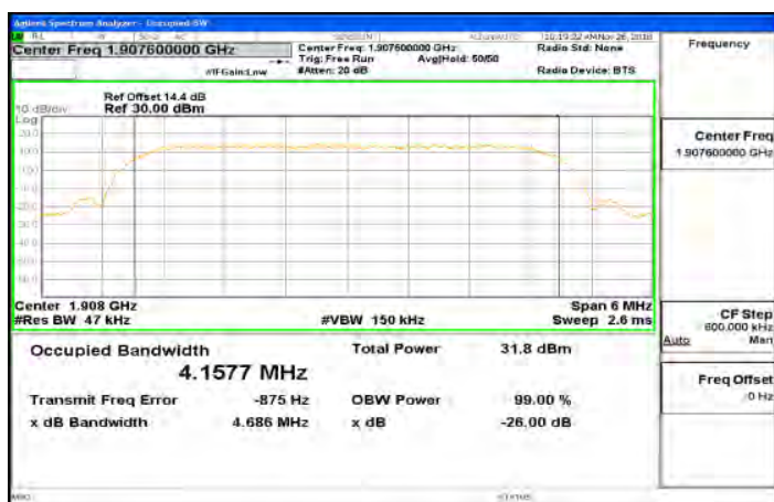
HSDPA_B2_HighCH9538-1907.6
