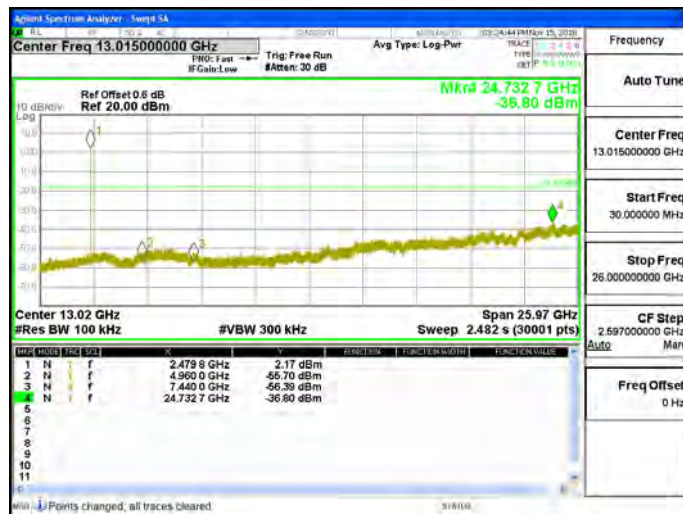
Spurious Emission_8DPSK_3M_DH5_2480MHz
