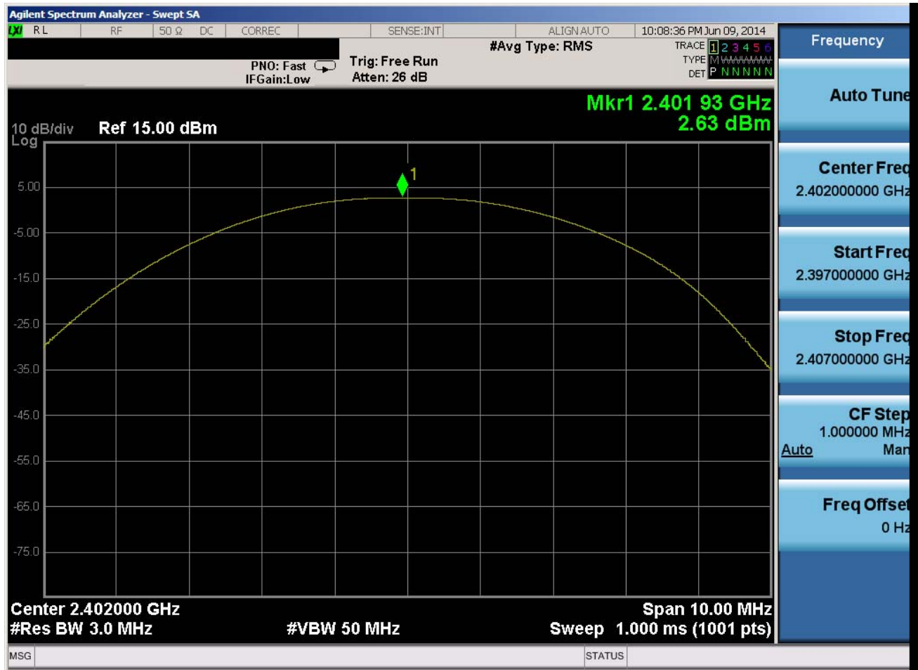
Plot 6-4. Peak Power Plot (Bluetooth (LE) – Ch. 0)
