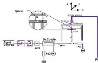
Figure 9-1 System Verification Setup Diagram
