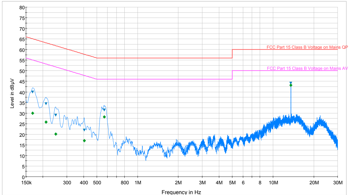
Plot 8-2. Line-Conducted Test Plot (N)
