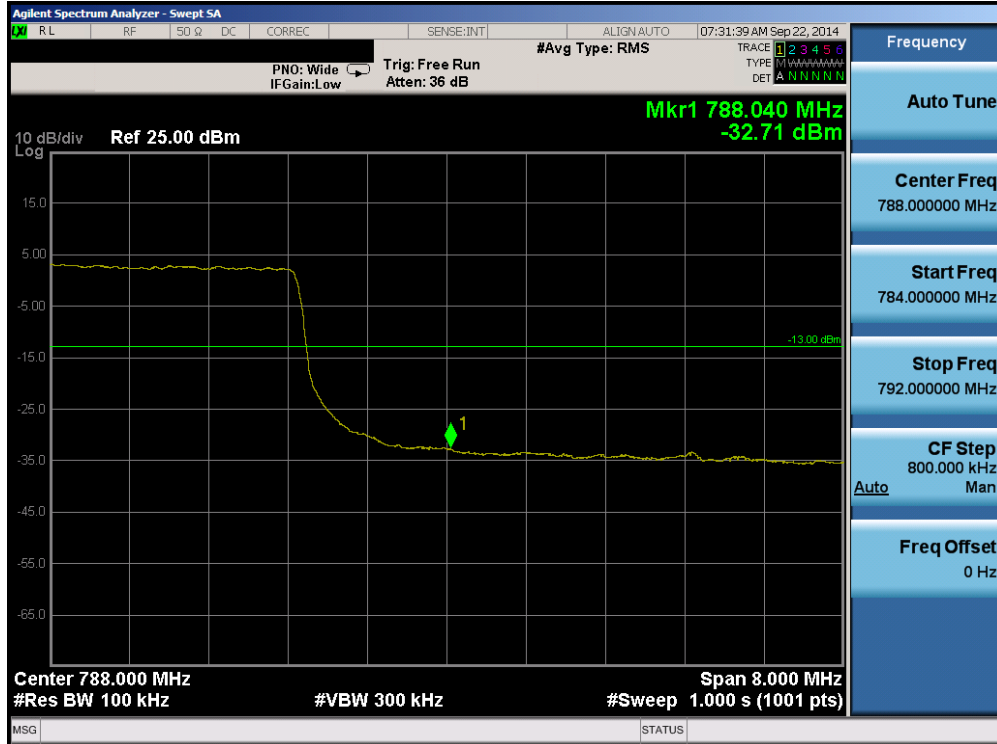
Plot 6-37. Upper Band Edge Plot (Band 13 – 10.0MHz QPSK – RB Size 50)
