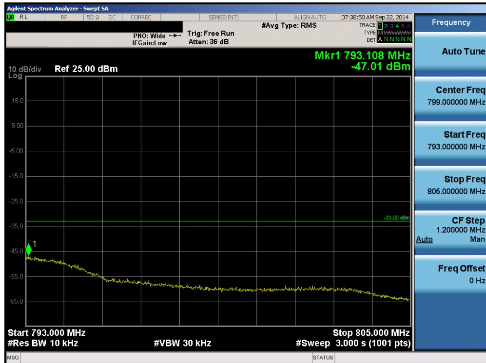
Plot 6-38. Upper Extended Band Edge Plot (Band 13 – 10.0MHz QPSK – RB Size 50)
