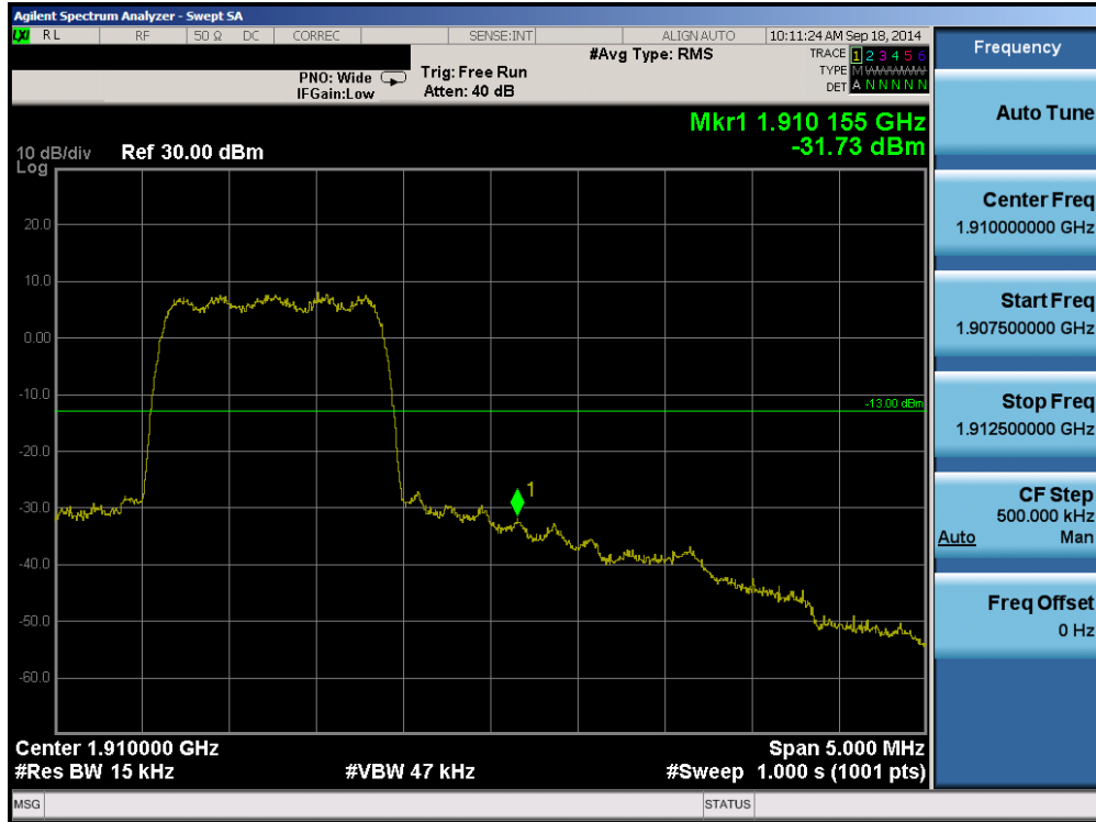
Plot 6-58. Band Edge Plot (PCS CDMA Mode – Ch. 1175)
