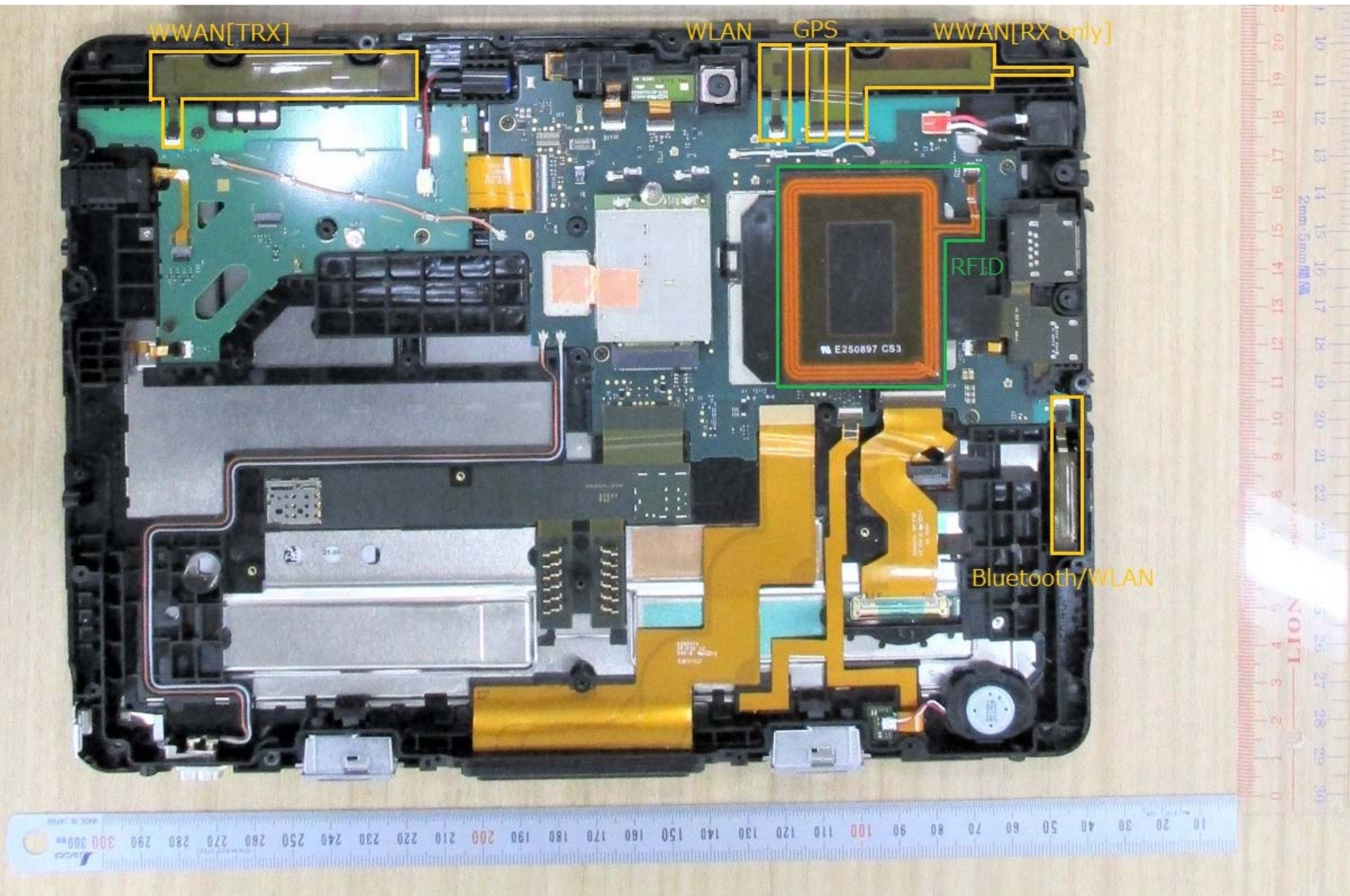
Model with external antenna ports
