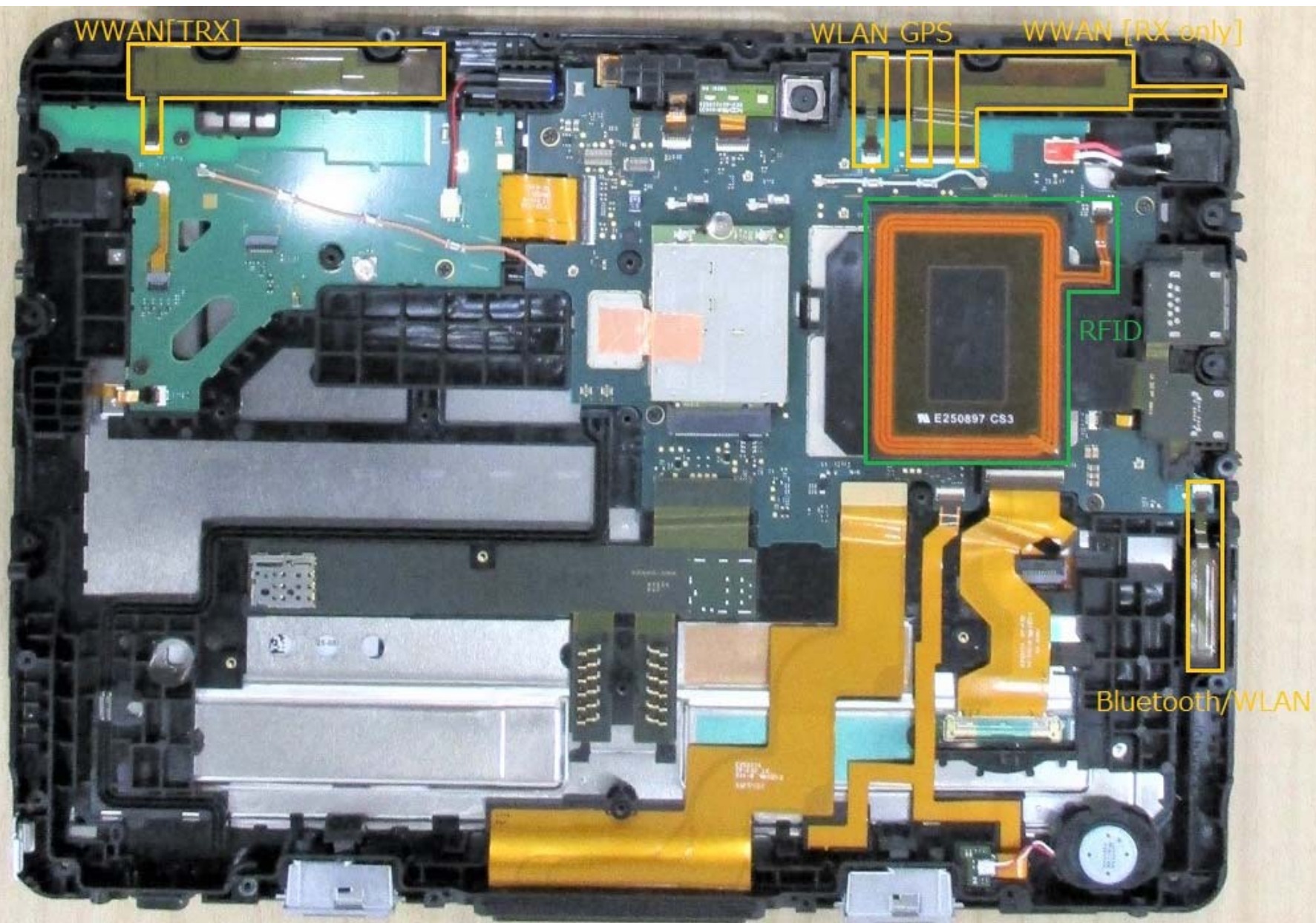
Model without external antenna port
