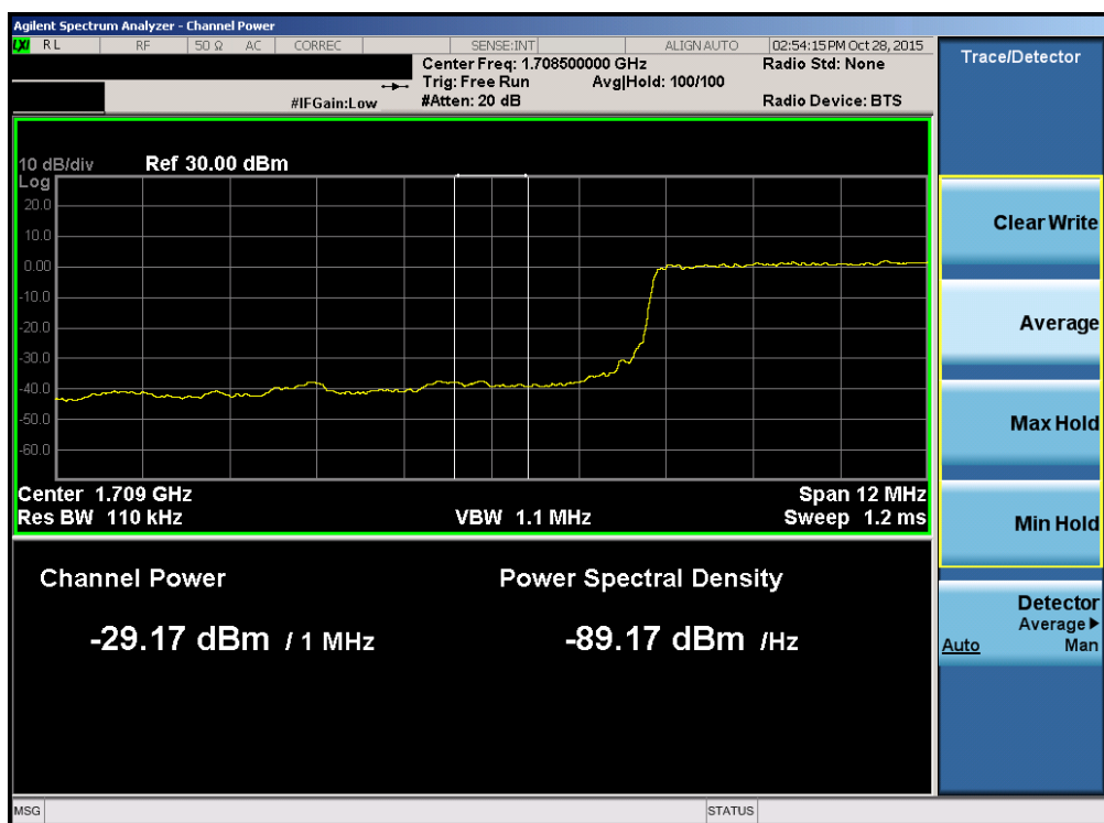
Plot 7-15. Lower Extended Band Edge Plot (Band 4 – 15.0MHz QPSK – RB Size 75)
