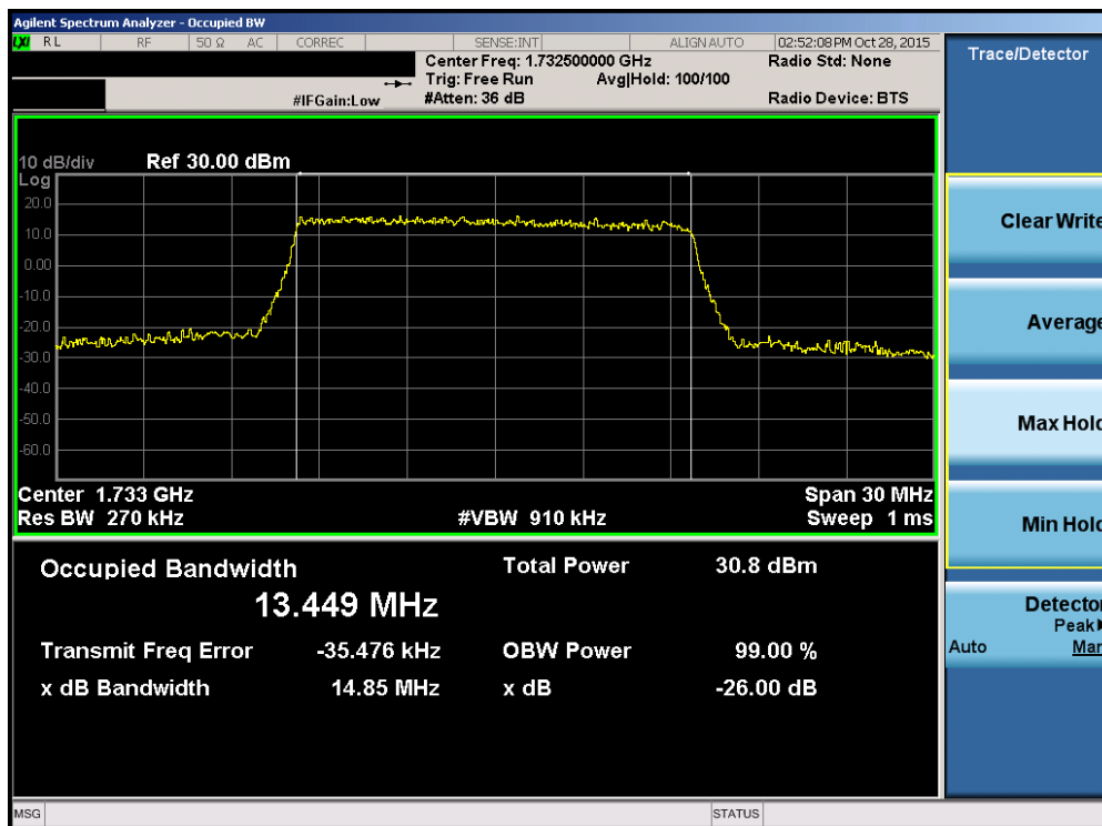
Plot 7-1. Occupied Bandwidth Plot (Band 4 – 15.0MHz QPSK – RB Size 75)
