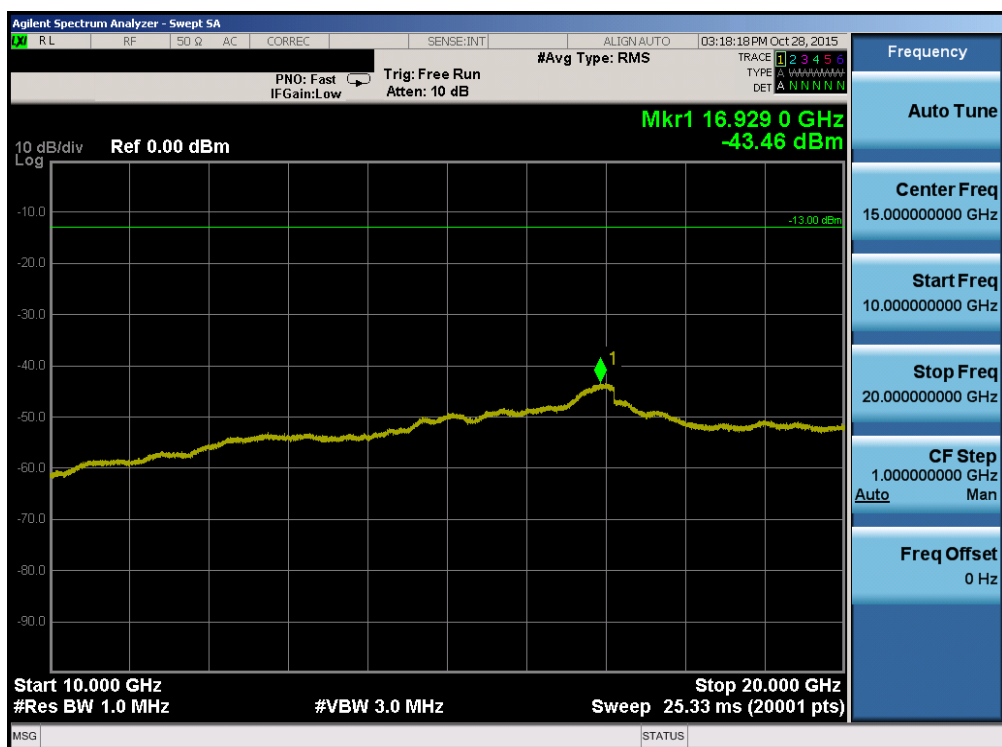
Plot 7-10. Conducted Spurious Plot (Band 4 – 15.0MHz QPSK – RB Size 1, RB Offset 0 – Mid Channel)
