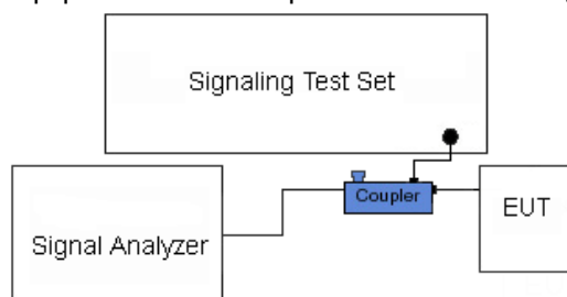
Figure 7-3. Test Instrument & Measurement Setup
