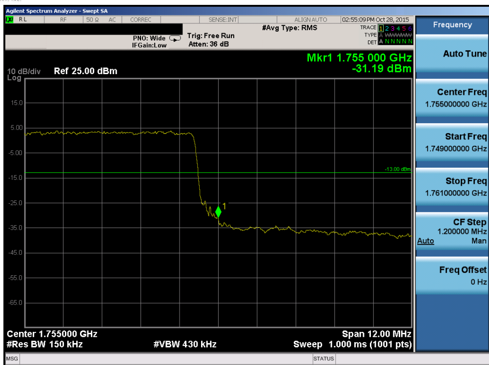
Plot 7-16. Upper Band Edge Plot (Band 4 – 15.0MHz QPSK – RB Size 75)
