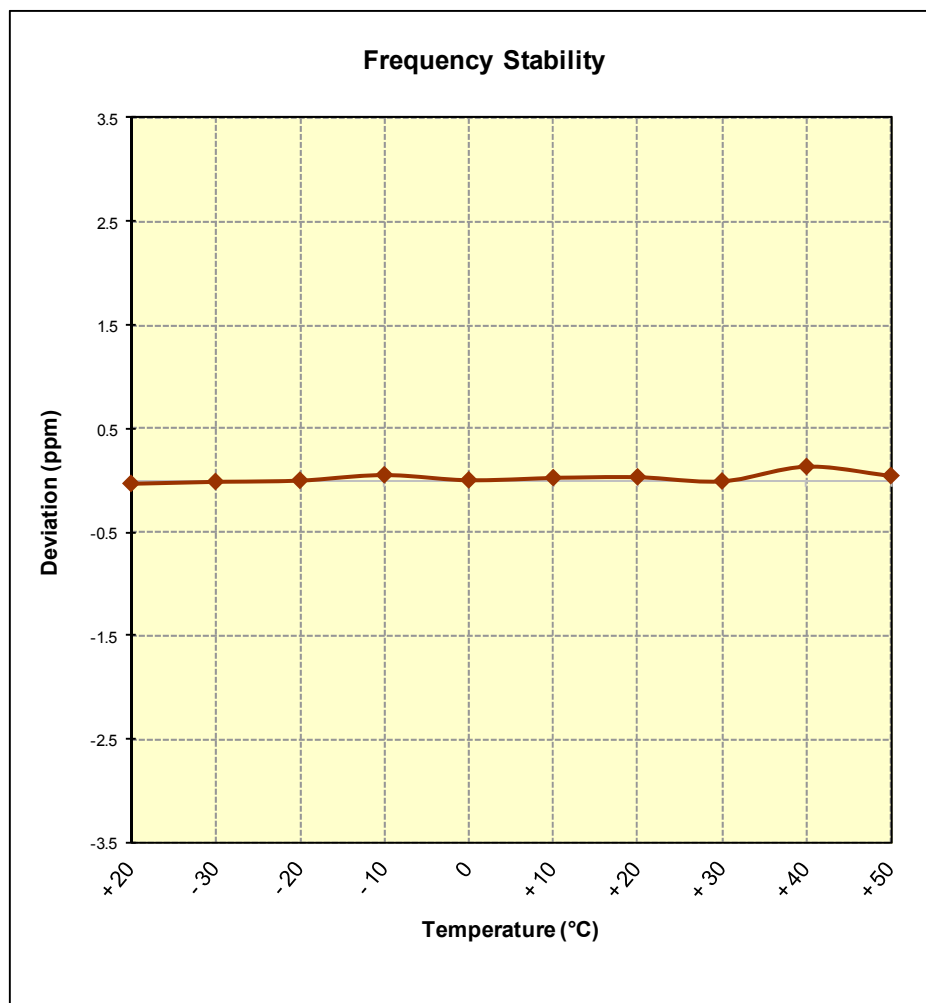
Figure 7-7. Frequency Stability Graph (Band 4)
