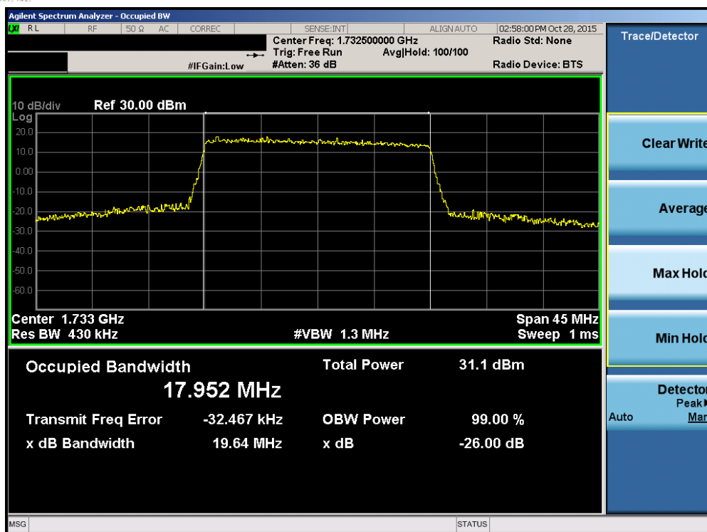
Plot 7-3. Occupied Bandwidth Plot (Band 4 – 20.0MHz QPSK – RB Size 100)
