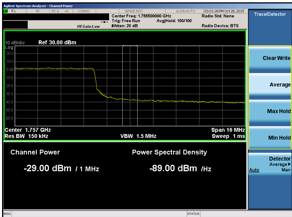
Plot 7-21. Upper Extended Band Edge Plot (Band 4 – 20.0MHz QPSK – RB Size 100)
