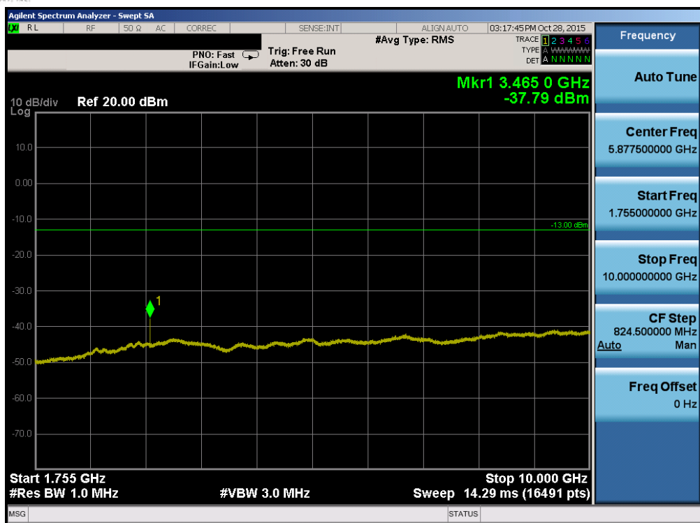
Plot 7-9. Conducted Spurious Plot (Band 4 – 15.0MHz QPSK – RB Size 1, RB Offset 0 – Mid Channel)
