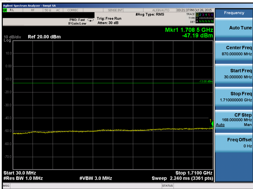
Plot 7-11. Conducted Spurious Plot (Band 4 – 15.0MHz QPSK – RB Size 1, RB Offset 0 – High Channel)
