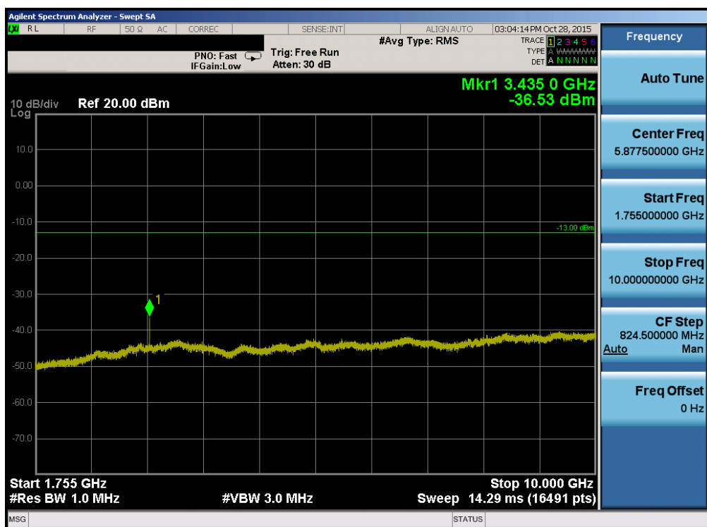
Plot 7-6. Conducted Spurious Plot (Band 4 – 15.0MHz QPSK – RB Size 1, RB Offset 0 – Low Channel)
