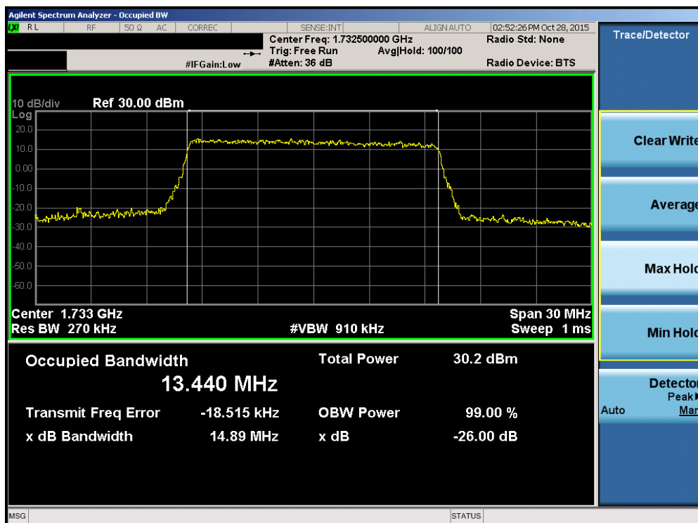
Plot 7-2. Occupied Bandwidth Plot (Band 4 – 15.0MHz 16-QAM – RB Size 75)
