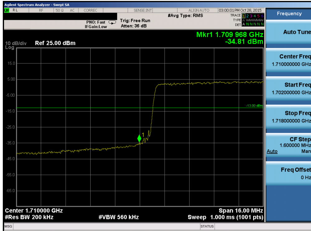
Plot 7-18. Lower Band Edge Plot (Band 4 – 20.0MHz QPSK – RB Size 100)
