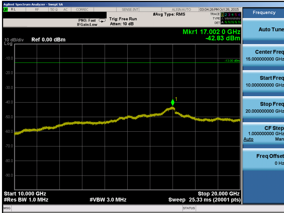
Plot 7-7. Conducted Spurious Plot (Band 4 – 15.0MHz QPSK – RB Size 1, RB Offset 0 – Low Channel)
