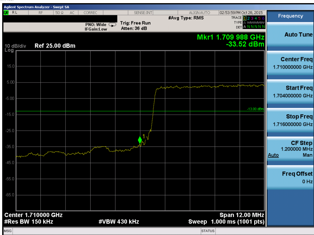
Plot 7-14. Lower Band Edge Plot (Band 4 – 15.0MHz QPSK – RB Size 75)
