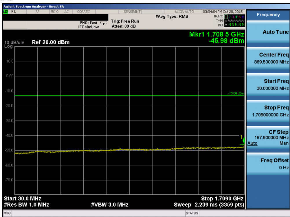
Plot 7-5. Conducted Spurious Plot (Band 4 – 15.0MHz QPSK – RB Size 1, RB Offset 0 – Low Channel)
