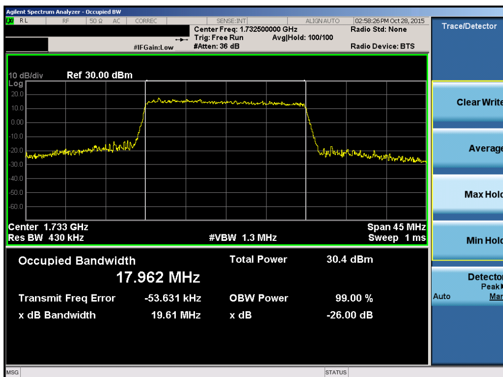
Plot 7-4. Occupied Bandwidth Plot (Band 4 – 20.0MHz 16-QAM – RB Size 100)
