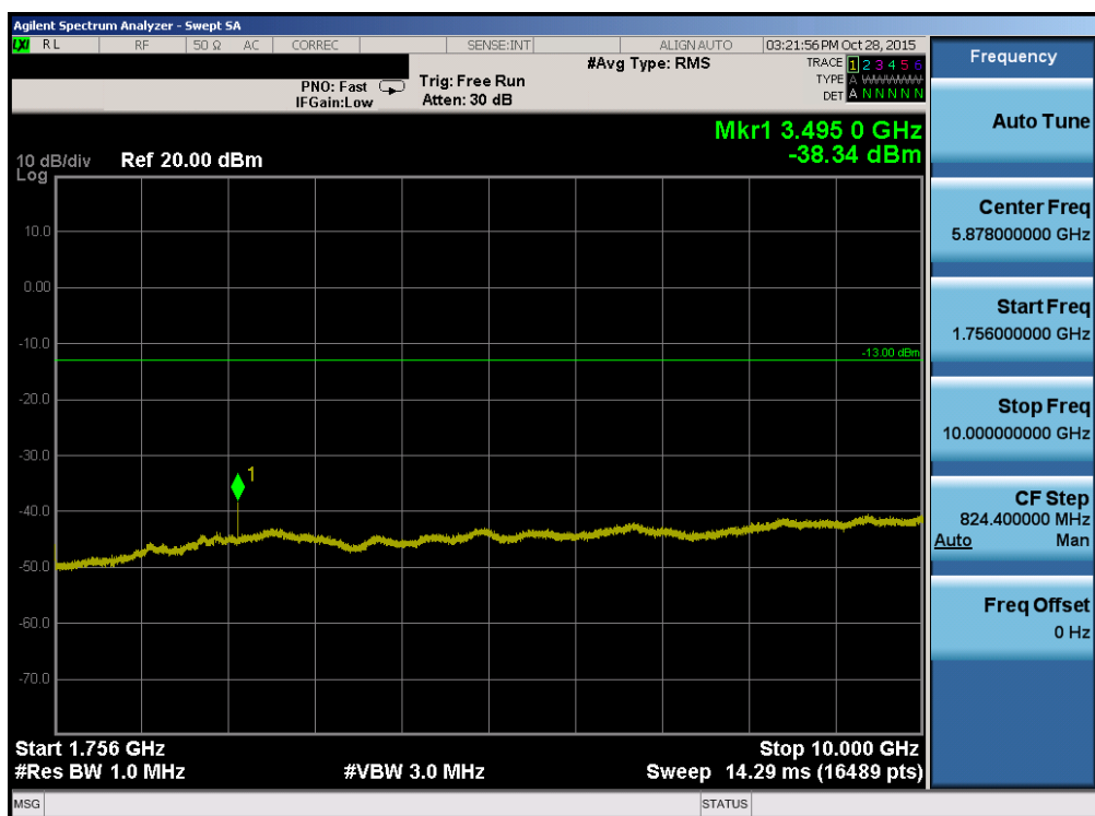
Plot 7-12. Conducted Spurious Plot (Band 4 – 15.0MHz QPSK – RB Size 1, RB Offset 0 – High Channel)
