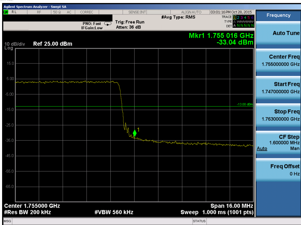
Plot 7-20. Upper Band Edge Plot (Band 4 – 20.0MHz QPSK – RB Size 100)
