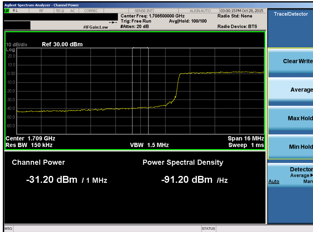
Plot 7-19. Lower Extended Band Edge Plot (Band 4 – 20.0MHz QPSK – RB Size 100)
