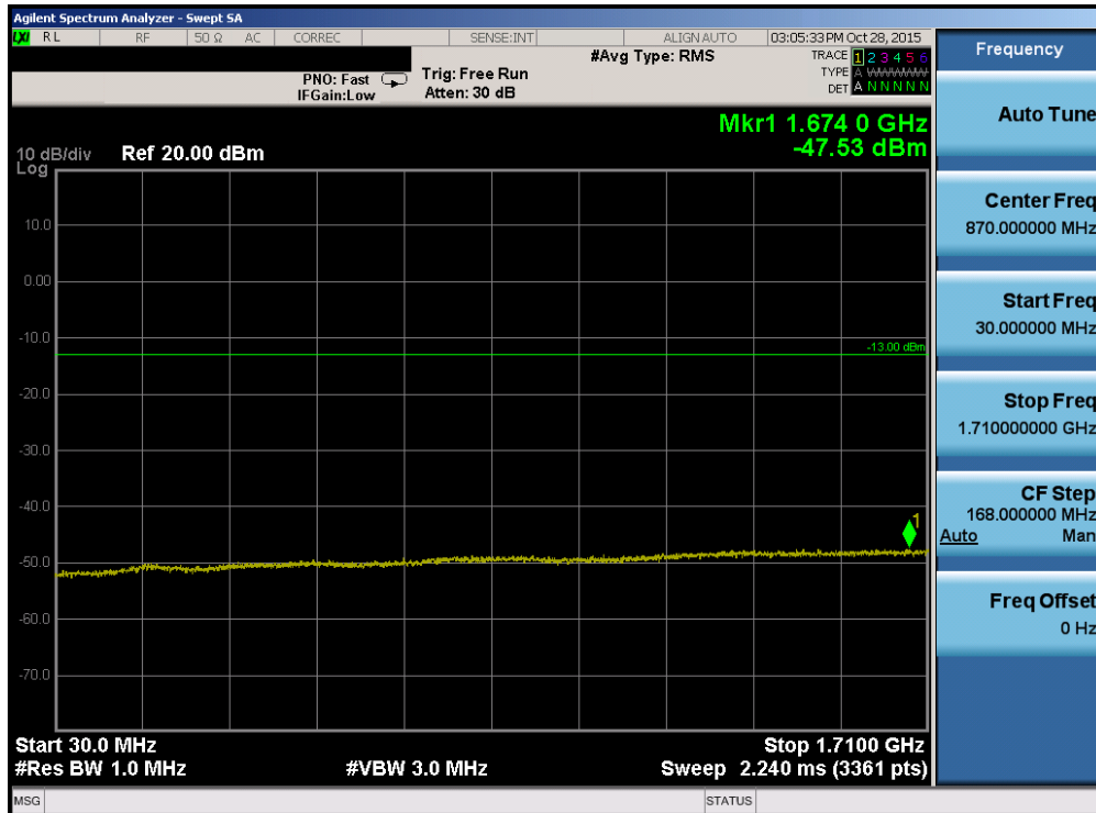
Plot 7-8. Conducted Spurious Plot (Band 4 – 15.0MHz QPSK – RB Size 1, RB Offset 0 – Mid Channel)
