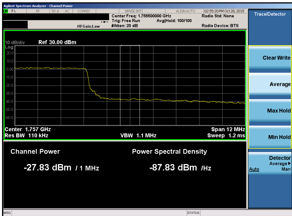
Plot 7-17. Upper Extended Band Edge Plot (Band 4 – 15.0MHz QPSK – RB Size 75)
