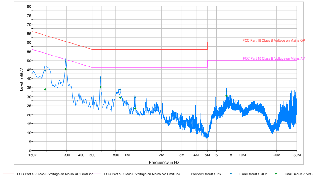
Plot 6-111. Line Conducted Plot with 802.11a UNII Band 2A (L1)
