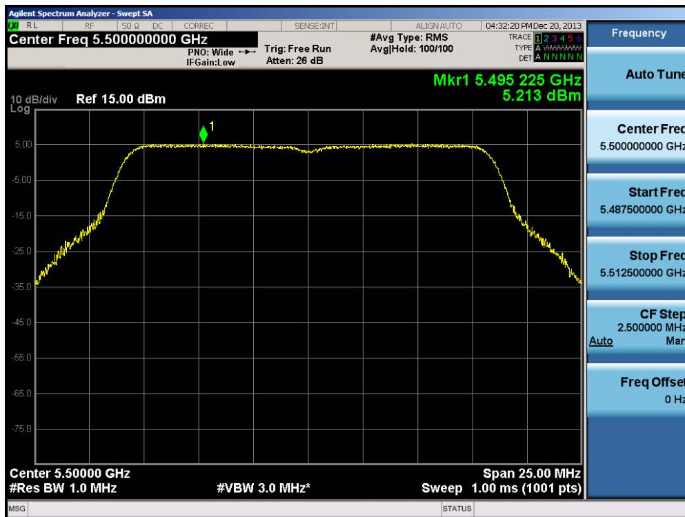
Plot 6-57. Peak Power Spectral Density Plot (802.11a (UNII Band 2C) – Ch. 100)
