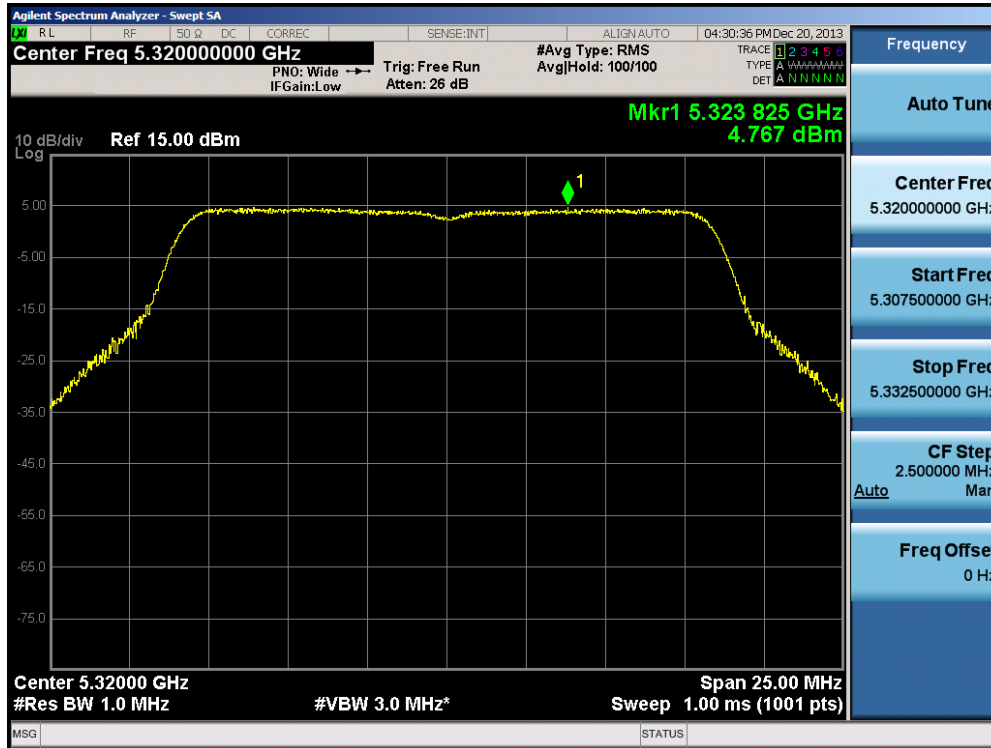
Plot 6-50. Peak Power Spectral Density Plot (802.11a (UNII Band 2A) – Ch. 64)
