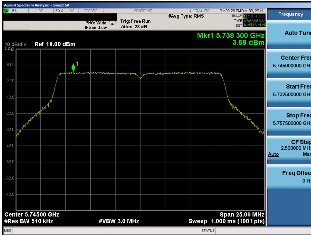
Plot 6-68. Peak Power Spectral Density Plot (802.11a (UNII Band 3) – Ch. 149)
