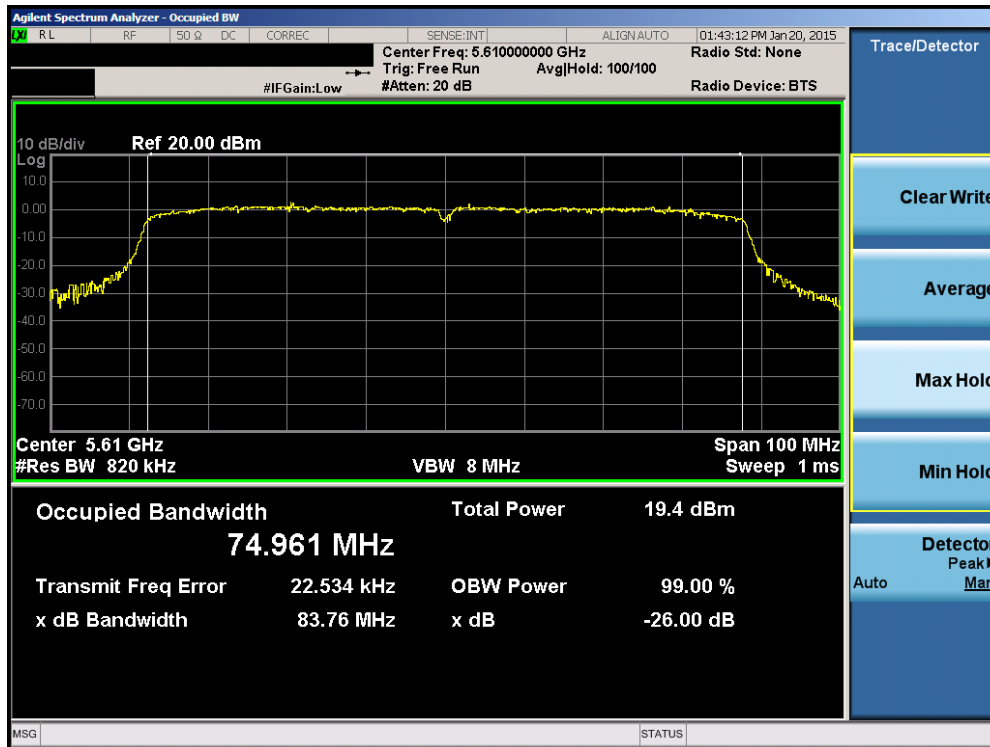
Plot 6-29. 26dB Bandwidth Plot (80MHz BW 802.11ac (UNII Band 2C) – Ch. 122
