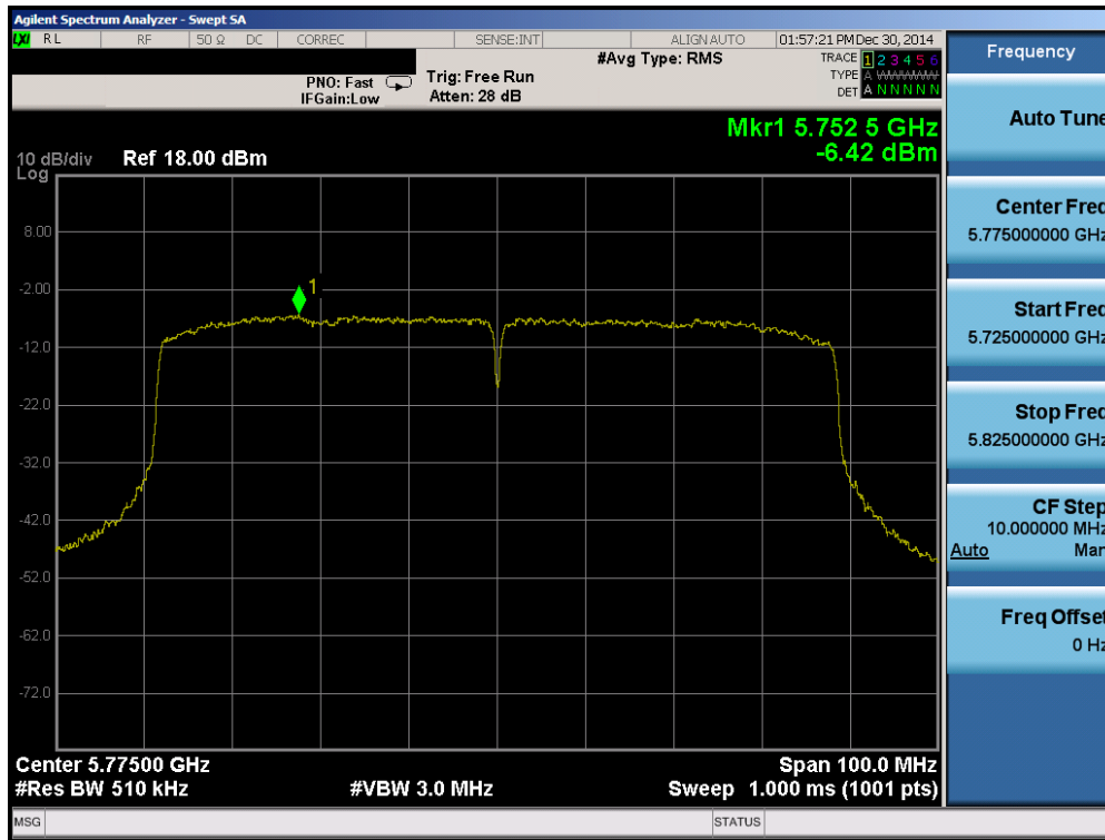
Plot 6-76. Peak Power Spectral Density Plot (80MHz BW 802.11ac (UNII Band 3) – Ch. 155)
