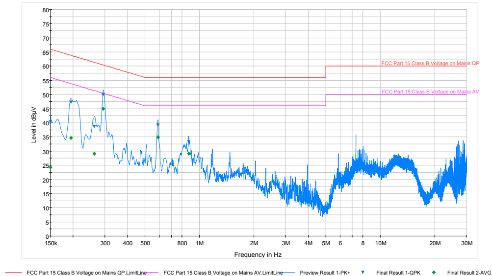
Plot 6-110. Line Conducted Plot with 802.11a UNII Band 1 (N)
