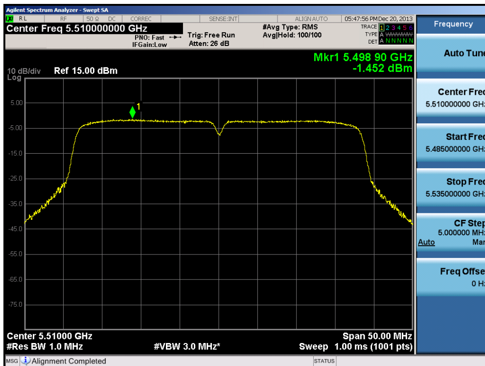
Plot 6-63. Peak Power Spectral Density Plot (40MHz BW 802.11n (UNII Band 2C) – Ch. 102)
