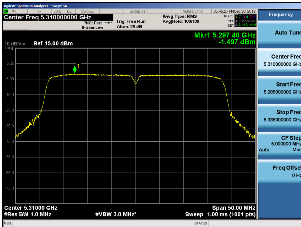
Plot 6-55. Peak Power Spectral Density Plot (40MHz BW 802.11n (UNII Band 2A) – Ch. 62)
