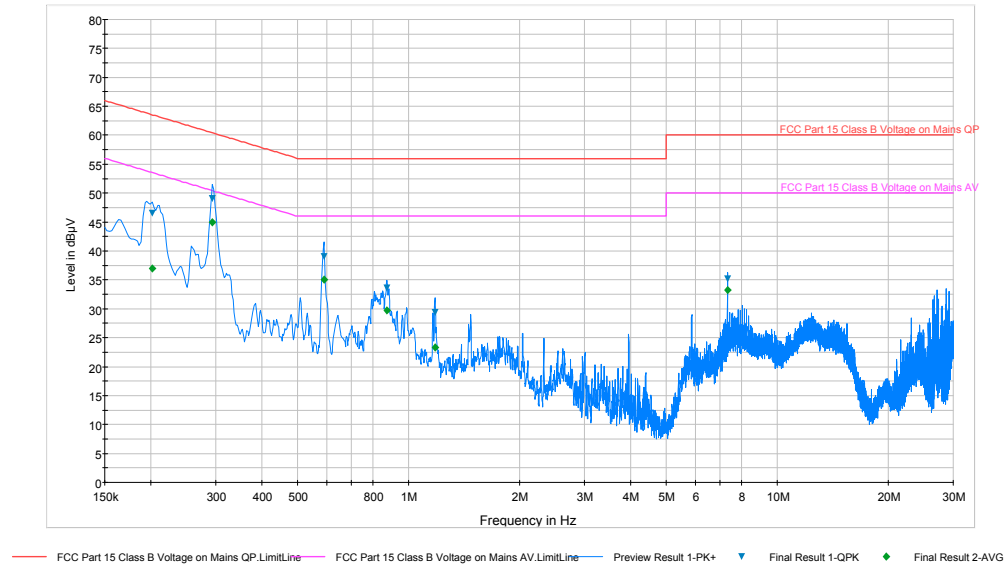
Plot 6-109. Line Conducted Plot with 802.11a UNII Band 1 (L1)
