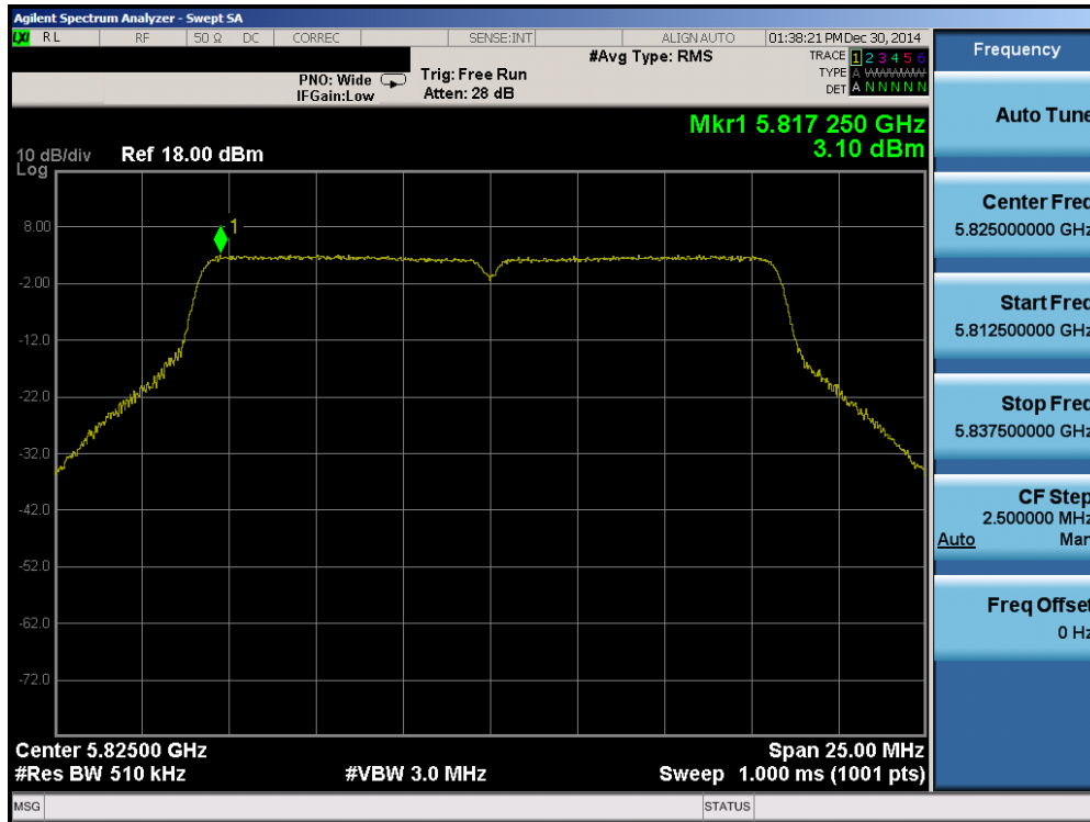
Plot 6-70. Peak Power Spectral Density Plot (802.11a (UNII Band 3) – Ch. 165)
