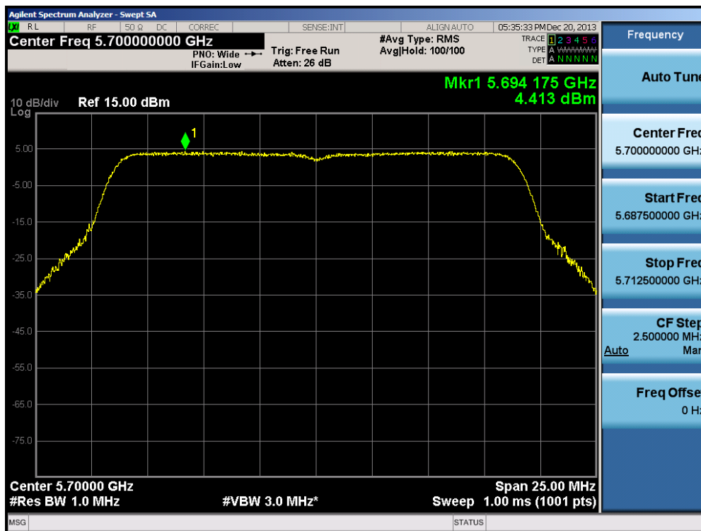
Plot 6-62. Peak Power Spectral Density Plot (20MHz BW 802.11n (UNII Band 2C) – Ch. 140)
