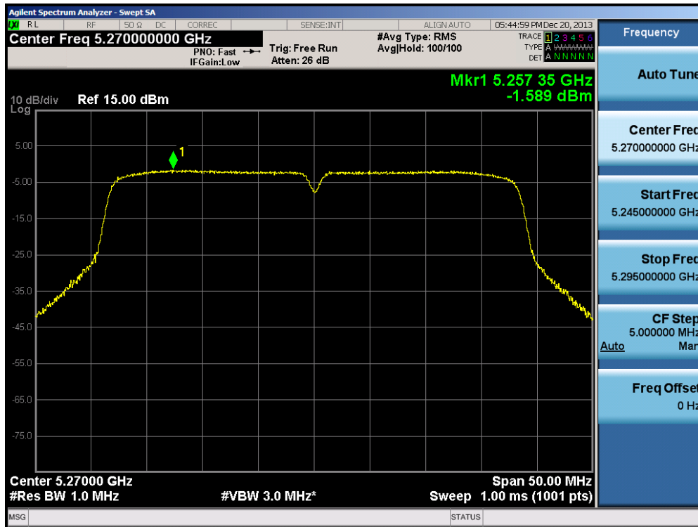
Plot 6-54. Peak Power Spectral Density Plot (40MHz BW 802.11n (UNII Band 2A) – Ch. 54)
