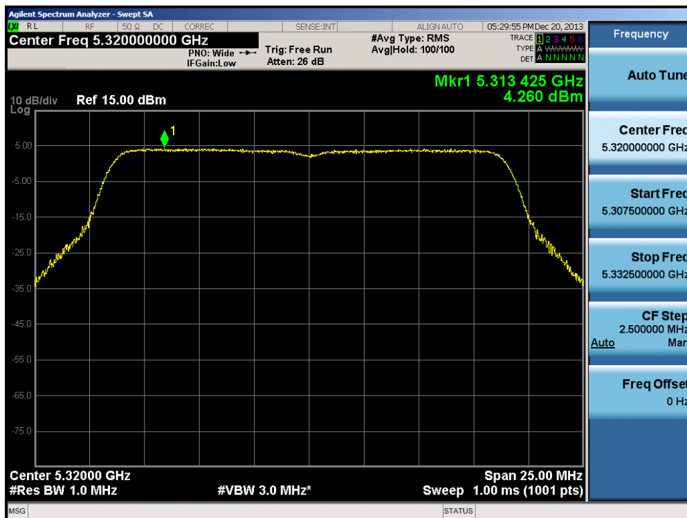
Plot 6-53. Peak Power Spectral Density Plot (20MHz BW 802.11n (UNII Band 2A) – Ch. 64)
