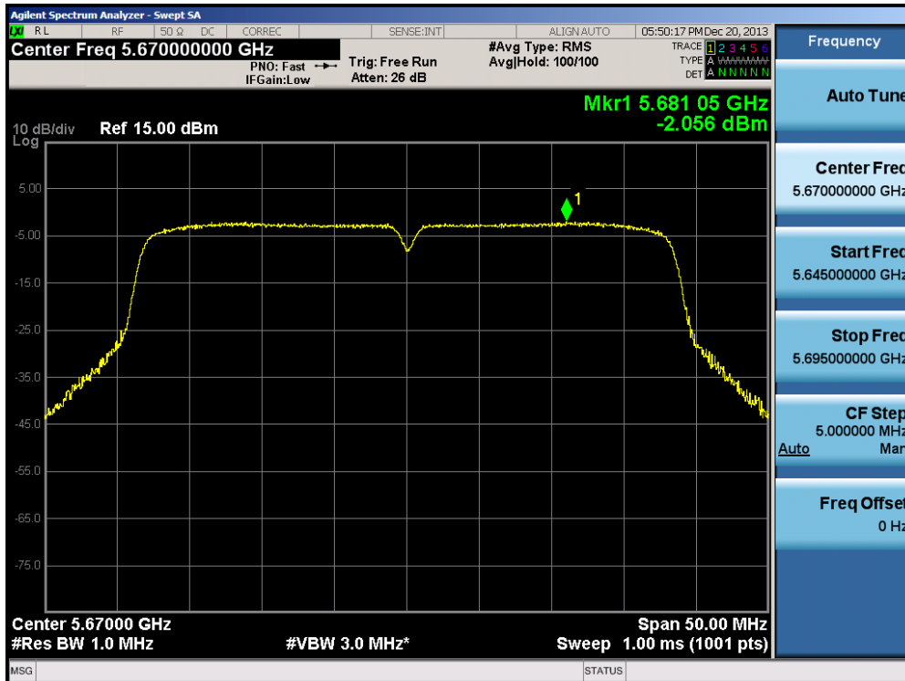
Plot 6-65. Peak Power Spectral Density Plot (40MHz BW 802.11n (UNII Band 2C) – Ch. 134)
