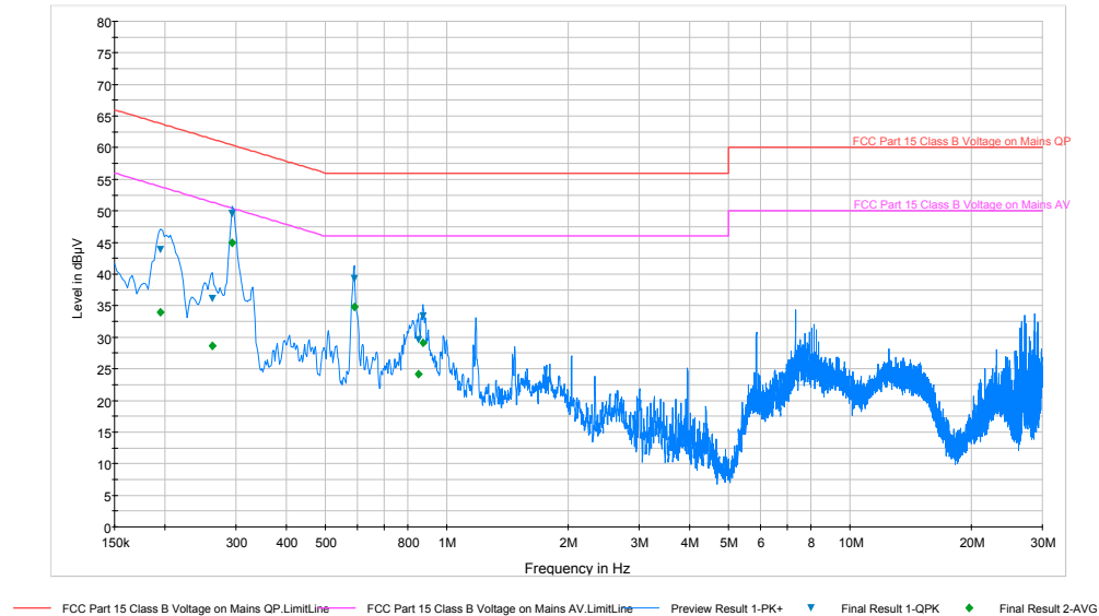
Plot 6-112. Line Conducted Plot with 802.11a UNII Band 2A (N)
