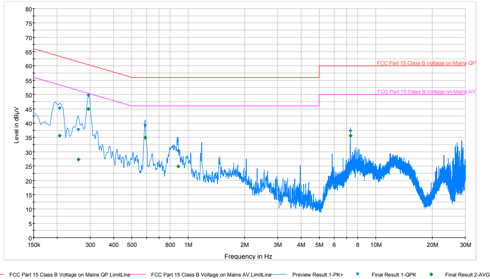
Plot 6-116. Line Conducted Plot with 802.11a UNII Band 3 (N)
