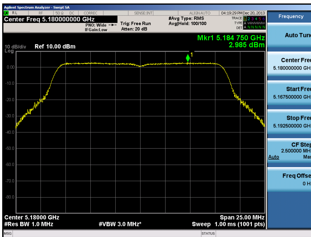
Plot 6-39. Peak Power Spectral Density Plot (802.11a (UNII Band 1) – Ch. 36)
