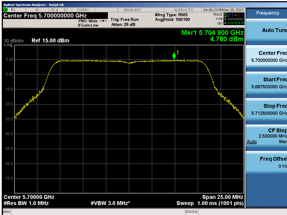
Plot 6-59. Peak Power Spectral Density Plot (802.11a (UNII Band 2C) – Ch. 140)
