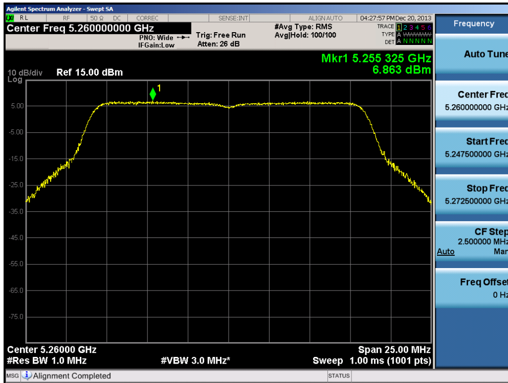
Plot 6-48. Peak Power Spectral Density Plot (802.11a (UNII Band 2A) – Ch. 52)
