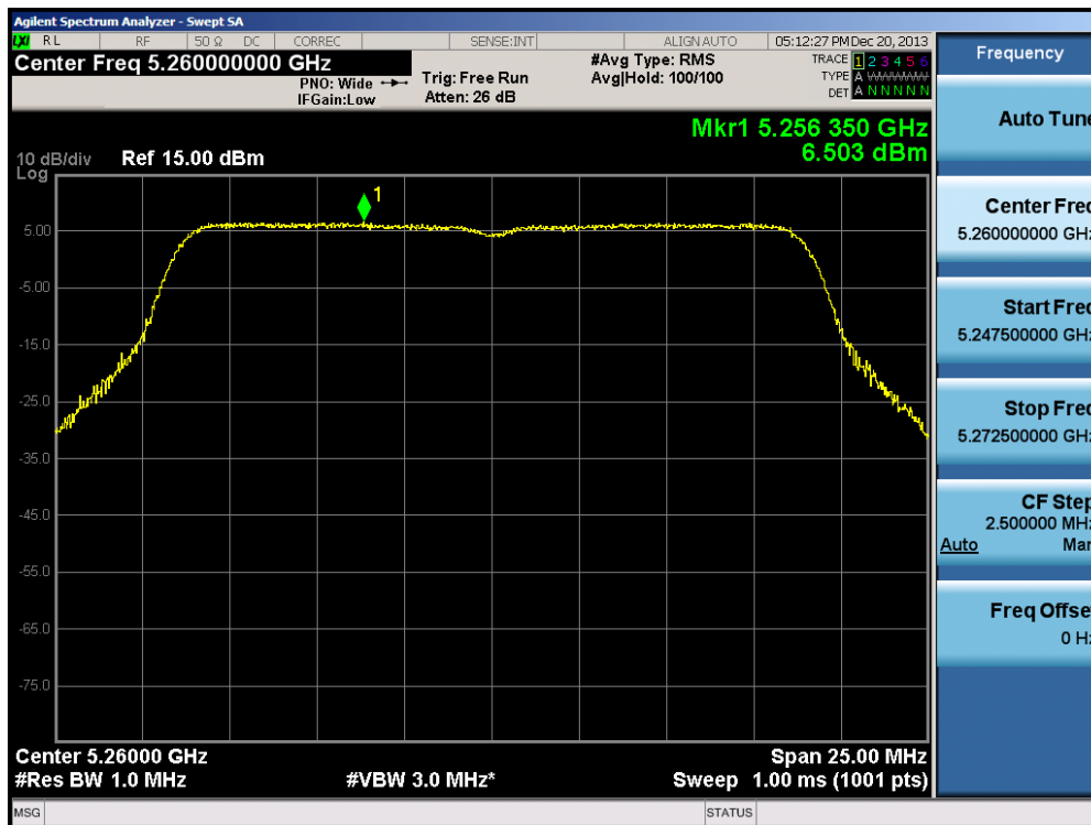
Plot 6-51. Peak Power Spectral Density Plot (20MHz BW 802.11n (UNII Band 2A) – Ch. 52)
