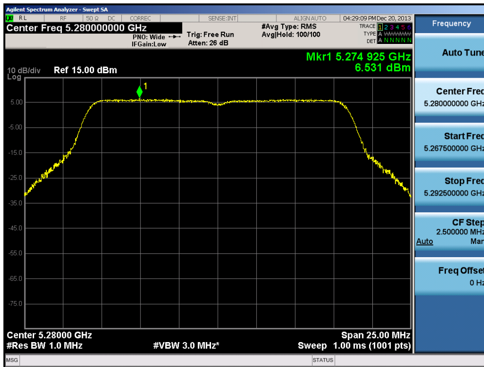
Plot 6-49. Peak Power Spectral Density Plot (802.11a (UNII Band 2A) – Ch. 56)
