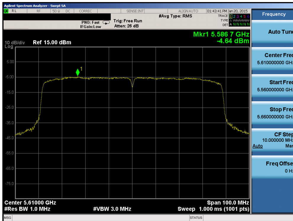
Plot 6-67. Peak Power Spectral Density Plot (80MHz BW 802.11ac (UNII Band 2C) – Ch. 122)
