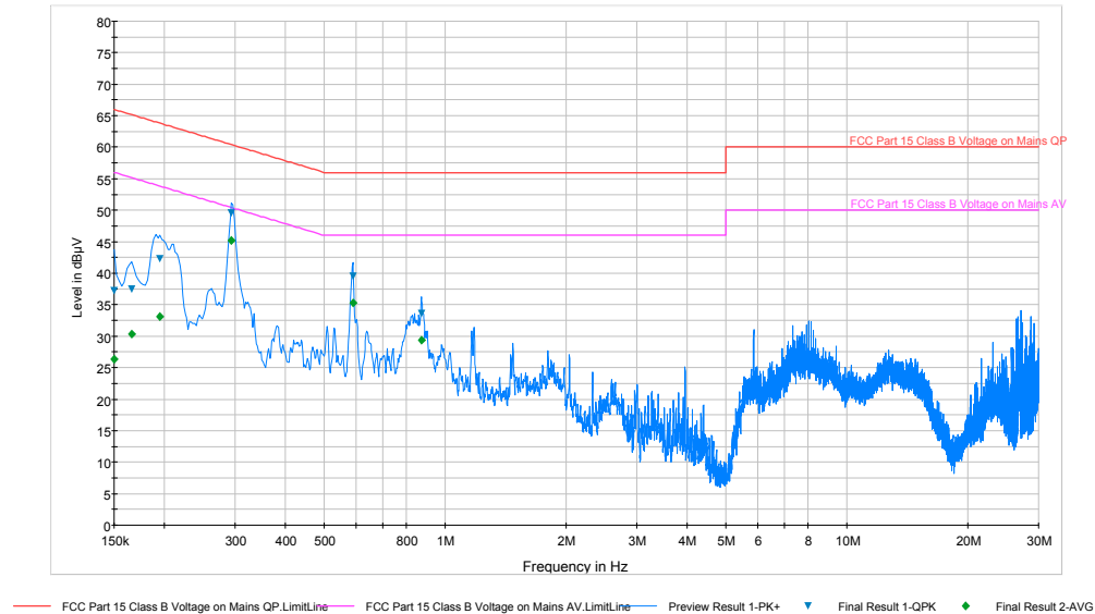
Plot 6-114. Line Conducted Plot with 802.11a UNII Band 2C (N)
