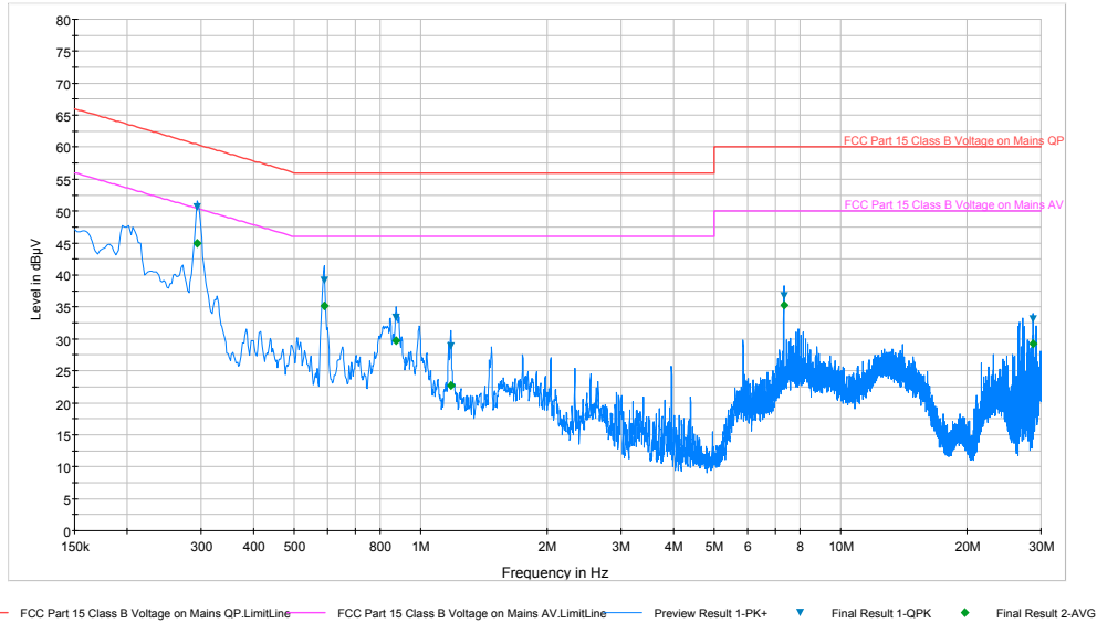
Plot 6-115. Line Conducted Plot with 802.11a UNII Band 3 (L1)
