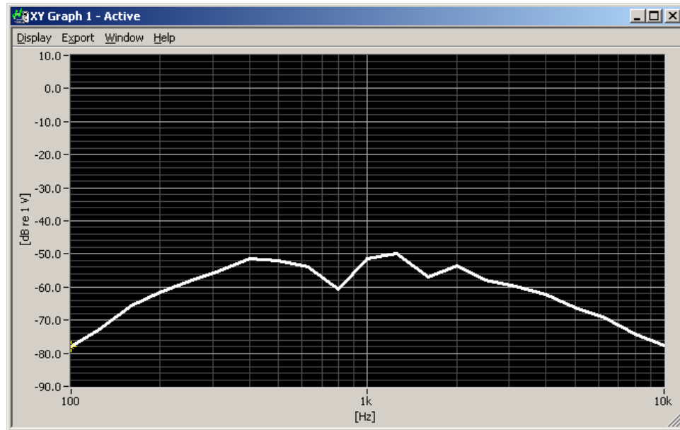
Figure 6-2 Worst-case ABM2 Plot for CDMA
