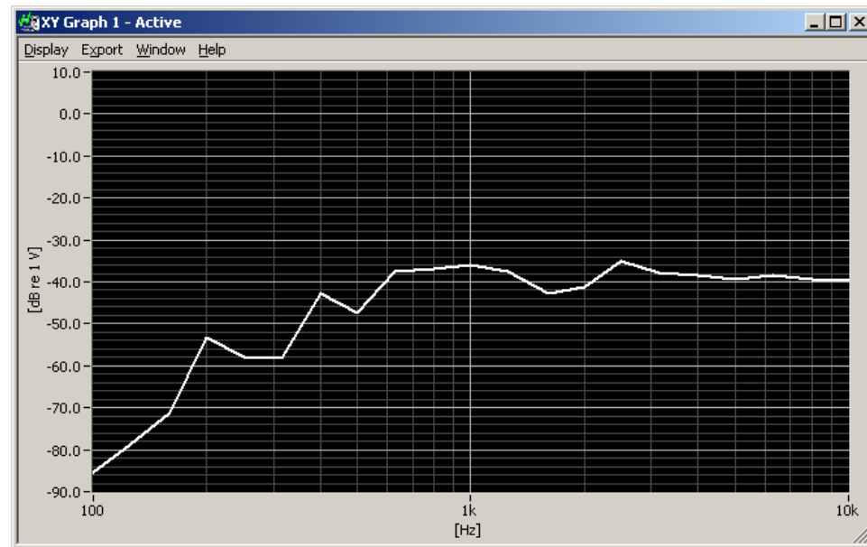
Figure 6-3 Worst-case ABM2 Plot for GSM
