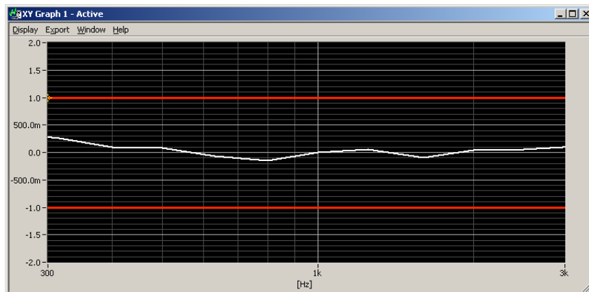
Figure 6-5 Helmholtz Coil Validation for Frequency Response
