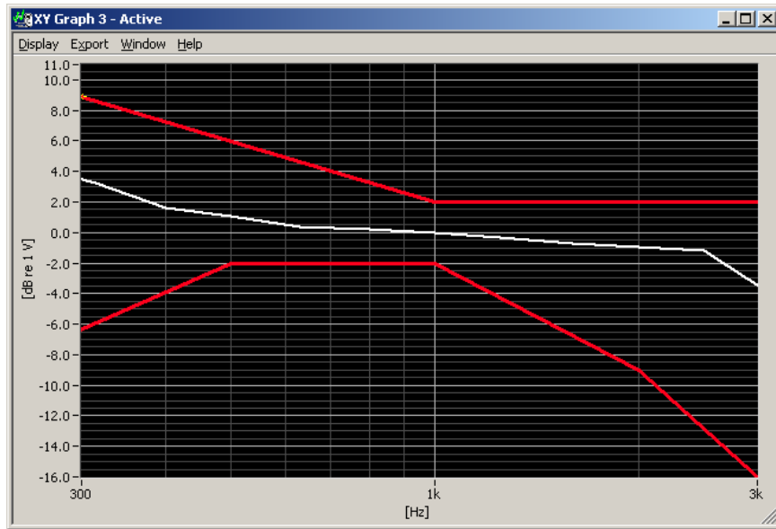
Figure 6-1 Axial Frequency Response
