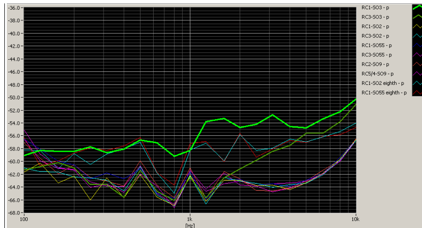
Figure 5-1 CDMA Audio Band Magnetic Noise
