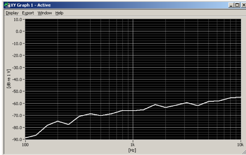
Figure 6-4 Worst-case ABM2 Plot for UMTS
