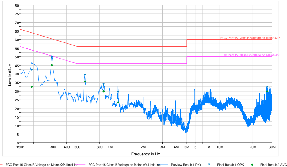
Plot 6-99. Line Conducted Plot with 802.11a UNII Band 2C (L1)
