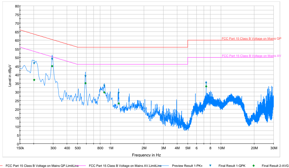
Plot 6-95. Line Conducted Plot with 802.11a UNII Band 1 (L1)
