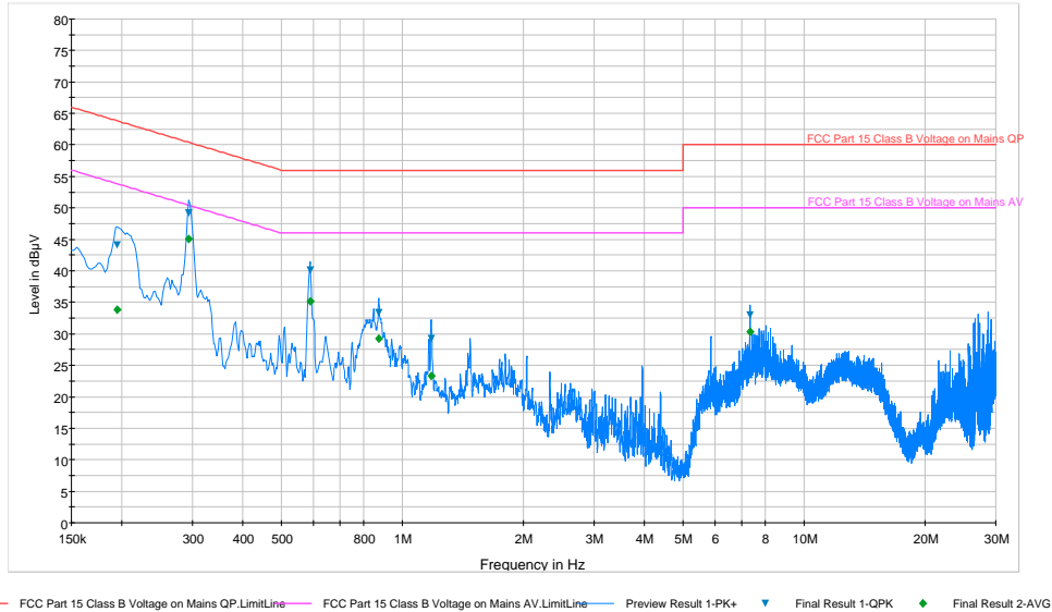
Plot 6-97. Line Conducted Plot with 802.11a UNII Band 2A (L1)
