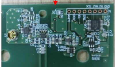
Zoom of main circuit
