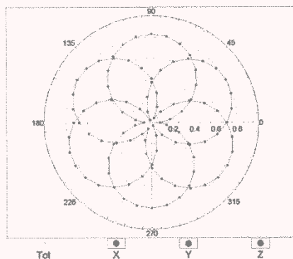
f=600 MHz,TEM
