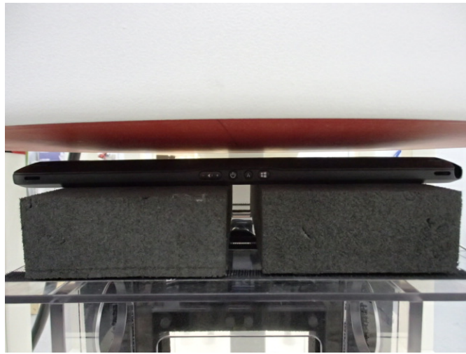
Bottom side, 16 mm Separation Distance
