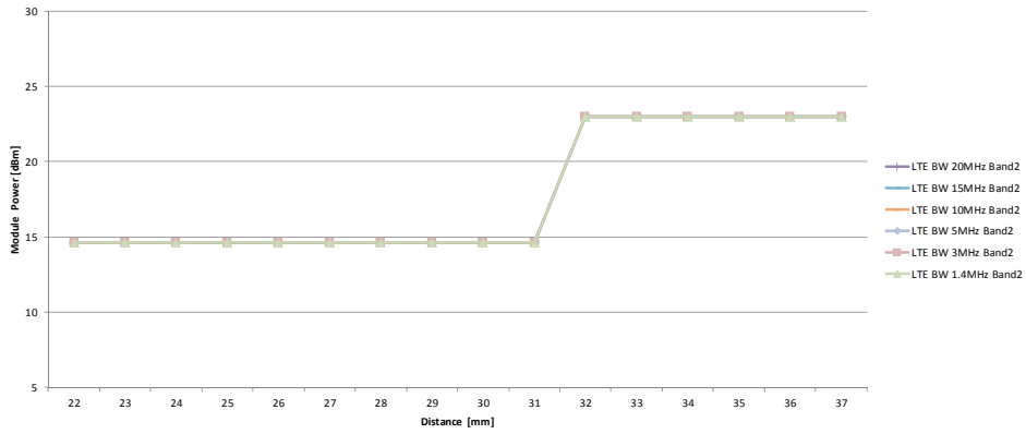
Power Reduction Graph For LTE Band 2
