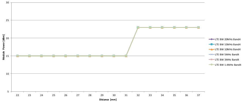
Power Reduction Graph For LTE Band 4
