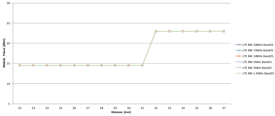
Power Reduction Graph For LTE Band 25
