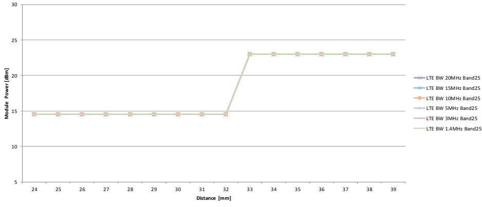
Power Reduction Graph For LTE Band 25
