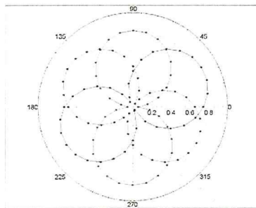
f=600 MHz,TEM
