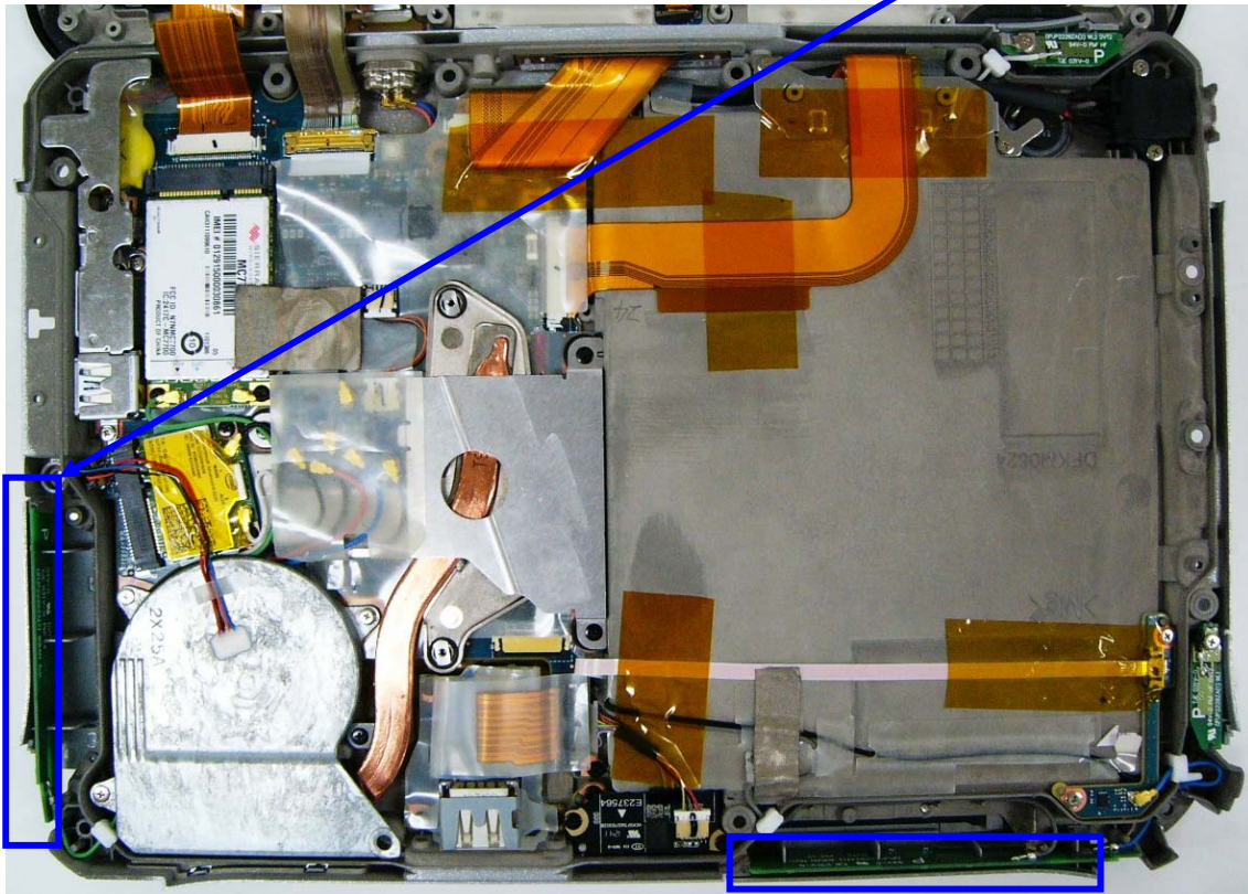
WWAN Main Antenna (Tx / Rx)
