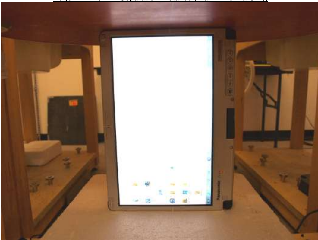
Edge 2 with 0 mm Separation Distance (Main Antenna Only)
