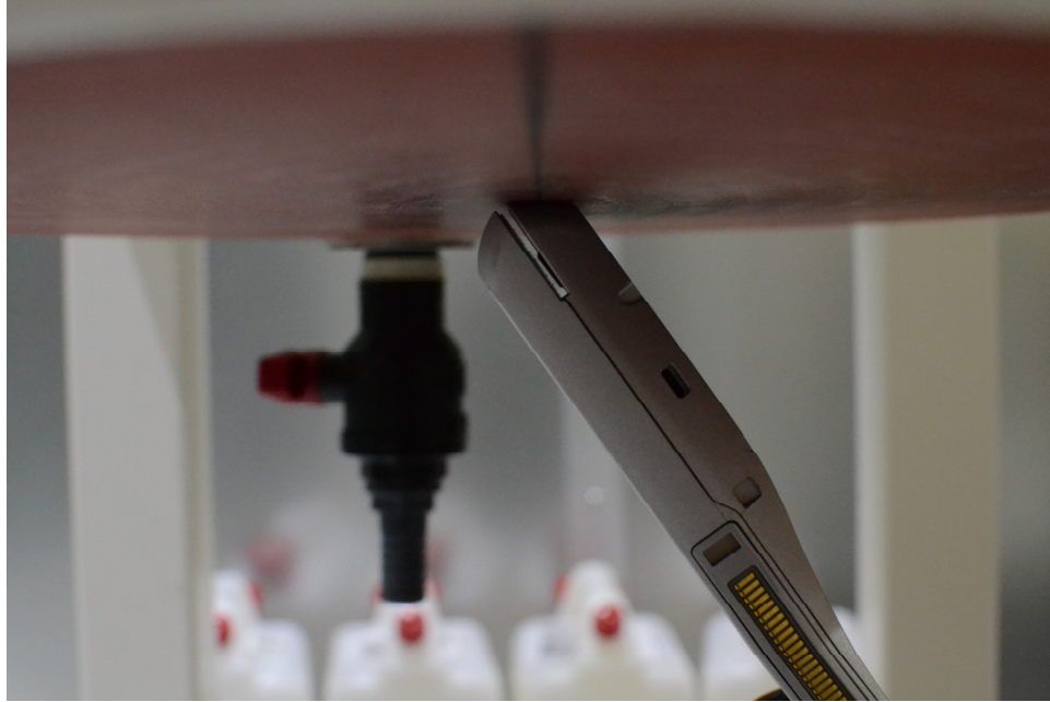
SAR Test Setup Photo 3: Top Edge Tilt (Top-Back Surface) at 0.0 cm
