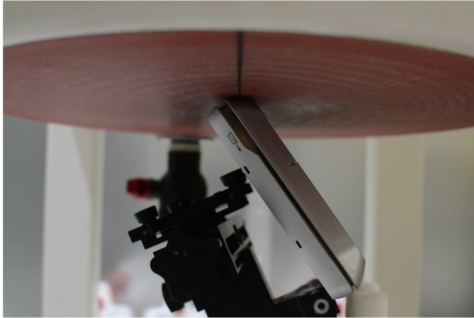
SAR Test Setup Photo 7: Left Edge Tilt (Left-Back Surface) at 0.0 cm
