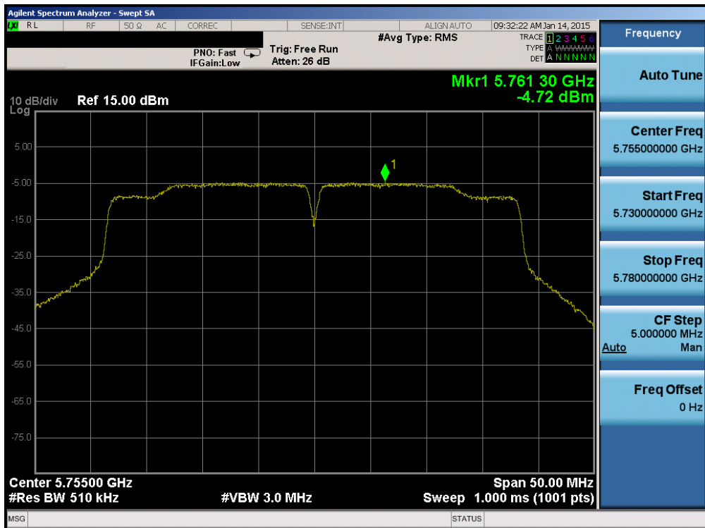
Plot 6-50. Power Spectral Density Plot (40MHz BW 802.11n (UNII Band 3) – Ch. 151)
