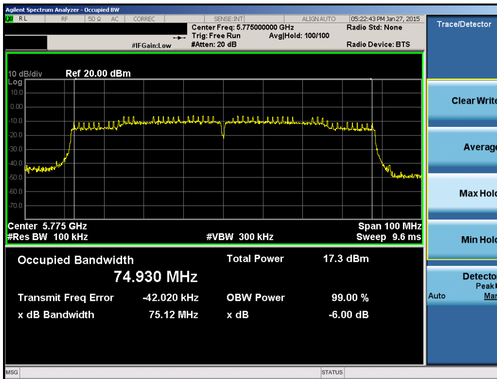
Plot 6-17. 6dB Bandwidth Plot (80MHz BW 802.11ac (UNII Band 3) – Ch. 155)
