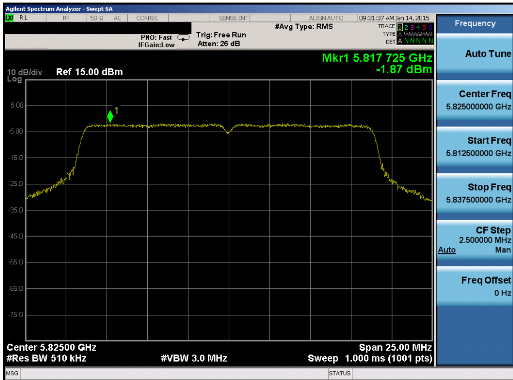
Plot 6-49. Power Spectral Density Plot (20MHz BW 802.11n (UNII Band 3) – Ch. 165)
