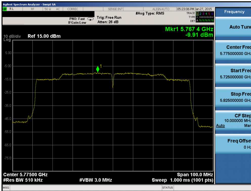
Plot 6-43. Power Spectral Density Plot (80MHz BW 802.11ac (UNII Band 3) – Ch. 155)
