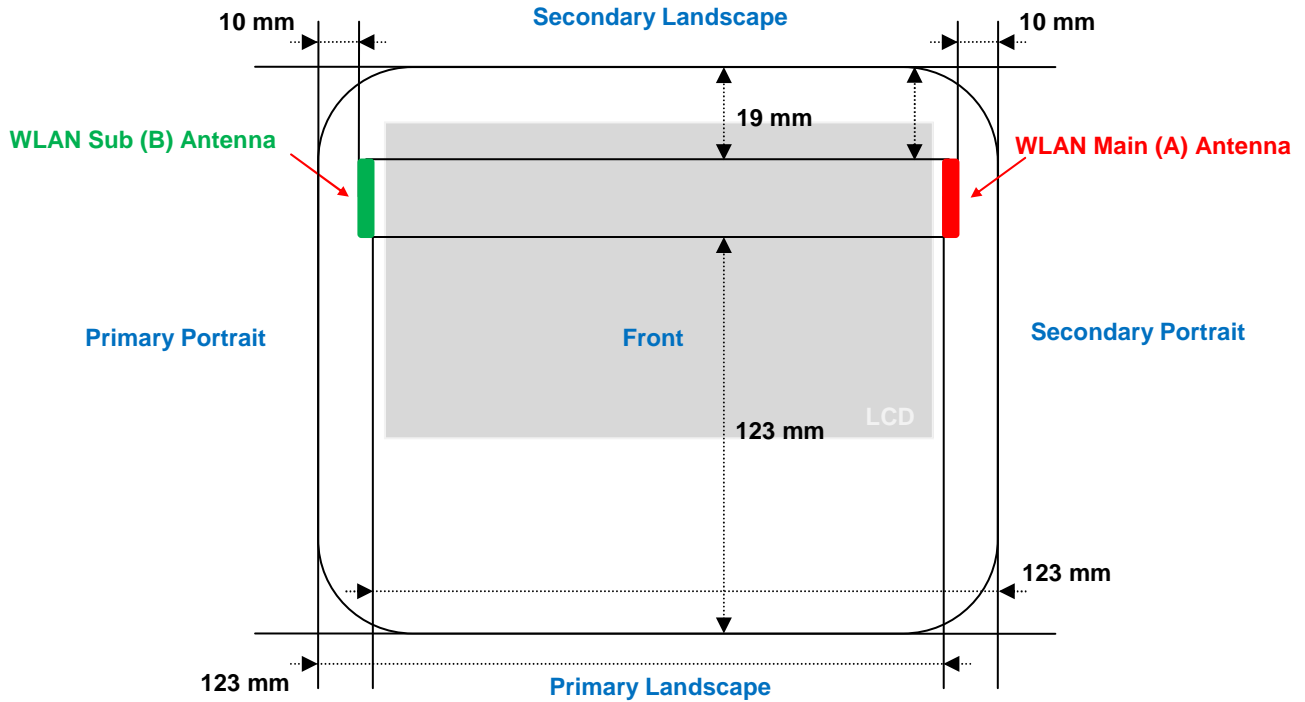
Front View
