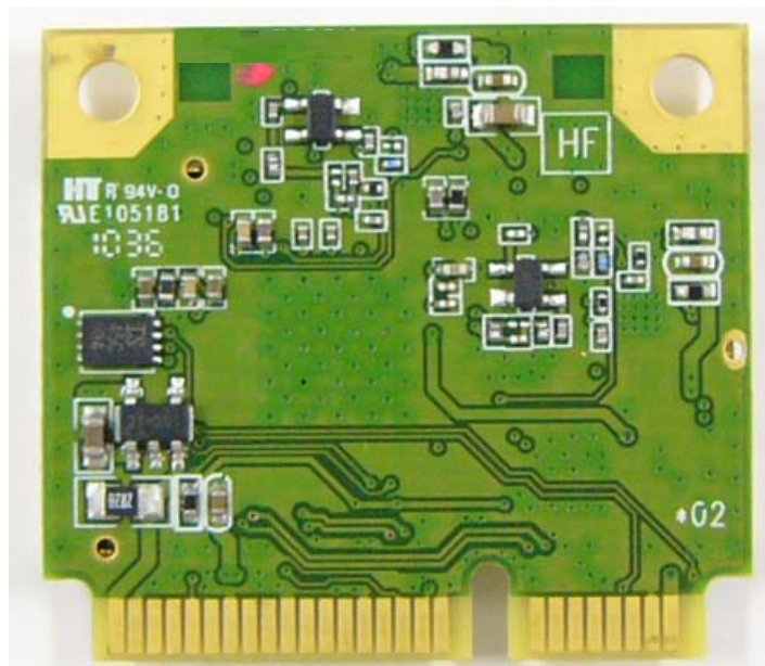
WLAN Exterior Bottom View
