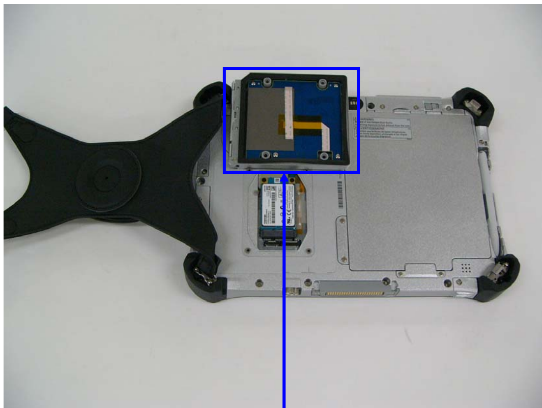
This is a HF-RFID module and antenna.
