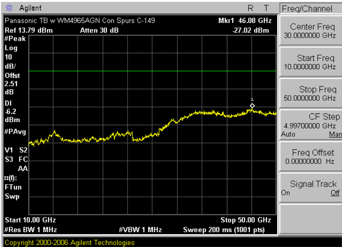
Plot 6-24. Conducted Spurious Plot (802.11a – Ch. 149)
