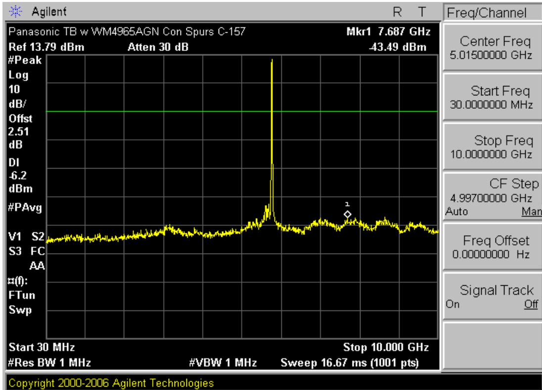
Plot 6-25. Conducted Spurious Plot (802.11a – Ch. 157)
