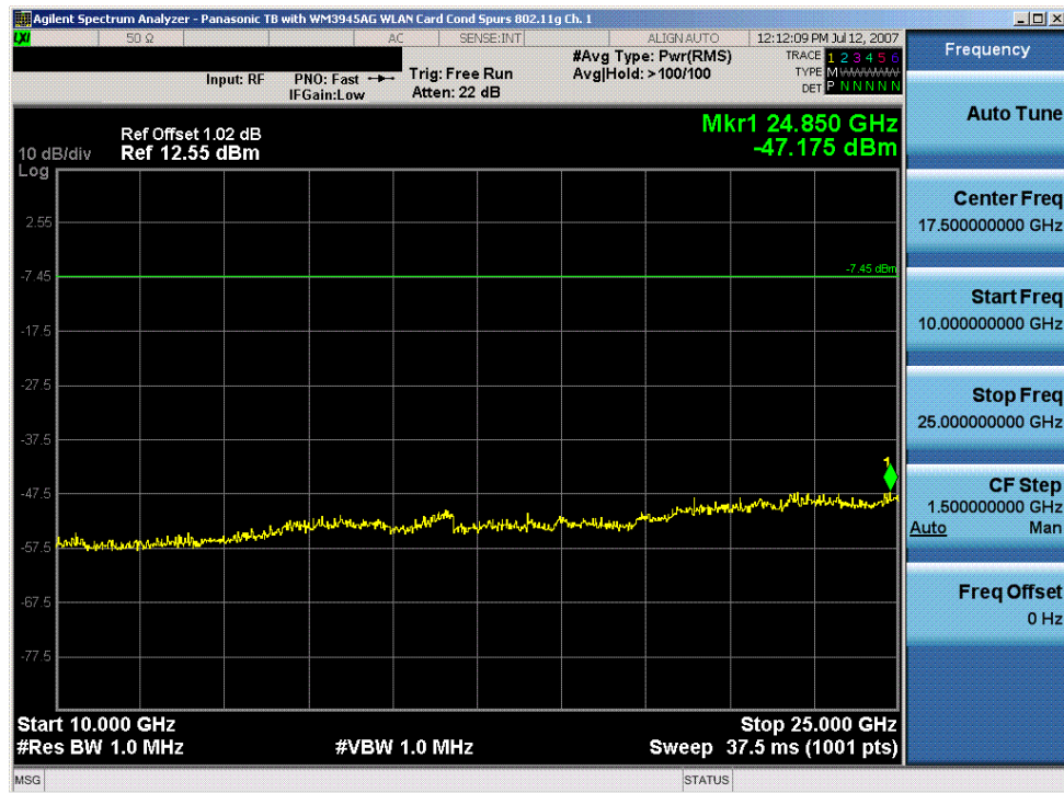
Plot 6-18. Conducted Spurious Plot (802.11g – Ch. 1)
