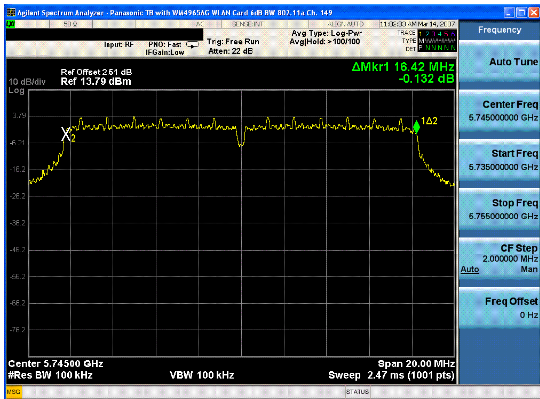
Plot 6-4. 6dB Bandwidth Plot (802.11a – Ch. 149)
