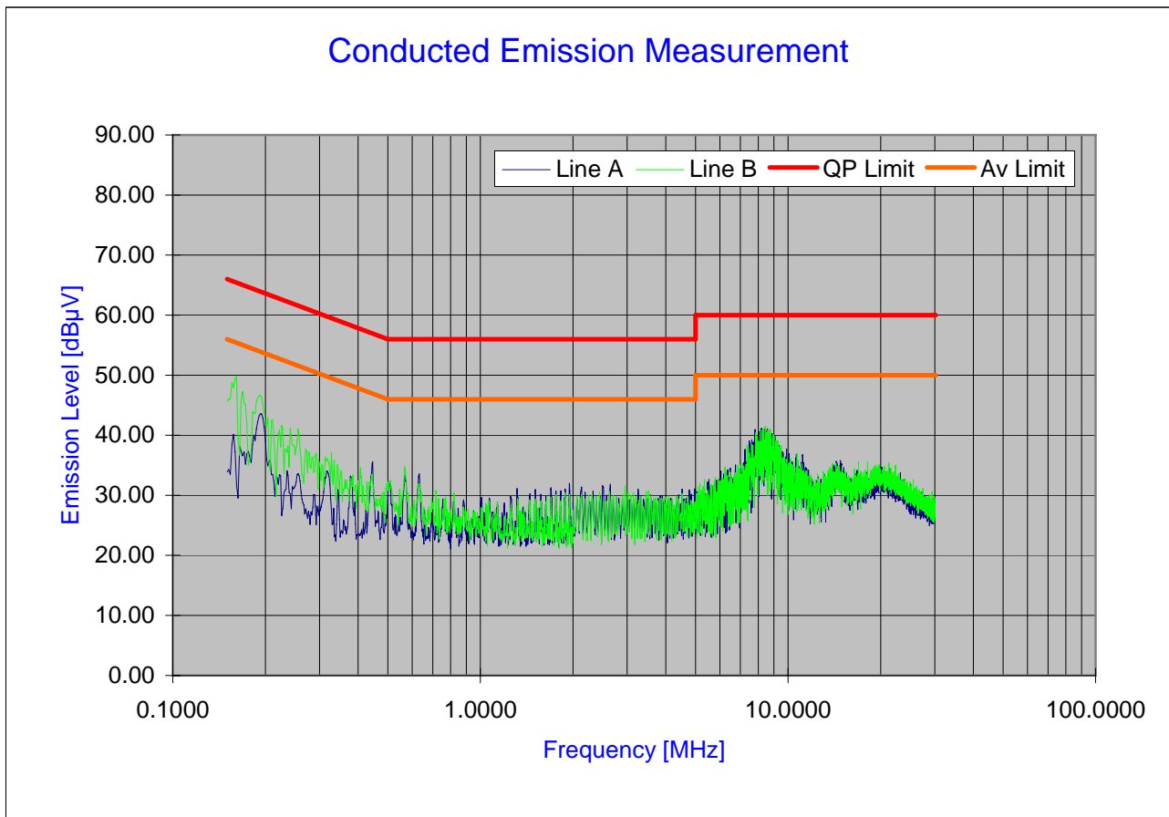
Plot 6-30. Line Conducted Plot with 802.11a
