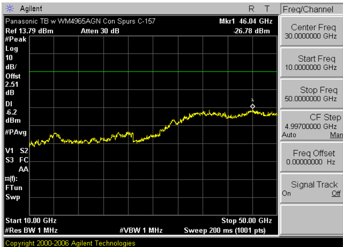
Plot 6-26. Conducted Spurious Plot (802.11a – Ch. 157)
