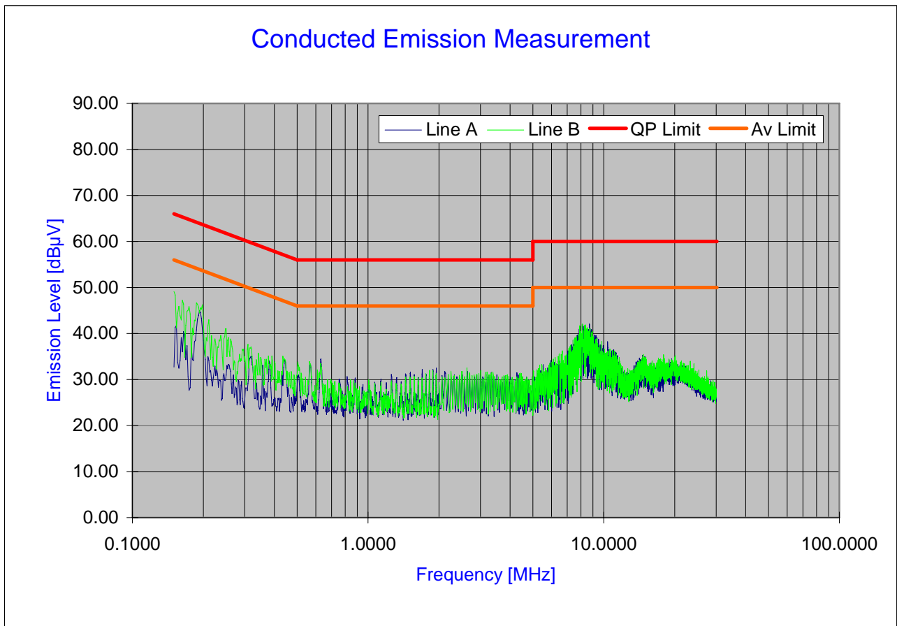
Plot 6-29. Line Conducted Plot with 802.11g
