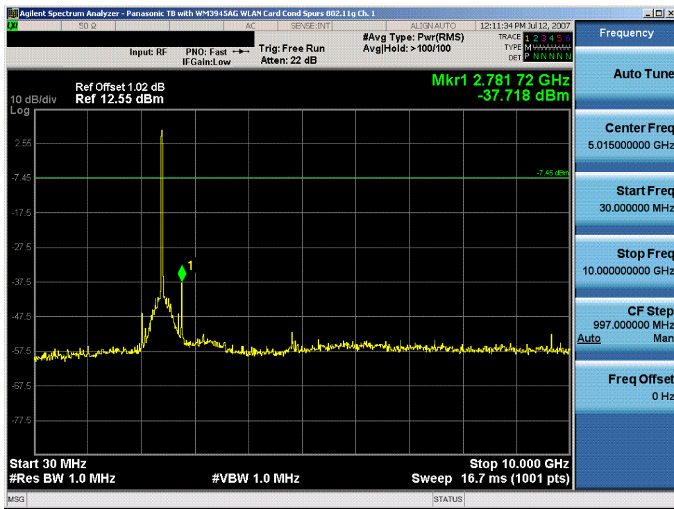
Plot 6-17. Conducted Spurious Plot (802.11g – Ch. 1)
