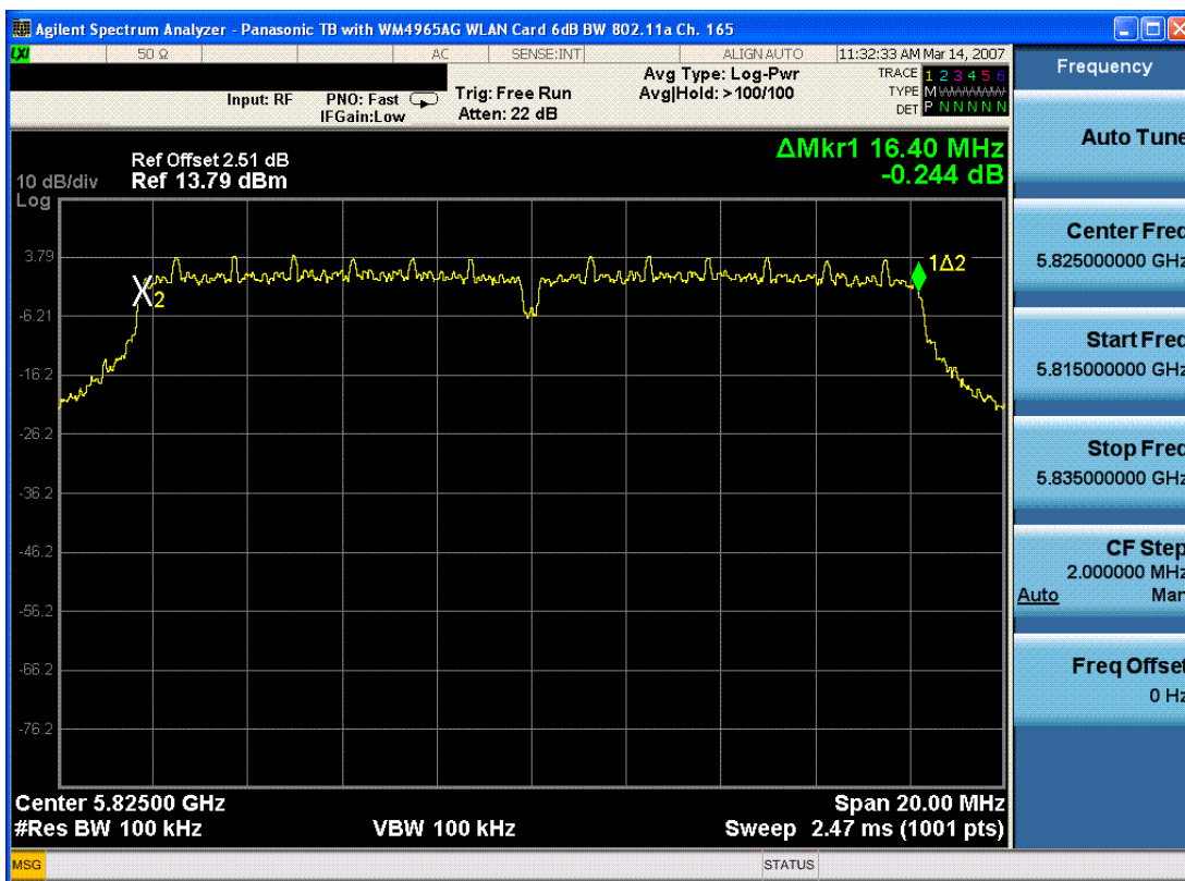
Plot 6-6. 6dB Bandwidth Plot (802.11a – Ch. 165)
