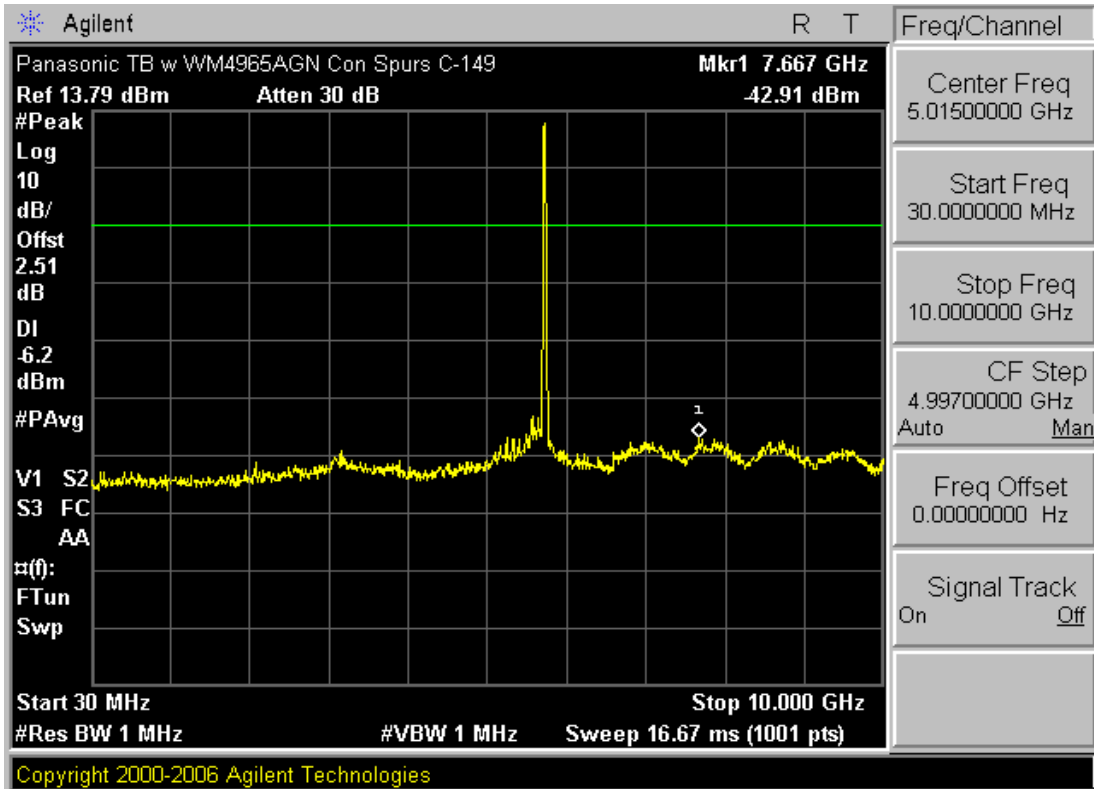
Plot 6-23. Conducted Spurious Plot (802.11a – Ch. 149)
