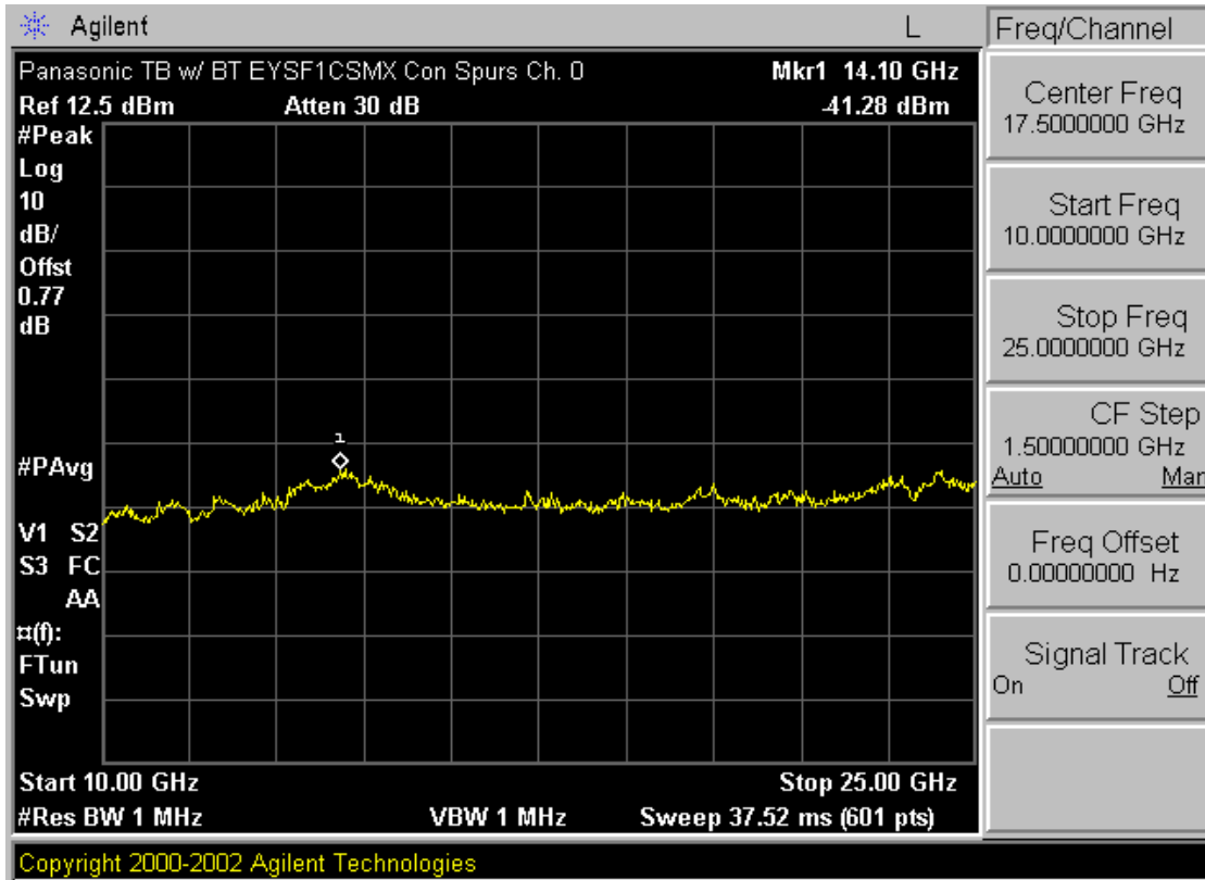
Plot 6-12. Conducted Spurious Plot (Bluetooth – Ch. 0)
