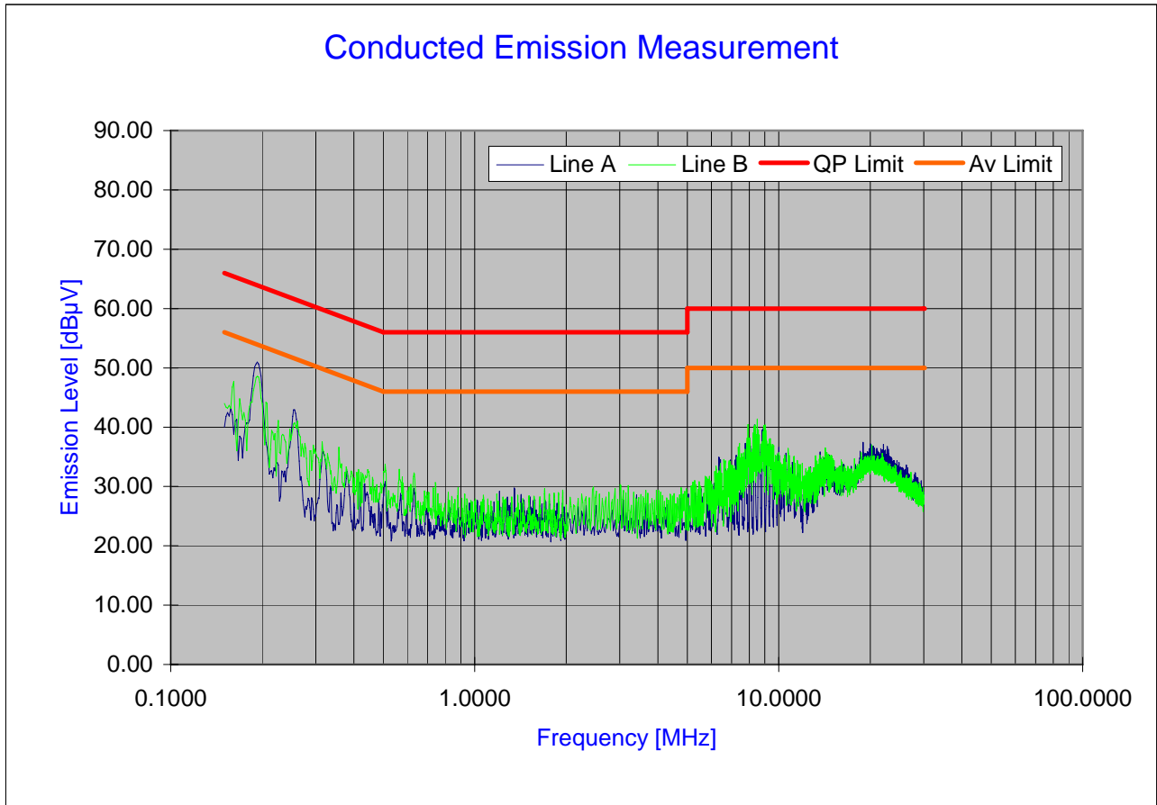
Plot 6-19. Line Conducted Plot with Bluetooth
