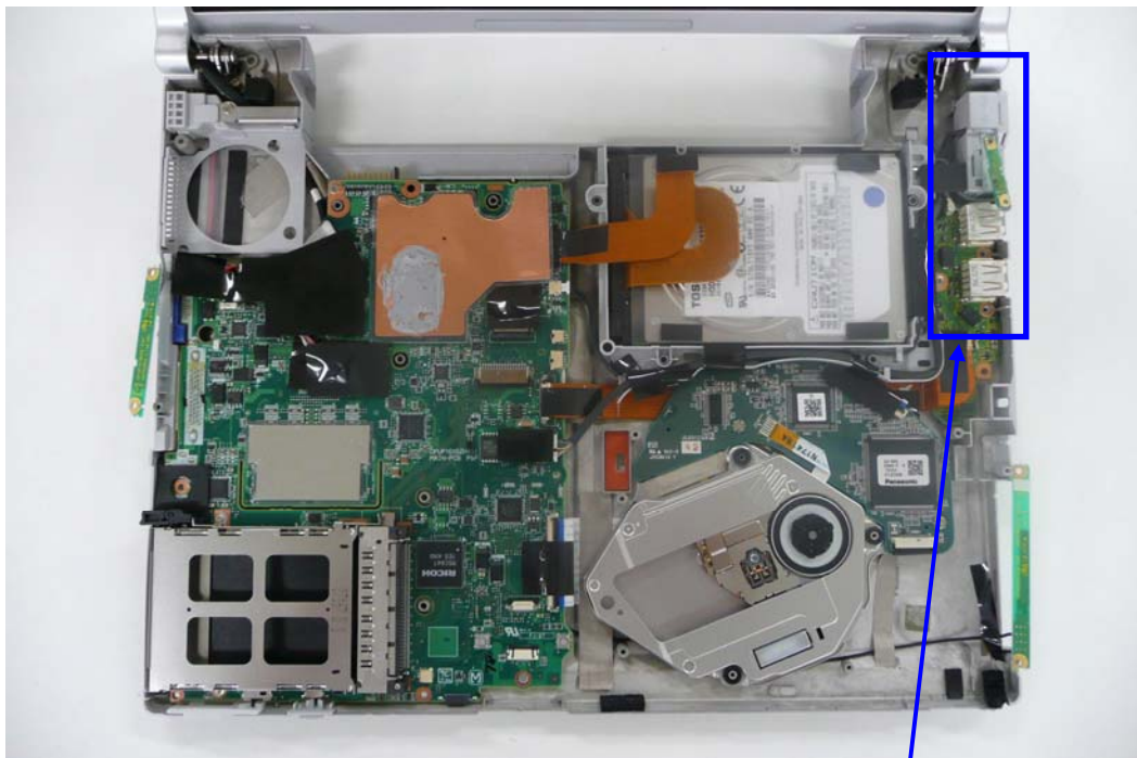
BlueTooth Module (Reverse side of PWB)
