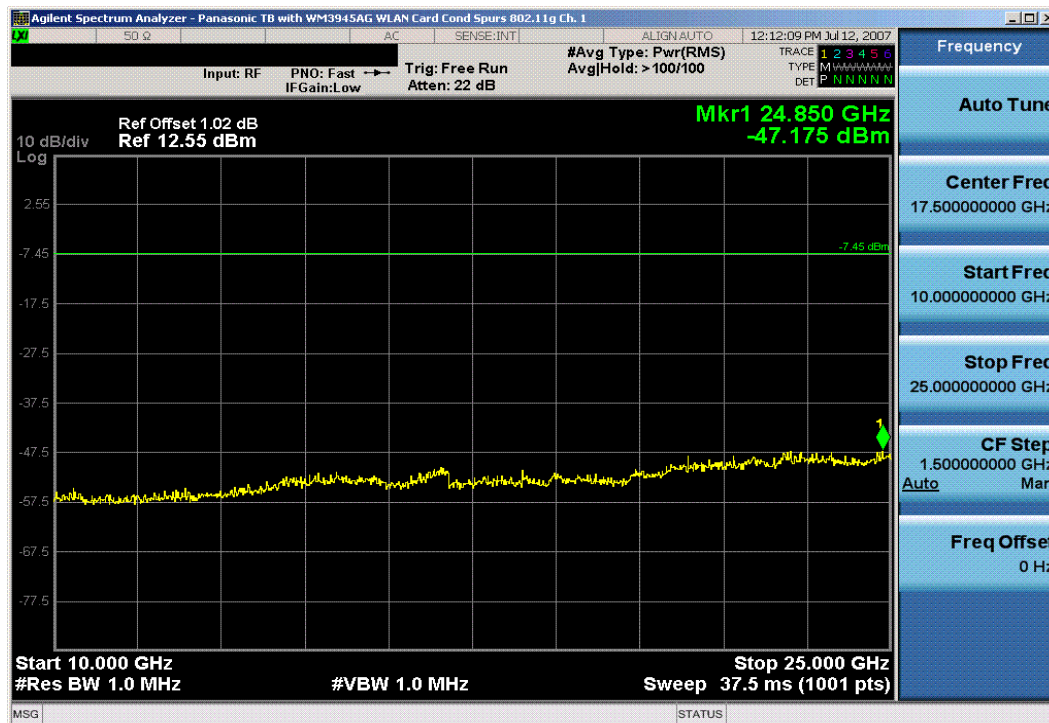
Plot 6-18. Conducted Spurious Plot (802.11g – Ch. 1)
