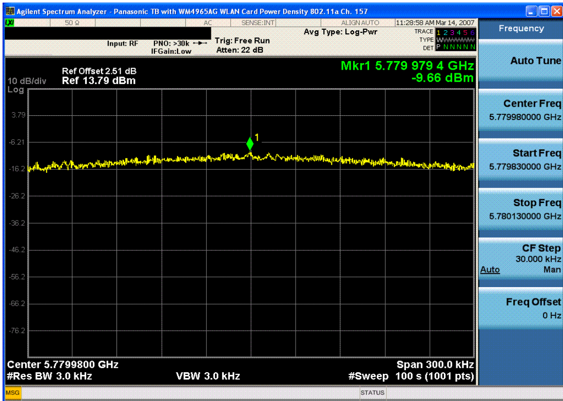
Plot 6-11. Power Spectral Density Plot (802.11a – Ch. 157)
