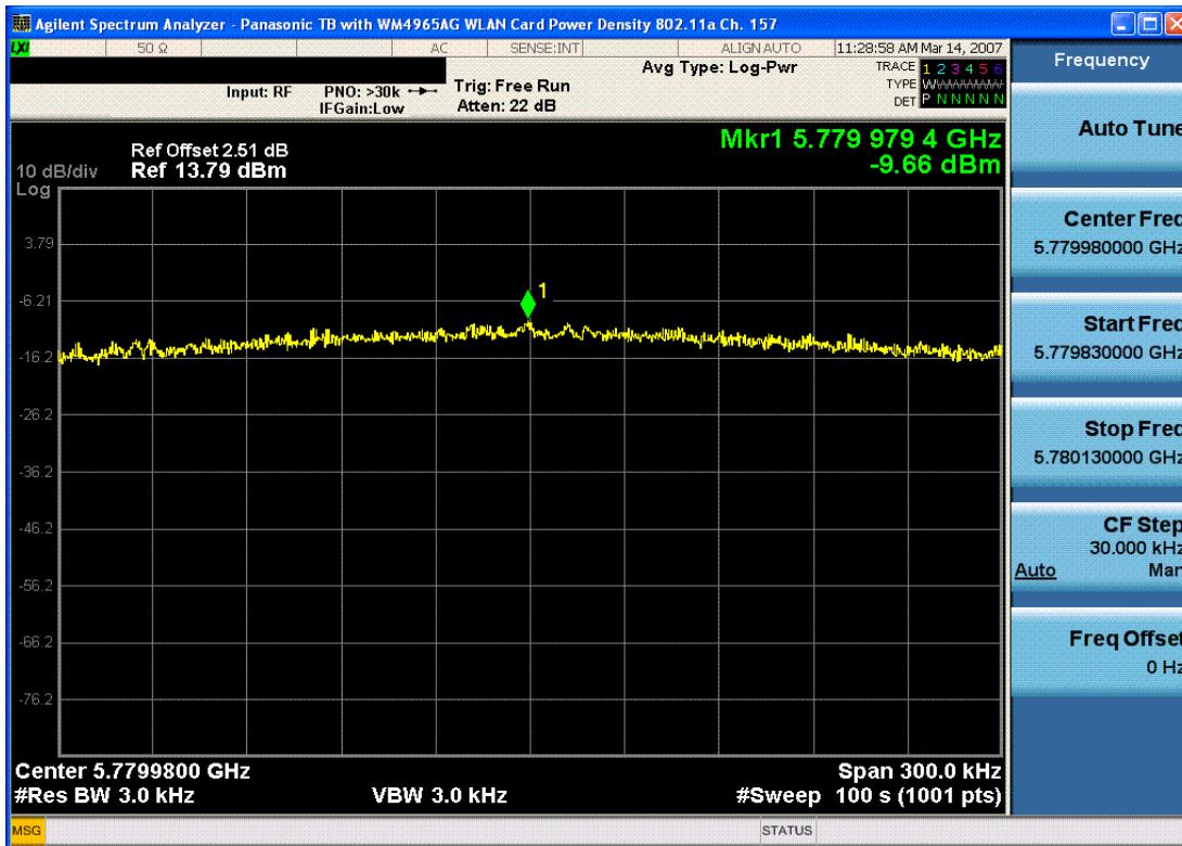
Plot 6-11. Power Spectral Density Plot (802.11a – Ch. 157)
